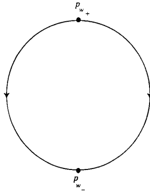
Figure 4.6: The one-dimensional connection from p_{w+} to p_{w-} on the invariant circle that is the intersection of Fix(SO(2)) with S_r^3 .
