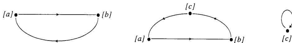
Figure 3.6: Quotient heteroclinic cycles of the quotient heteroclinic network \Sigma/\Gamma .
