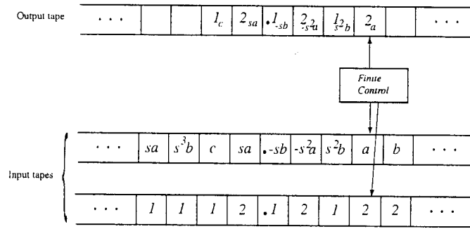
Figure 6.1: The Turing machine \mathcal{T} that takes a sequence in X_M , a sequence in X_2 and outputs a sequence in X_N .
