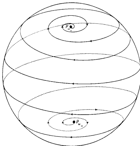
Figure 4.5: Invariant two-sphere \mathbf{D} on \mathbf{S}_r^3 that coincides with the two-dimensional heteroclinic connection from p_{w-} to p_{w+} , when \alpha > 0 . (If \alpha < 0 the arrows are reversed.)
