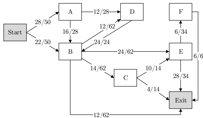
Figure 2.10: Example of a user navigational trails [Sin04].
