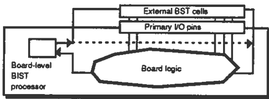
Fig. 1: Test of primary I/O pins under control of the on-board BIST processor.
