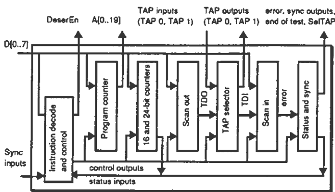
Fig. 7: Block diagram of the board-level BIST processor.
