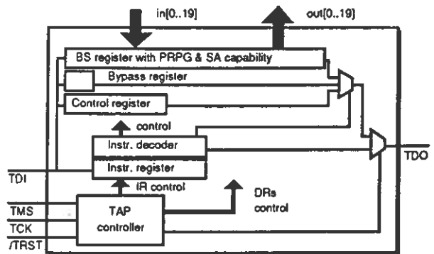
Fig. 4: Block diagram of the programmable-length LFSR PLD.
