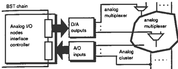
Fig. 5: The interface to analog I/O nodes.
