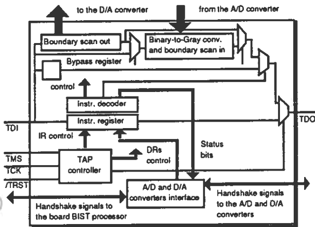
Fig. 6: Block diagram of the analog I/O nodes interface controller.
