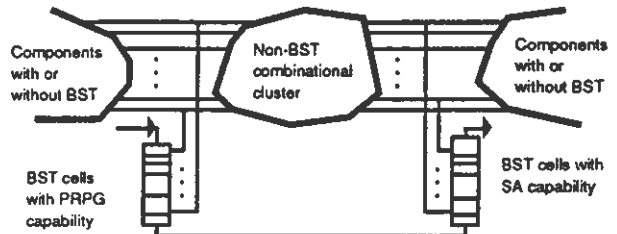
Fig. 3: Virtual cluster testing by PRPG and SA techniques.
