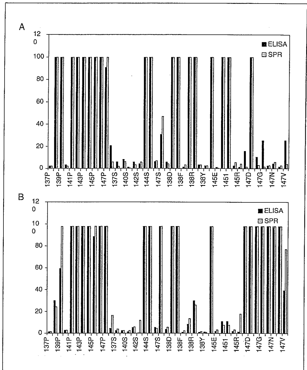
Figure 18.9.6 Comparison of antigenic ranking of FMDV peptides (series of 43 A15 single-point mutants) by SPR and ELISA: (A) Interaction of FMDV peptides with MAb SD6. (B) Interaction of FMDV peptides with MAb 4C4. On both panels, the vertical axis depicts relative IC 50 and K D values for ELISA and SPR data, respectively. Relative IC 50 is defined as the quotient IC 50 (mutant peptide)/IC 50 (A15 peptide). Similarly, relative K D = K D (mutant peptide)/K D (A15 peptide).
