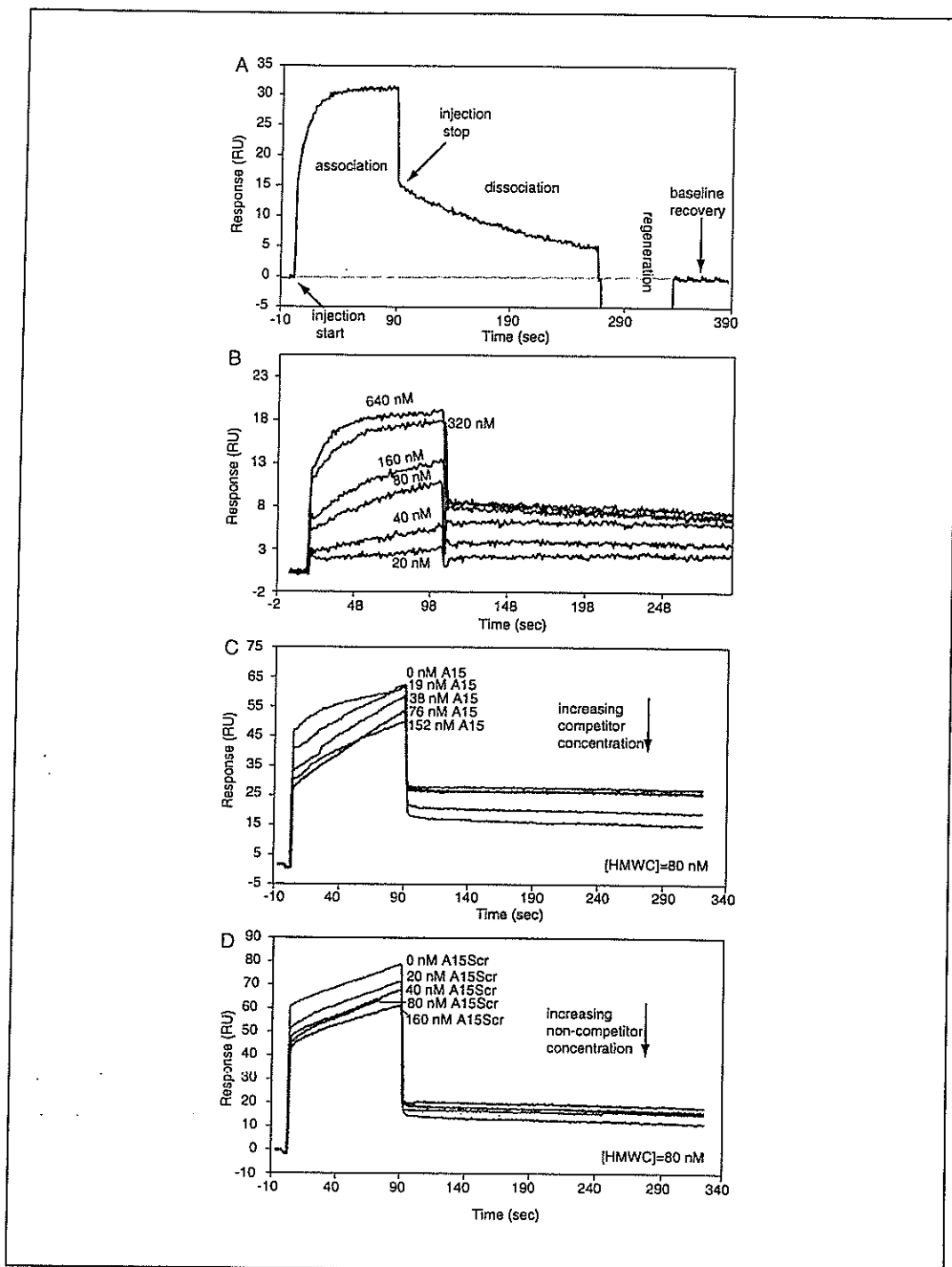
Figure 18.9.5 Experimental sensorgrams in different situations: (A) interaction of FMDV peptide A15 (600 nM in HBS) with immobilized MAb SD6 (see Table 18.9.1, footnotes a and b). (B) Full set of binding curves for the interaction between peptide A15(140P) (A15 with a Ser→Pro mutation at position 140; see Table 18.9.2, footnotes a and b) and immobilized MAb 4C4. (C) Surface competition assay between varying concentrations of native peptide A15 and a constant concentration of protein JX249A (an engineered \beta -galactosidase containing the immunodominant site of FMDV strain C-S8c1) on a 4C4 surface. The competition is shown by the fact that JX249A-antibody association and dissociation rates respectively decrease (decreasing positive slopes during first 90 sec) and increase (increasing negative slopes after 90 sec) with increasing concentrations of the target analyte (peptide A15). (D) Surface competition assay between varying concentrations of negative control peptide A15Scr (contains the same amino acid residues of A15, but randomized) and a constant concentration of antigenic protein JX249A on a 4C4 surface. In contrast to panel C, no decrease in slope during the association phase (or corresponding increase during the dissociation phase) is observed in this case.
