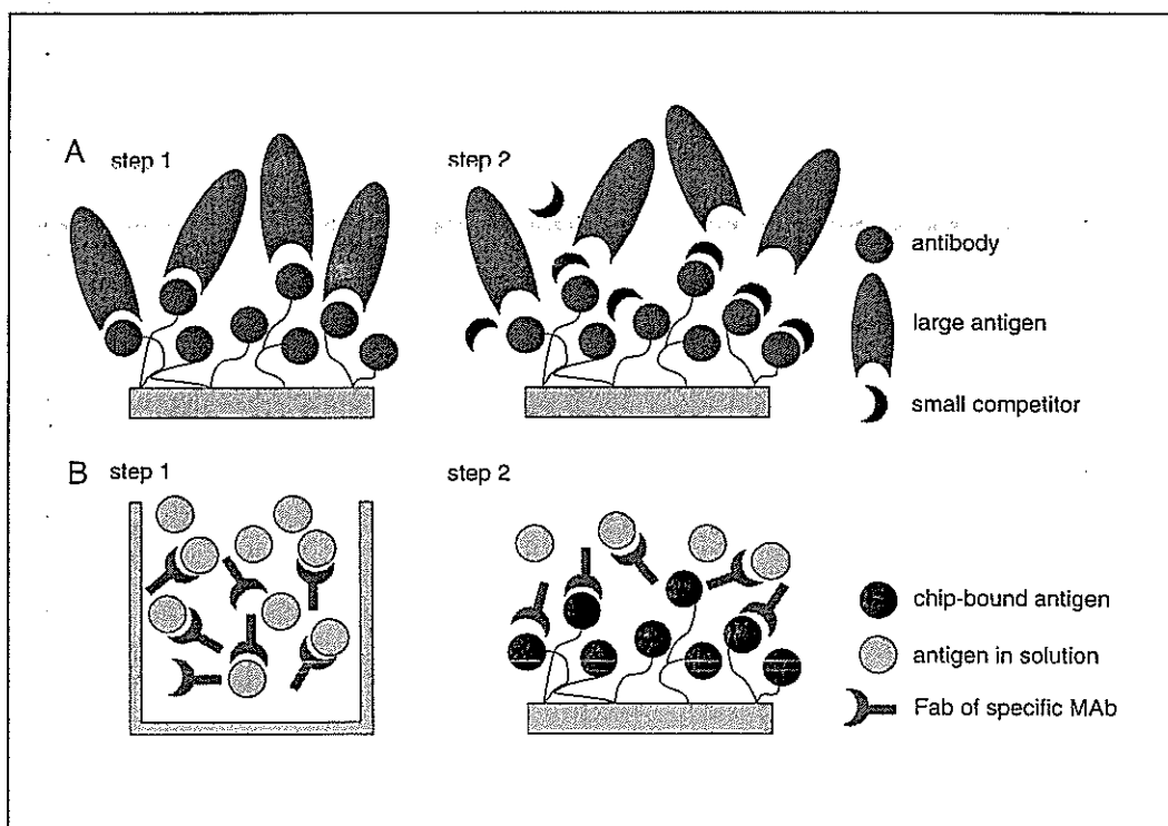
Figure 18.9.2 Indirect biospecific interaction analysis by SPR: (A) Surface competition assay. (B) Solution affinity assay.
