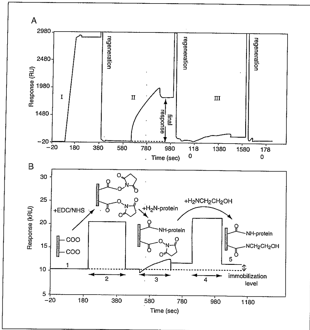
Figure 18.9.4 Stages involved in the covalent immobilization of MAb on the chip: (A) Three sequential pre-concentration assays: I, 50 \mu\text{g/ml} MAb in 10 mM acetate buffer, pH 5.5; II, 5 \mu\text{g/ml} MAb in 10 mM acetate buffer, pH 5.5; III, 5 \mu\text{g/ml} MAb in 10 mM formate buffer, pH 4.5. (B) Steps in covalent MAb immobilization via amine coupling: 1, free carboxymethyl dextran layer; 2, activation of carboxyl groups with an EDC/NHS mixture; 3, injection of MAB solution; 4, unreacted groups blocked by ethanolamine injection; 5, final MAB surface.
