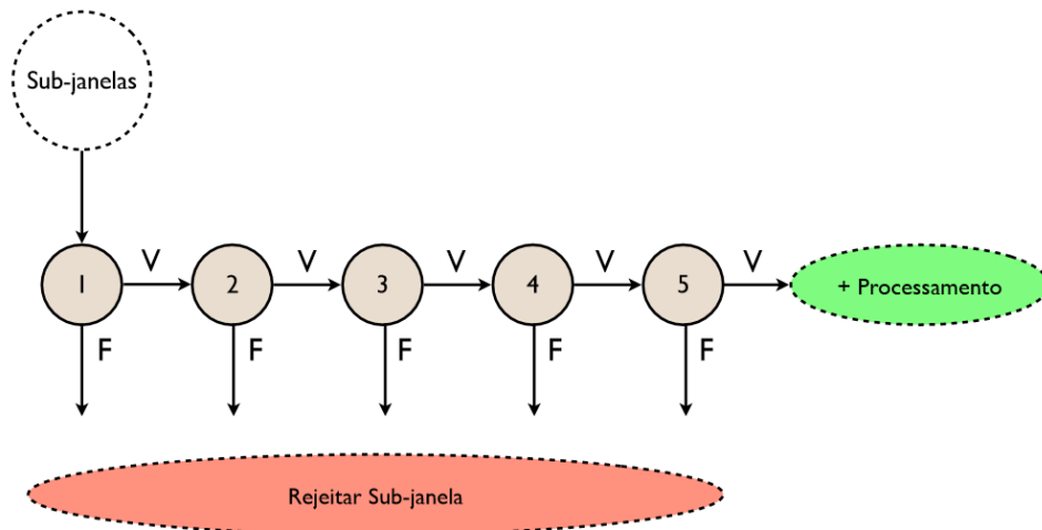
Figura 3.12: Cascade of Classifiers
