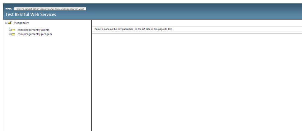
Figura 4.26: Interface Inicial
