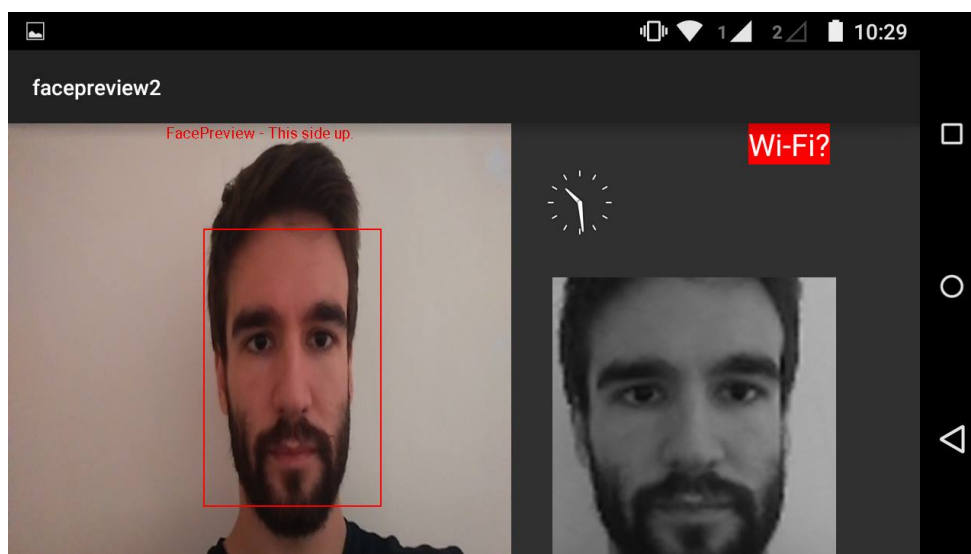
Figura 3.13: Interface RBLCF
