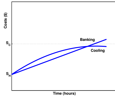
Figure 2.2: Start up cost function in plants with steam turbines.
