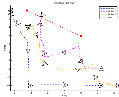
Figure 6.4: The Solution Simulation: Formation Behavior with the TS-TFA approach
