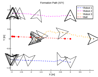
Figure 4.21: Simulation 4: Homogeneous Keeping Formation - Plot XY
