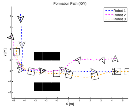
Figure 5.8: Simulation 1: Heterogeneous Formation - Plot XY
