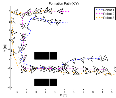
Figure 5.6: Simulation 1: Homogeneous Formation - Plot XY
