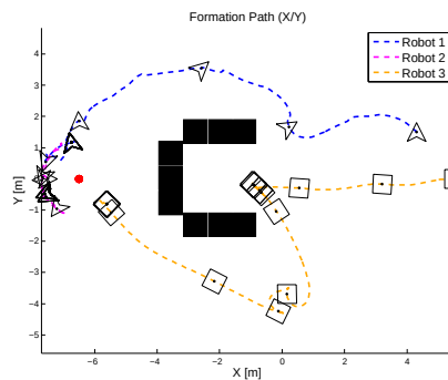
Figure 5.12: Simulation 2: Heterogeneous Formation - Plot XY
