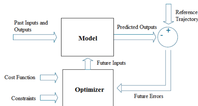
Figure 2.6: Generic MPC Structure.
