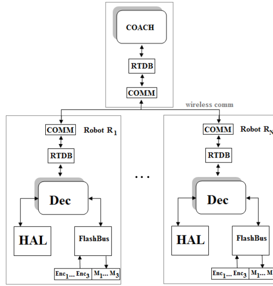
Figure 3.4: The General Architecture
