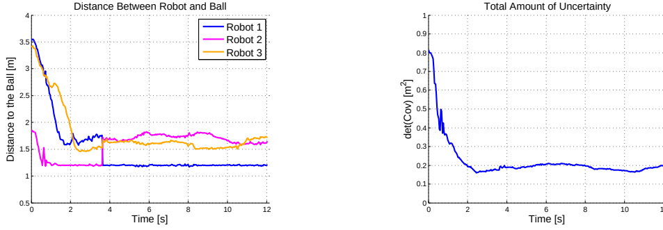
Figure 4.29: Real Experiment 1: Formation Convergence - Distance between the robot and the ball and Determinant of \Sigma_{\text{Merged}}^{\perp}(k)
