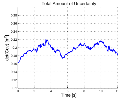
Figure 4.36: Real Experiment 4: Keeping Formation - Plot XY and Determinant of \Sigma_{\text{Merged}}^{\perp}(k)
