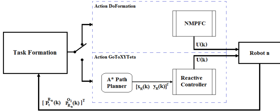
Figure 5.3: Switching approach
