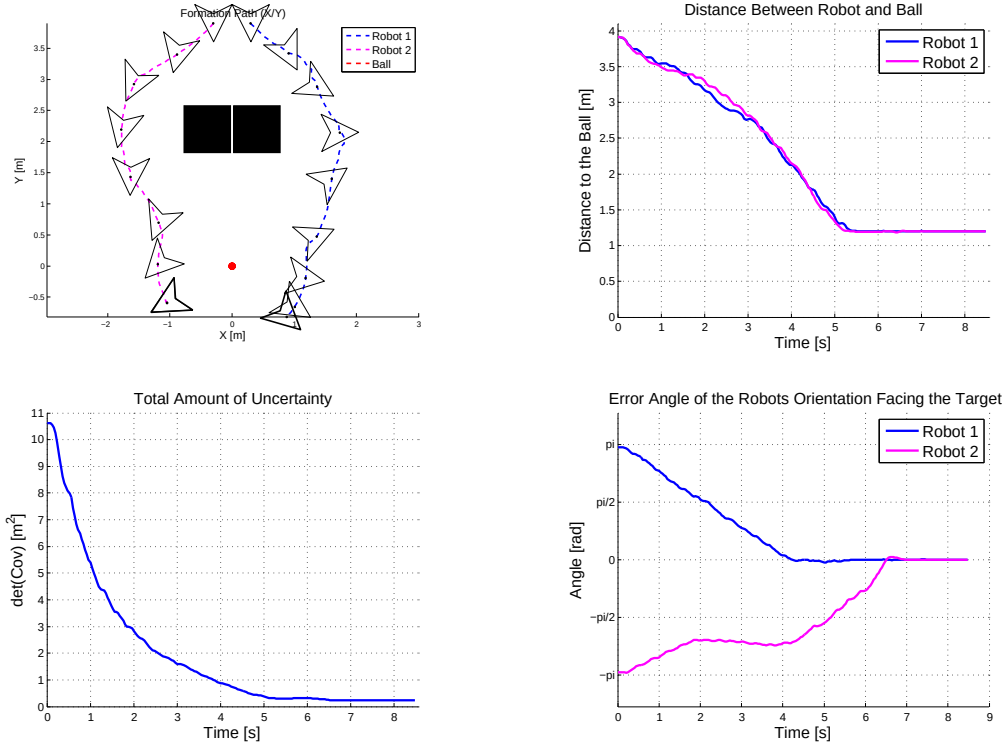
Figure 4.7: Testbed results: using the initial weights
