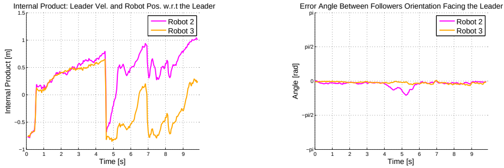
Figure 4.34: Real Experiment 3: Leader Following - Internal Product Between Leader and Followers and Error Angle of the Followers Orientation Facing the Leader
