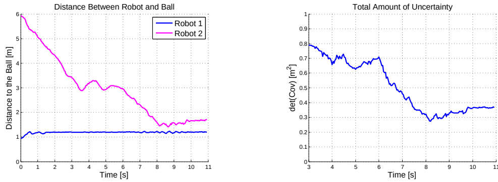
Figure 5.19: Real Experiment 2 - Distance between Robot and Determinant of \Sigma_{\text{Merged}}^{\perp}
