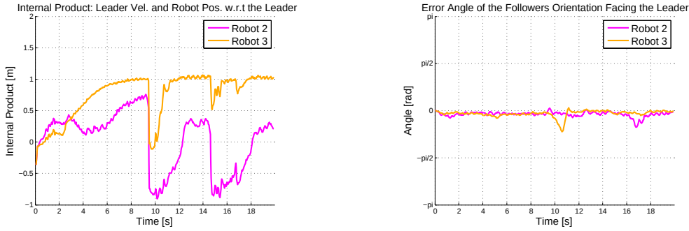
Figure 4.18: Simulation 3: Homogeneous Leader Following - Internal Product Between Leader and Followers and Error Angle of the Followers Orientation Facing the Leader
