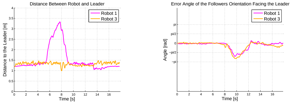
Figure 5.7: Simulation 1: Homogeneous Formation - Distance between Robot and Leader and Angle Between the Leader and the Followers
