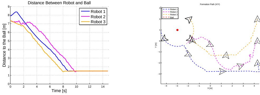
Figure 6.9: Simulation 3: Distance Robot-Ball and Plot XY of the Robots Path
