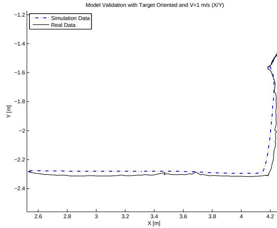
Figure 3.16: Test with 1\text{m/s} and \theta = \text{Variable}
