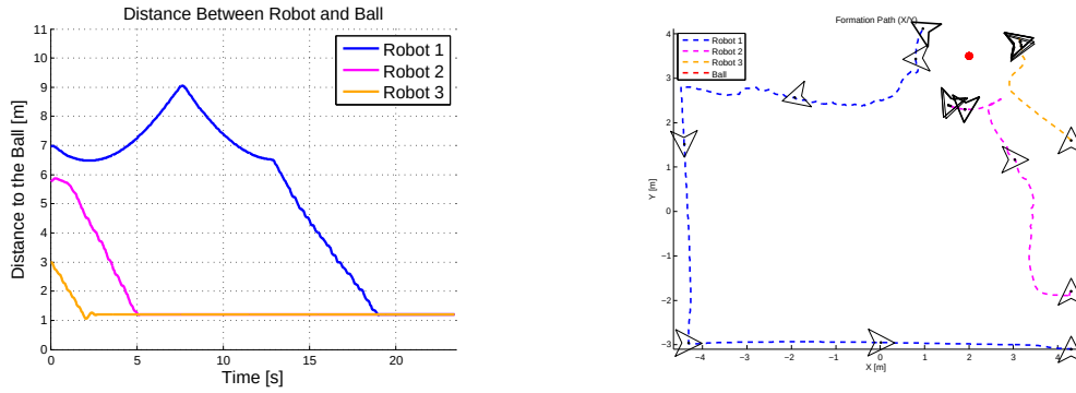
Figure 6.5: Simulation 1: Distance Robot-Ball and Plot XY of the Robots Path
