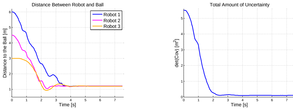
Figure 4.16: Simulation 2: Heterogeneous Formation Convergence - Distance between Robot and Ball and the Determinant of \Sigma_{\text{Merged}}^{\perp}
