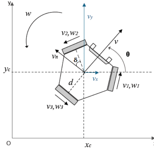
Figure 4.3: The 5dpo robot graph representation.
