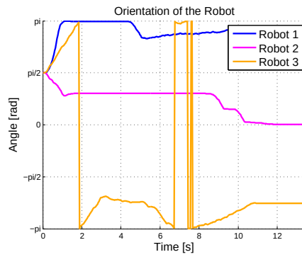
Figure 6.8: Simulation 2: Orientation of the robots
