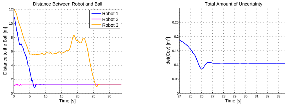
Figure 5.13: Simulation 2: Heterogeneous Formation - Distance between Robot and Ball and the Determinant of \Sigma_{\text{Merged}}^{\perp}
