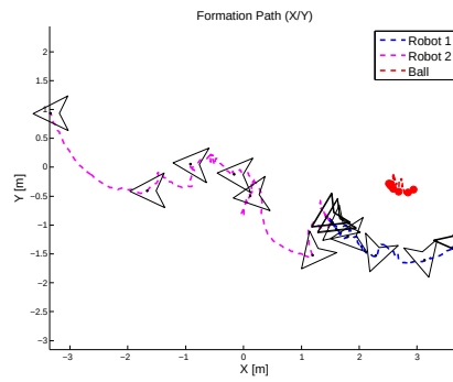
Figure 5.20: Real Experiment 3 - Plot XY
