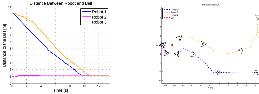
Figure 6.7: Simulation 2: Distance Robot-Ball and Plot XY of the Robots Path
