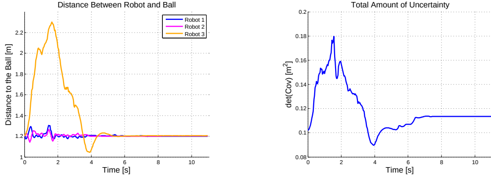
Figure 4.25: Simulation 4: Heterogeneous Keeping Formation - Distance between Robot and Determinant of \Sigma_{\text{Merged}}^{\perp}
