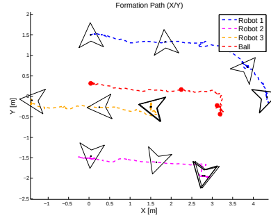
Figure 4.35: Real Experiment 4: Keeping Formation
