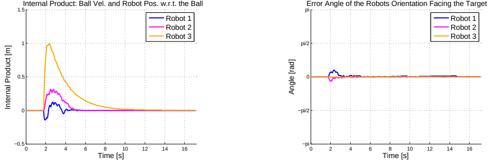
Figure 4.23: Simulation 4: Homogeneous Keeping Formation - Internal Product Between the Robots and the Ball and Error Angle of the Robots Orientation Facing the Target
