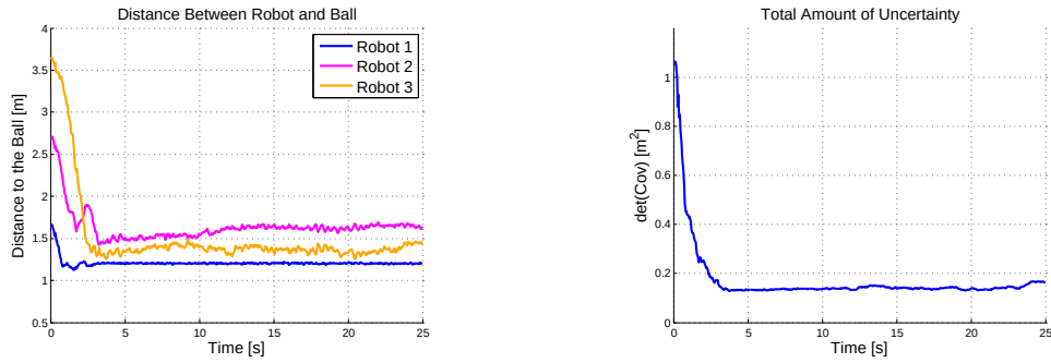
Figure 4.31: Real Experiment 2: Formation Convergence - Distance between the robot and the ball and Determinant of \Sigma_{\text{Merged}}^{\perp}(k)
