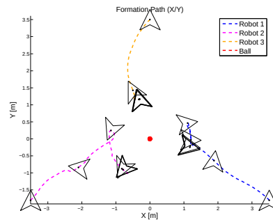
Figure 4.9: Simulation 1: Homogeneous Formation Convergence - Plot XY
