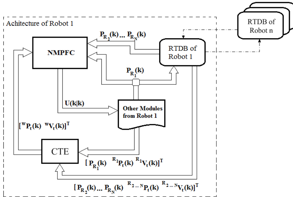
Figure 4.2: Controller Diagram
