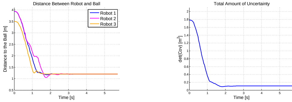
Figure 4.10: Simulation 1: Homogeneous Formation Convergence - Distance between Robot and Determinant of \Sigma_{\text{Merged}}^{\perp}(k)
