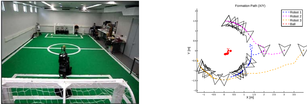
Figure 4.30: Real Experiment 2: Formation Convergence
