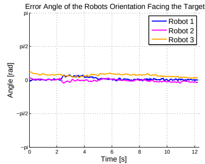
Figure 4.37: Real Experiment 4: Keeping Formation - Internal Product Between the Robots and the Ball and Error Angle of the Robots Orientation Facing the Target
