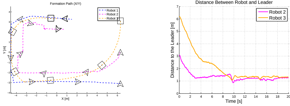
Figure 4.19: Simulation 3: Heterogeneous Leader Following - Plot XY and the Distance between the Leader Robot
