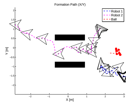
Figure 5.16: Real Experiment 1 - Environment and Plot XY
