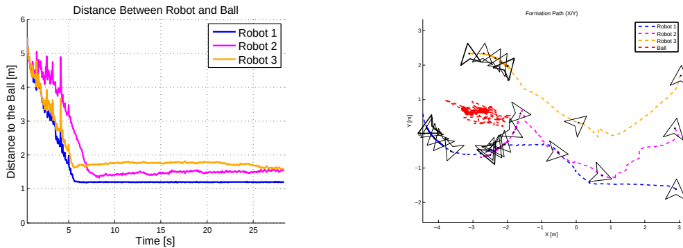
Figure 6.10: Real Experiment: Distance Robot-Ball and Plot XY of the Robots Path
