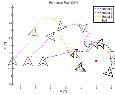
Figure 4.13: Simulation 2: Homogeneous Formation Convergence - Plot XY
