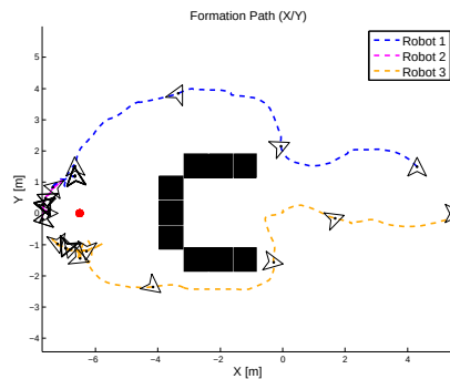
Figure 5.10: Simulation 2: Homogeneous Formation - Plot XY
