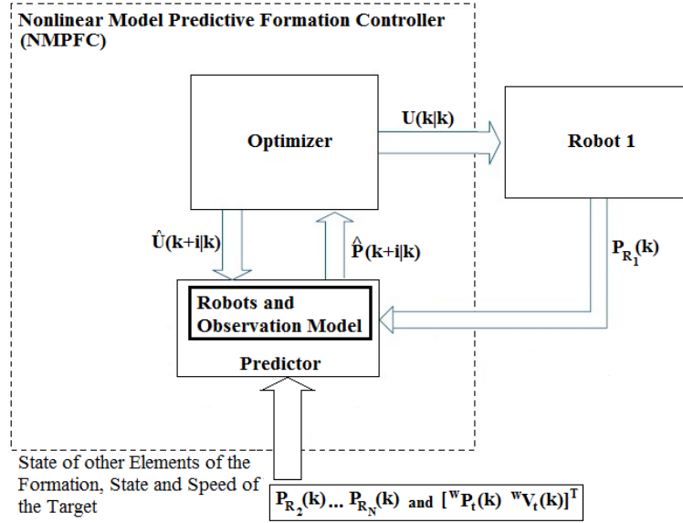
Figure 4.1: Structure of the Nonlinear Model Predictive Formation Controller Applied to robot 1
