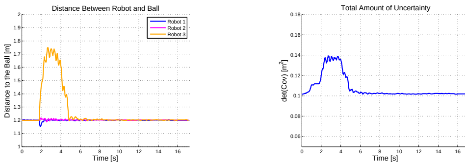
Figure 4.22: Simulation 4: Homogeneous Keeping Formation - Distance between Robot and Ball and Determinant of \Sigma_{\text{Merged}}^{\perp}(k)
