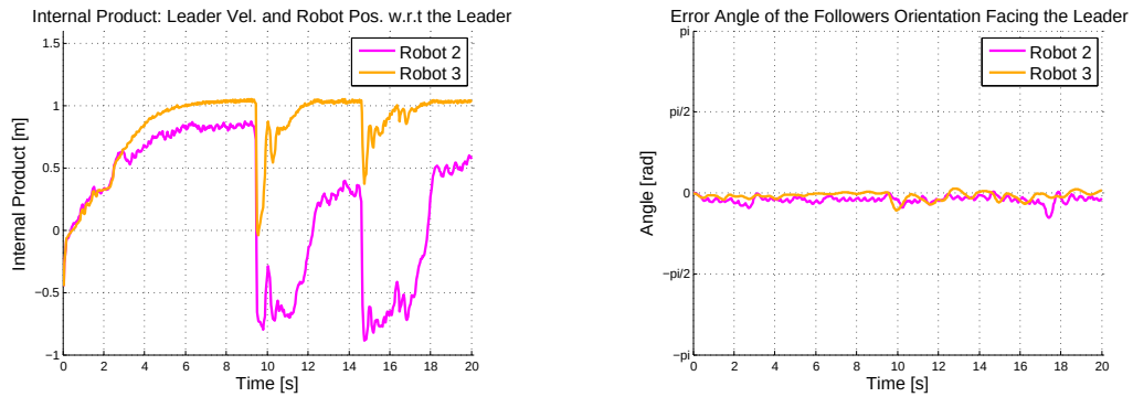
Figure 4.20: Simulation 3: Heterogeneous Leader Following - Internal Product Between Leader and Followers and Angle Between the Leader and the Followers
