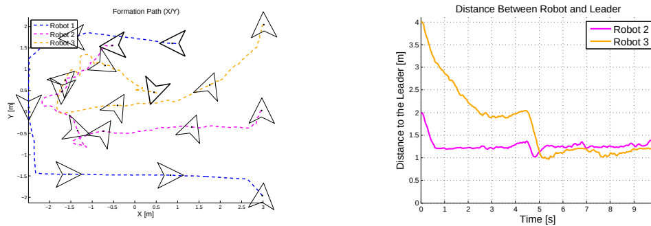
Figure 4.33: Real Experiment 3: Leader Following - Plot XY and Distance between the Leader Robot and the Followers
