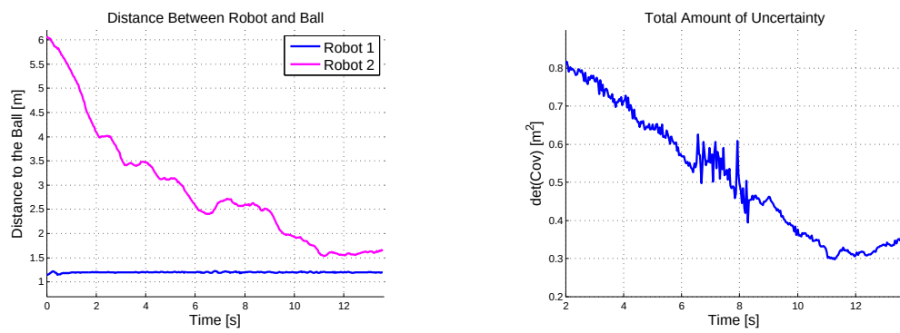
Figure 5.21: Real Experiment 3 - Distance between Robot and Determinant of \Sigma_{\text{Merged}}^{\perp}
