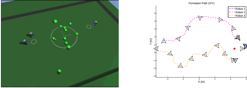
Figure 5.14: Simulation 3 - Environment and Plot XY
