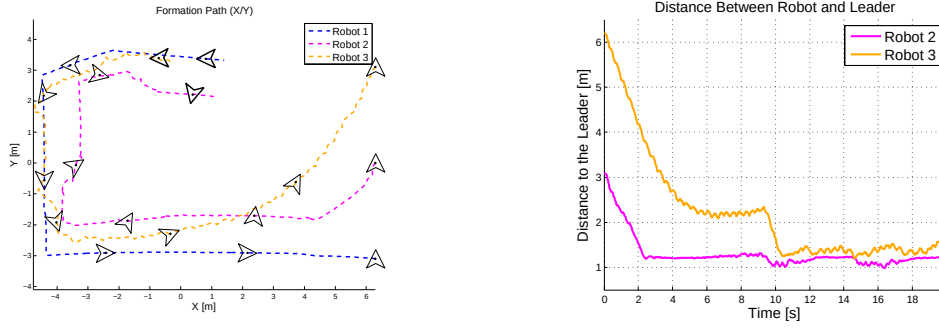
Figure 4.17: Simulation 3: Homogeneous Leader Following - Plot XY and Distance between the Leader Robot and the Followers
