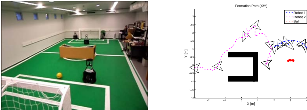
Figure 5.18: Real Experiment 2 - Environment and Plot XY
