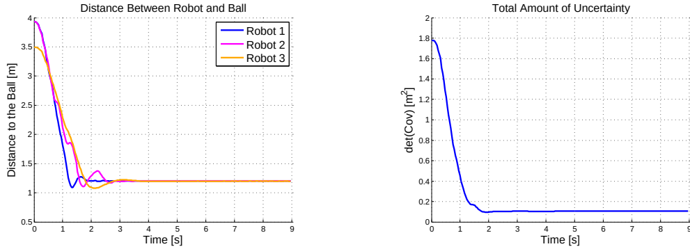
Figure 4.12: Simulation 1: Heterogeneous Formation Convergence - Distance between Robot and Ball and the Determinant of \Sigma_{\text{Merged}}^{\perp}
