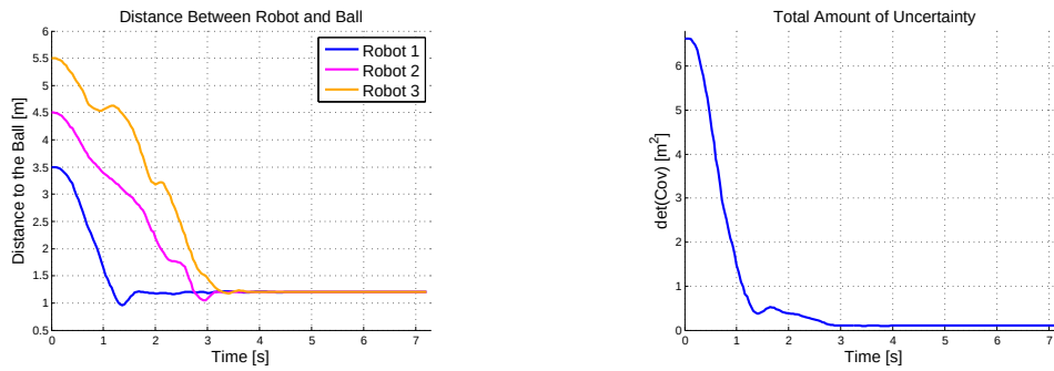
Figure 4.14: Simulation 2: Homogeneous Formation Convergence - Distance between Robot and Determinant of \Sigma_{\text{Merged}}^{\perp}(k)
