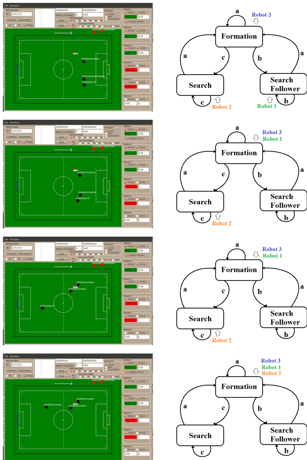
Figure 6.6: Simulation 1
