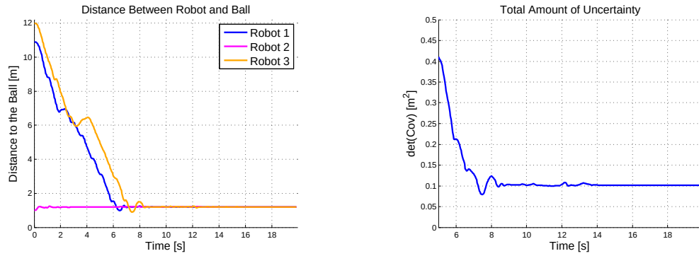
Figure 5.11: Simulation 2: Homogeneous Formation - Distance between Robot and Determinant of \Sigma_{\text{Merged}}^{\perp}
