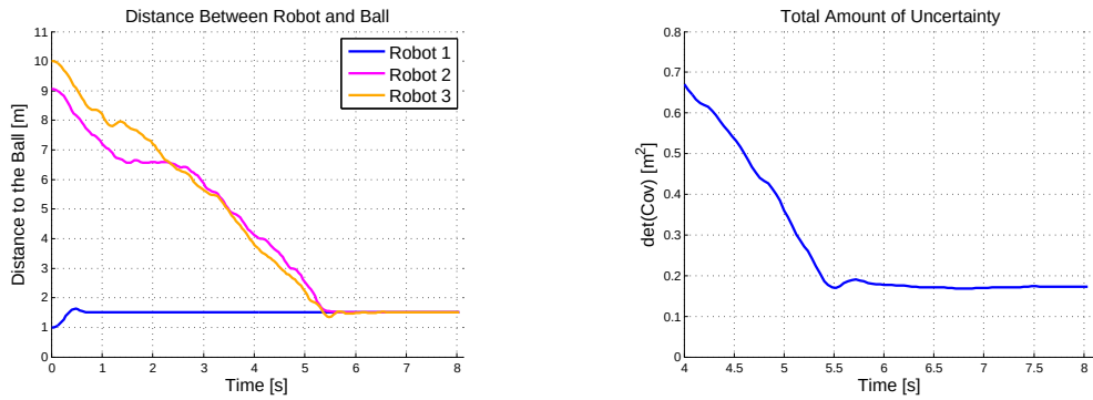
Figure 5.15: Simulation 3 - Distance between Robot and Ball and Determinant of \Sigma_{\text{Merged}}^{\perp}
