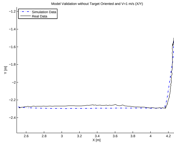
Figure 3.15: Test with 1\text{m/s} and \theta = 0^\circ
