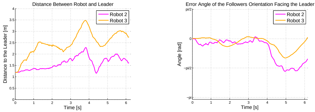
Figure 5.9: Simulation 1: Heterogeneous Formation - Distance between Robot and Leader and Angle Between the Leader and the Followers
