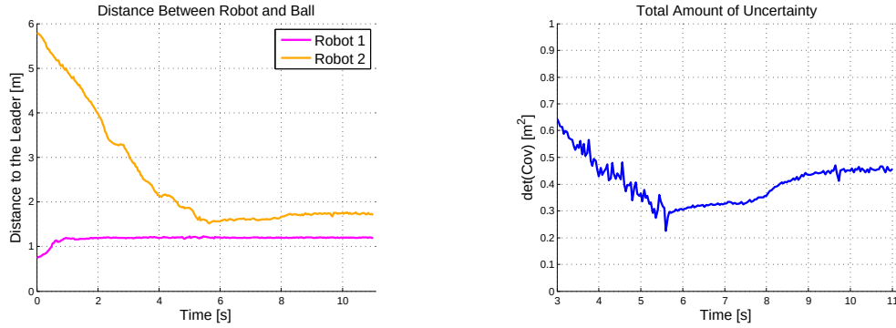
Figure 5.17: Real Experiment 1 - Distance between Robot and the Ball and Determinant of \Sigma_{\text{Merged}}^{\perp}
