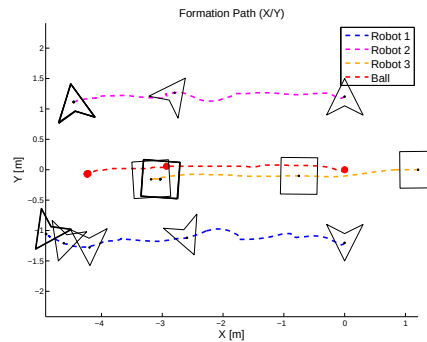
Figure 4.24: Simulation 4: Heterogeneous Keeping Formation - Plot XY
