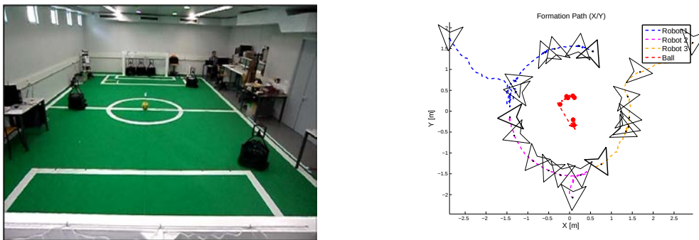
Figure 4.28: Real Experiment 1: Formation Convergence
