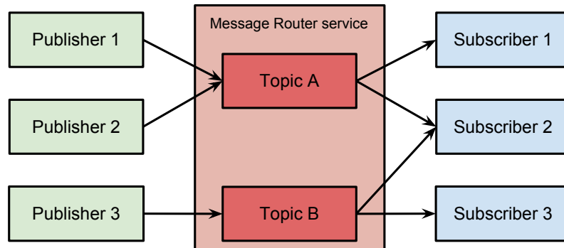
Figure 3.5: Publisher/Subscriber pattern and message routing example.
