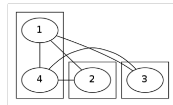
(c) Recursive Bisection
