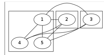
(c) Recursive Bisection
