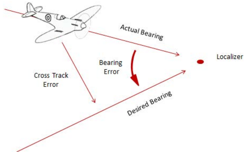
Figure 3.9: Localizer
