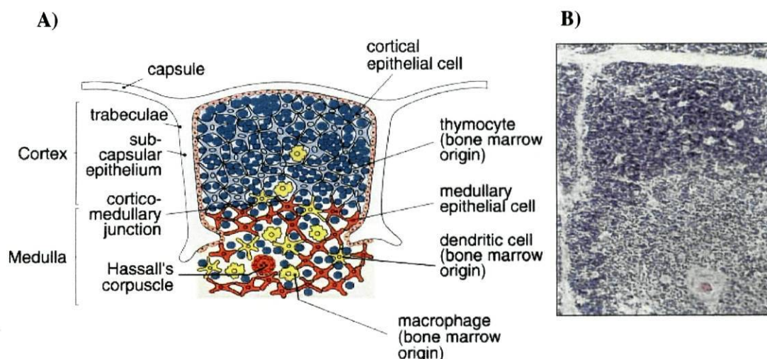
Figure 1- The Thymus: Its structure and its cellular content. The figure shows the histology of the organ (B), and the distribution of the different cell types in the identifiable areas (A). (From Janeway, C. et al., 1999)
