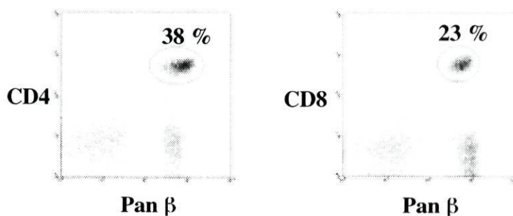
Figure 8: T cell populations in the Lymph nodes. The figure shows the FACS analysis of a Lymph node cell suspension obtained from a 8 weeks old C57Bl6 mouse, after staining with the indicated antibodies. The numbers represent the percentages of cells in the regions displayed.
