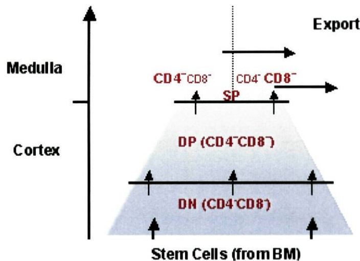
Figure 2: Differentiation along the T cell pathway in the Thymus
