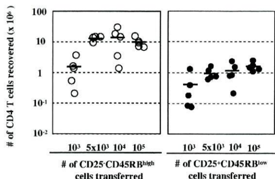
FIGURE 4. Expansion capacity of CD4 T cell populations of C57BL/6 mice. Different numbers of purified naive CD4 + and CD25 + CD4 + T cells (1,000–100,000) were transferred into CD3 \epsilon^{-/-} mice. The results show the number of CD4 T cells recovered 10–11 wk after transfer in the spleen and LN of each individual host (the mean value is also shown).
