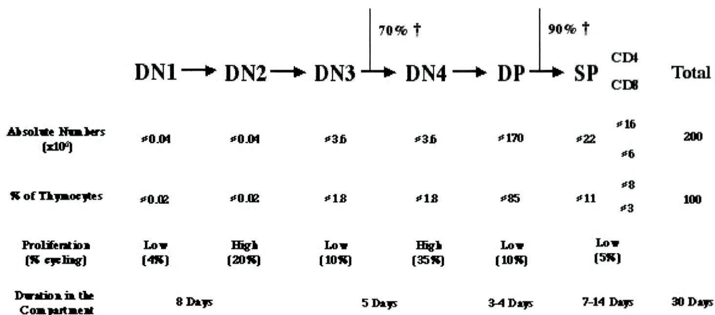
Figure 4: Kinetics and quantitative aspects of T cell development. Absolute numbers are calculated for a young adult mouse (200x10 6 thymocytes). The % of cycling cells is given as found after one single pulse labeling of BrDU. Data compiled from several studies (Egerton, 1990; Ernst, 1995; Huesmann, 1991; Lucas, 1994; Penit, 1995; Scollay, 1995).
