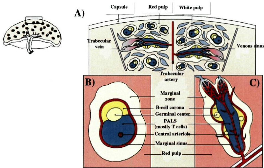
Figure 5: The Spleen. The figure shows a schematic representation of the selected area of the spleen. A) Structure of the spleen. The true lymphoid tissue of the spleen is contained in the white pulp. The bulk of the white pulp is arranged around a central arteriole and inside a marginal sinus (see also B and C, transverse and longitudinal sections of the white pulp, respectively). We can also distinguish the periarteriolar lymphoid sheath (PALS) consisted by a majority of T cells, and flanked by B cells. B cells can be organized in follicles. Secondary follicles form germinal centers (B and C). (Modified from Janeway et al., 1999).
