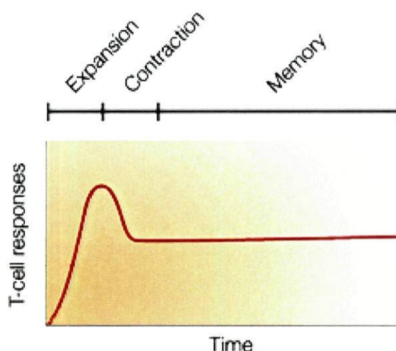
Figure 10: Immune responses. The Immune response consists of three distinct phases. See text for the quantitative correspondence. (Modified from Kaech et al., 2002).
