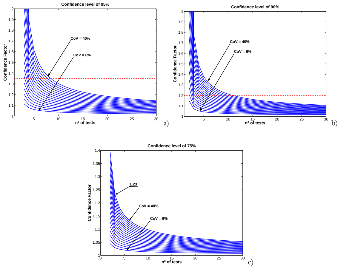
Figure 4.2. Values of CF_{LLM} considering a normal distributed strength with unknown variance, for increasing values of n , for the selected range of \overline{CoV} s and for (1-\alpha) confidence levels of 95% (a), 90% (b) and 75% (c).
