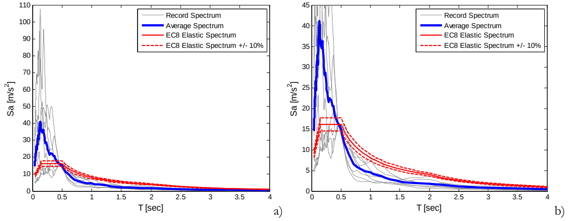
Figure 3.8. Response spectra of the S_a(T_1) scaled records for the limit state of NC and frame TF1 , their average spectrum and the EC8-1 elastic response spectrum \pm 10\% (a); larger view (b).
