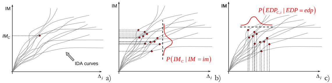
Figure 9.6. Illustration of step 9 (a), of step 11 considering n_{UC} = 1 (b) and of step 13 considering n_{UC} = 1 and for the i th storey (c).
