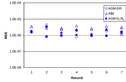
Figure 2.14. Mean squared error (MSE) values, Eq. (2.14), of the alternative CRQMs for the limit state of DL from the seven artificial records, for column (a) and beam (b) sections.
