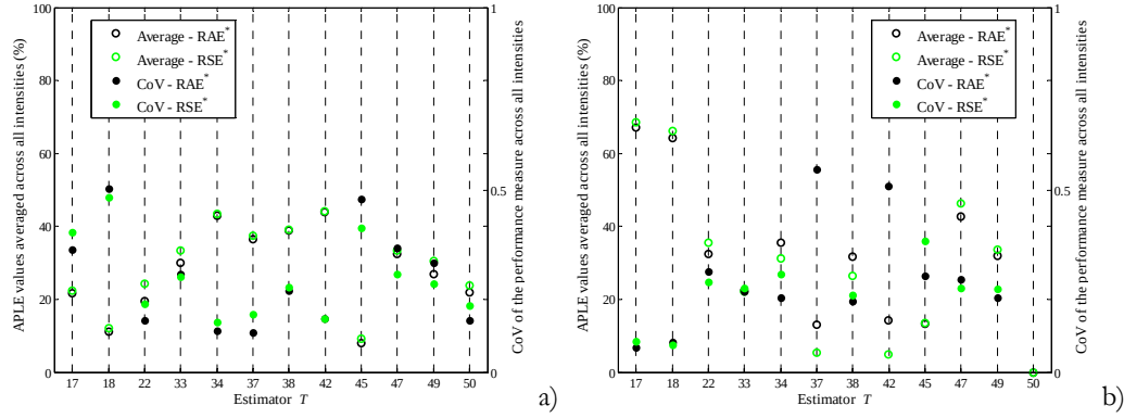
Figure 6.18. APLE values of the estimators averaged across all the intensities along with the CoVs representing the variability between intensities, for the RSE^* and RAE^* , for the ICONS shear force in original units, when S_a(T_1) is the IM when n^* is forty (a) and seven (b).
