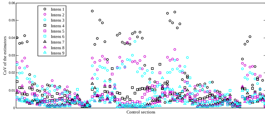
Figure 6.12. CoV of the central values obtained by all the estimators for the REG10 shear force in original units when PGA is the IM, for all the intensities and control sections.
