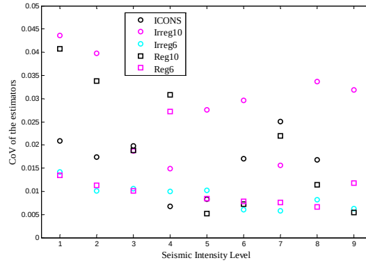
Figure 6.14. CoV of the central values obtained by all the estimators, for the inter-storey drift of all structures and for all the intensities, when S_a(T_1) is the IM.
