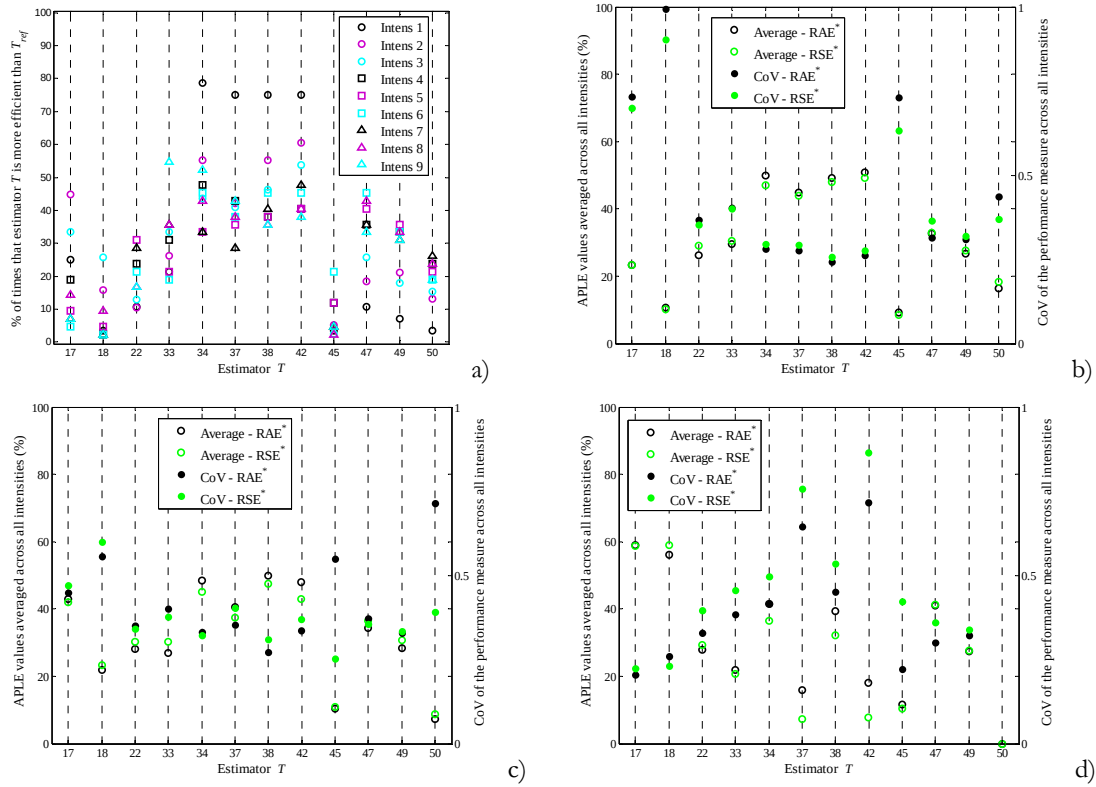
Figure 6.15. APLE values of the estimators for the IRREG6 positive chord rotation when PGA is the IM, for the RSE* and all the intensities (a); for the RSE* and RAE* averaged across all the intensities along with the CoVs representing the variability between intensities when n^* is thirty (b); fifteen (c); and seven (d).
