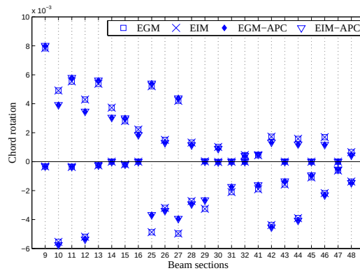
Figure 2.18. Performance of the EGM, the EIM, the EGM-APC and the EIM-APC for the limit state of DL considering one of the ReLUIS records for beam sections.
