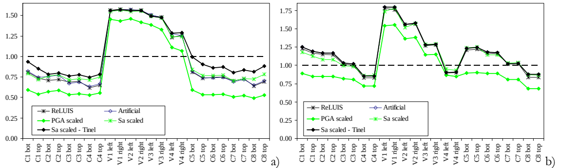
Figure 3.19. Safety assessment results of frame TF2 (a) and frame TF2 (b) considering different accelerogram sets, for the shear force NC limit state and KL3.
