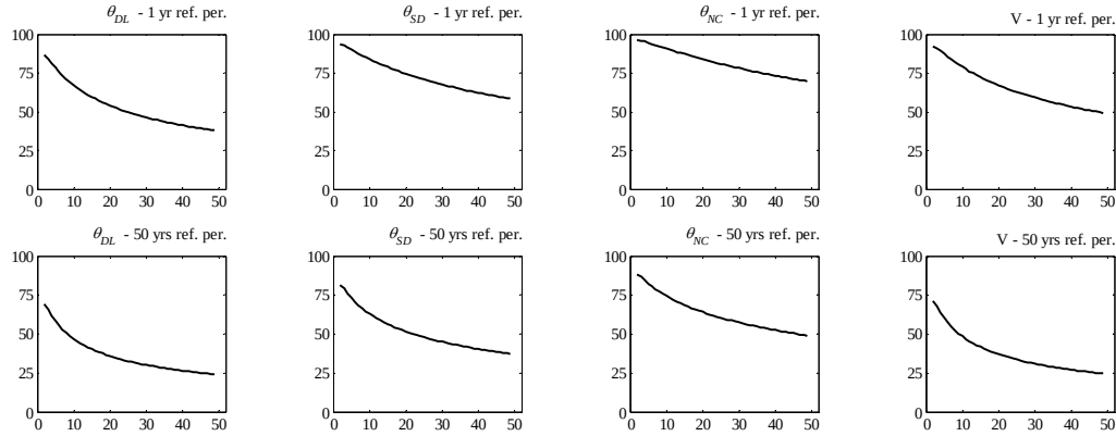
Figure 8.11. Evolution of the average of the SE_{\mu} , expressed as percentages of \mu_{LS} , for the chord rotation and shear force limit states of section 2 and the reference periods of 1 year and 50 years.
