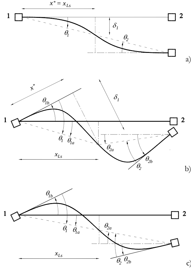
Figure 2.1. Examples of the chord rotation definition.
