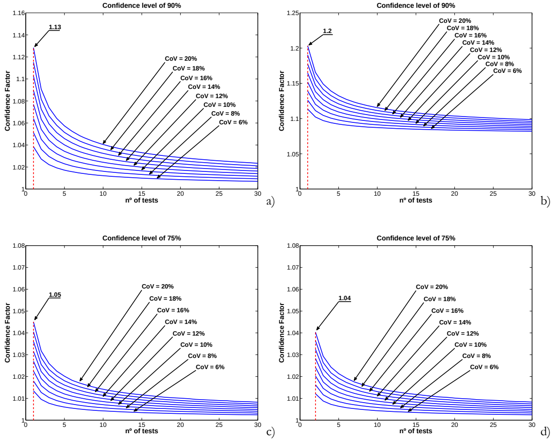
Figure 4.5. Values of CF_{LIM} obtained by simulation considering a normal distributed strength, the existence of prior knowledge, for increasing values of n , for the selected range of CoVs, for KL2 (confidence level of 90%) when the prior information and the new test data are in agreement (a), when the prior information exceeds the mean of the new test data by 15% (b); for KL3 (confidence level of 75%) when the prior information and the new test data are in agreement (c) and when the prior information and the new test data are in agreement and s_0 is known (d).
