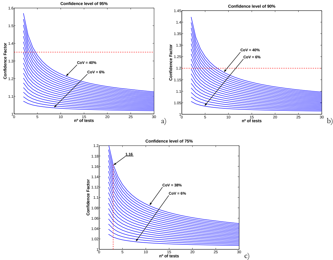
Figure 4.3. Values of CF_{LIM} considering a lognormal distributed strength with unknown variance, for increasing values of n , for the selected range of \overline{CoV} s and for (1-\alpha) confidence levels of 95% (a), 90% (b) and 75% (c).
