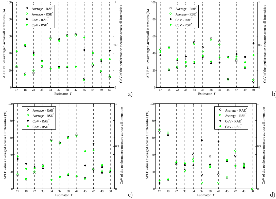
Figure 6.21. APLE values of the estimators, for the RSE^* and RAE^* averaged across all the intensities, along with the CoVs representing the variability between intensities, and obtained using T_{Ham, 3} as the reference estimator , for the IRREG6 positive chord rotation when PGA is the IM, when n^* is thirty (a) and fifteen (b); for the ICONS shear force in original units, when S_a(T_1) is the IM when n^* is forty (c) and seven (d).
