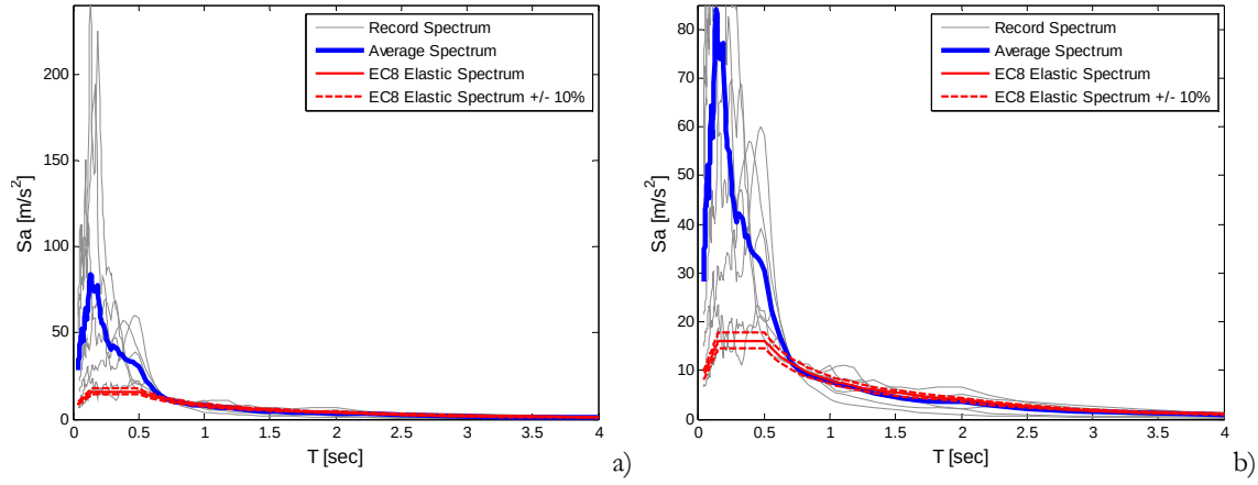
Figure 3.10. Response spectra of the S_a(T_{inel}) scaled records for the limit state of NC and frame TF1 , their average spectrum and the EC8-1 elastic response spectrum \pm 10\% (a); larger view (b).
