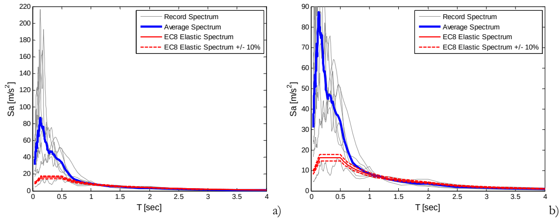
Figure 3.11. Response spectra of the S_a(T_{inel}) scaled records for the limit state of NC and frame TF2 , their average spectrum and the EC8-1 elastic response spectrum \pm 10\% (a); larger view (b).
