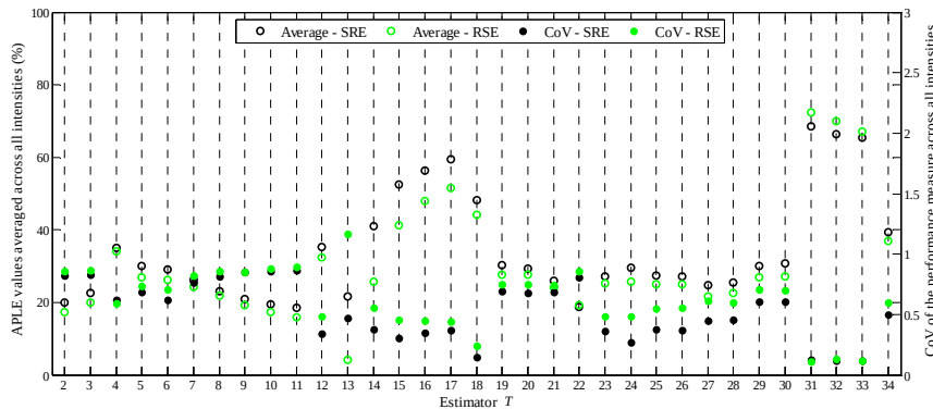
Figure 7.10. APLE values of the estimators, for the SRE and the RSE, for the REG6 shear force in log units when S_a(T_1) is the IM, averaged across all the intensities, and CoVs representing the variability between intensities.
