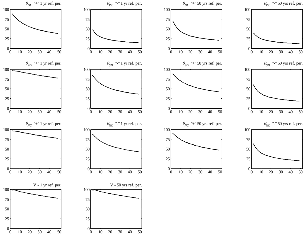
Figure 8.10. Evolution of the average of the SE_{\mu} , expressed as percentages of \mu_{LS} , for the chord rotation and shear force limit states of section 1 and the reference periods of 1 year and 50 years.
