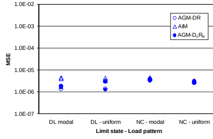
Figure 2.12. Mean squared error (MSE) values, Eq. (2.14), of the alternative CRQMs for two limit states and the pushover analysis cases, for column (a) and beam (b) sections.
