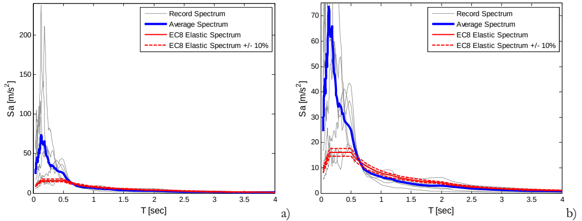
Figure 3.9. (a) Response spectra of the S_a(T_1) scaled records for the limit state of NC and frame TF2 , their average spectrum and the EC8-1 elastic response spectrum \pm 10\% (a); larger view (b).
