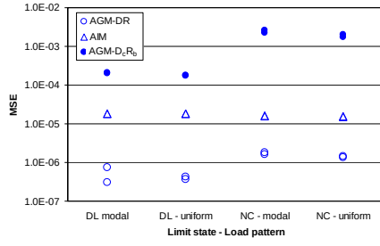
Figure 2.12. Mean squared error (MSE) values, Eq. (2.14), of the alternative CRQMs for two limit states and the pushover analysis cases, for column (a) and beam (b) sections.
