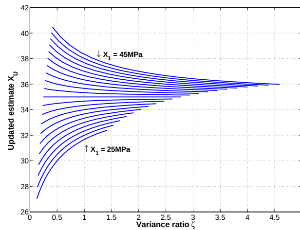
Figure 4.6. Values of X_U considering the existence of prior knowledge, for the case when both X_0 and s_0 are known.
