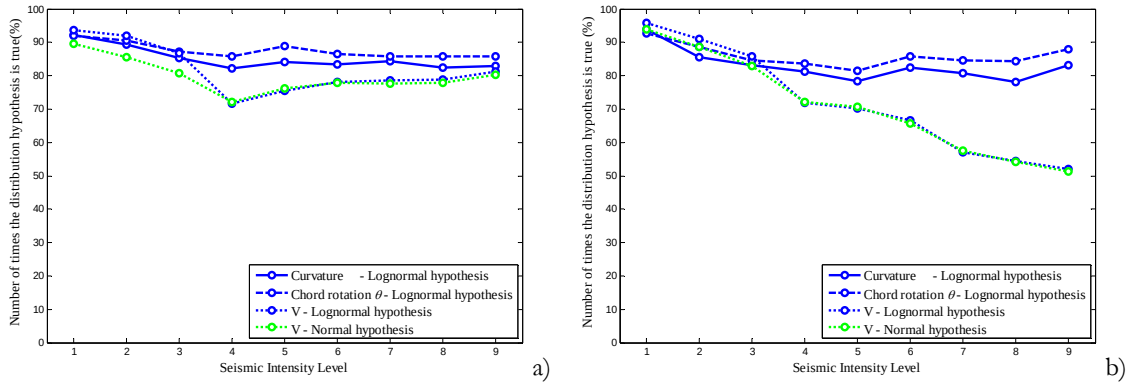
Figure 5.21. Enhanced APA results from the tests of Group 3 for the column (a) and beam (b) datasets of all the structures, when S_a is the IM.
