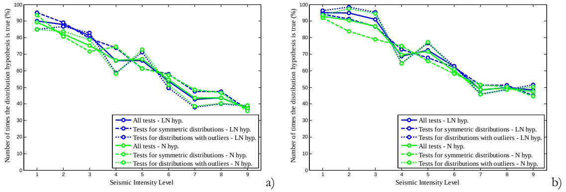
Figure 5.18. Shear force APA results (a) and enhanced APA results (b) for the beams of REG10 when \mathcal{S}_a is the IM (LN hyp. is the lognormal hypothesis and N hyp. is the normal hypothesis)
