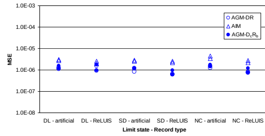
Figure 2.15. Mean squared error (MSE) values, Eq. (2.14), of the alternative CRQMs for all the limit states, for the two record sets based on the average chord rotation demand, for column (a) and beam (b) sections.
