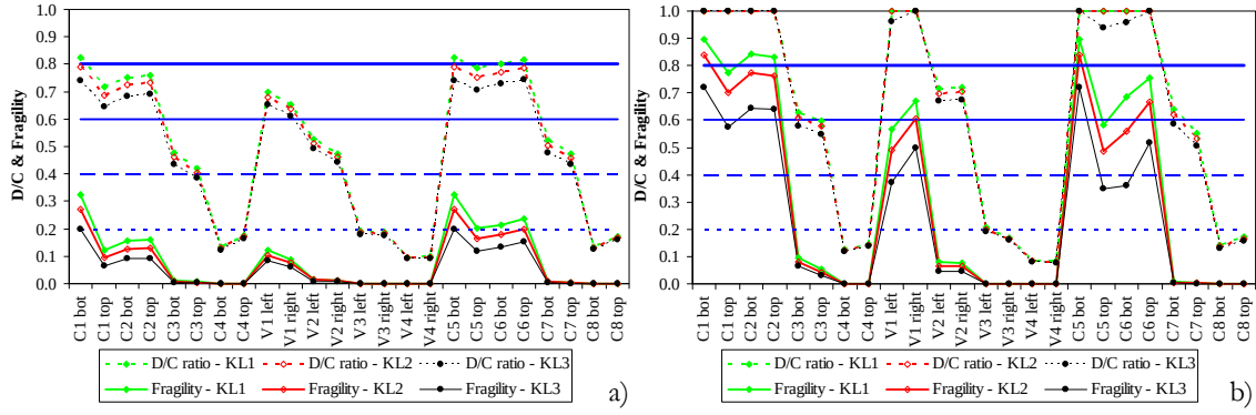
Figure 3.23. Fragility values vs deterministic D/C ratios for frame TF2 considering the three KLs, artificial accelerograms, the SD chord rotation limit state (a) and the NC chord rotation limit state (b).
