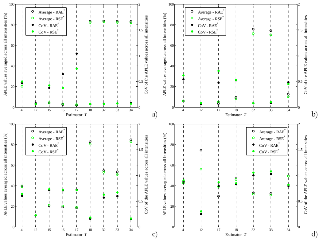
Figure 7.20. APLE values of the estimators averaged across all the intensities along with the CoVs representing the variability between intensities, for the RSE^* and RAE^* values, when S_a(T_i) is the IM, for the ICONS positive curvature when n^* is forty (a) and when n^* is seven (b), and when PGA is the IM, for the IRREG10 shear force in log units when n^* equal to forty (c), and for the shear force in original units when n^* equal to seven (d).
