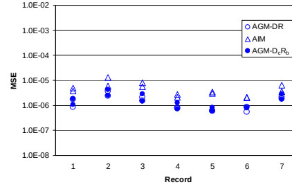
Figure 2.13. Mean squared error (MSE) values, Eq. (2.14), of the alternative CRQMs for the limit state of NC from the seven ReLUIS records, for column (a) and beam (b) sections.
