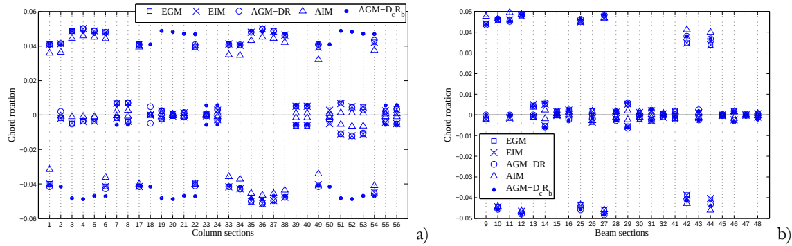
Figure 2.6. Performance of several CRQMs for the limit state of NC considering pushover analysis with modal loading pattern, for column (a) and beam (b) sections.
