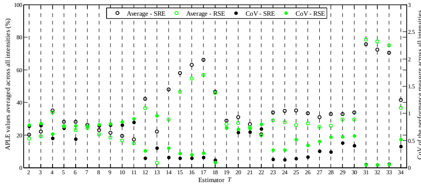
Figure 7.9. APLE values of the estimators, for the SRE and the RSE, for the REG6 shear force in original units when S_a(T_1) is the IM, averaged across all the intensities, and CoVs representing the variability between intensities.
