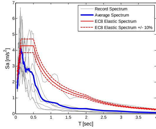
Figure 3.7. Response spectra of the PGA scaled records for the limit state of DL, their average spectrum and the EC8-1 elastic response spectrum \pm 10\% .
