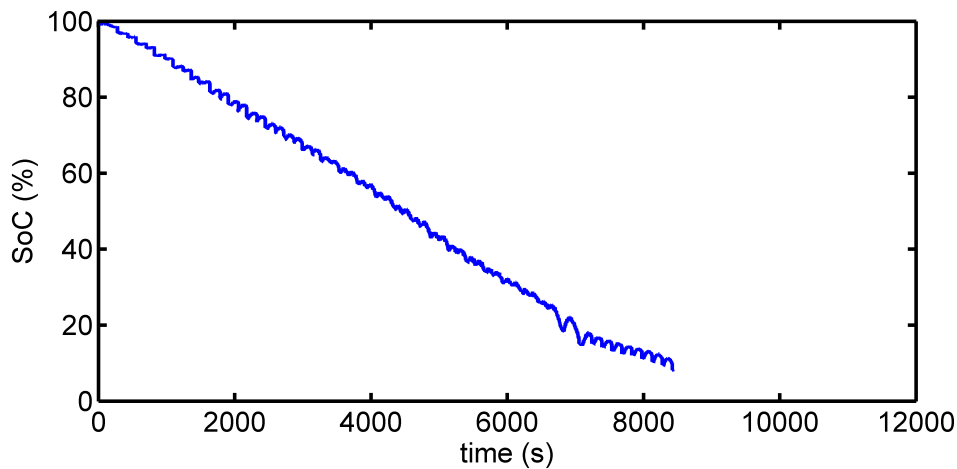
Figure 4.25: Validation of the ANN Method
