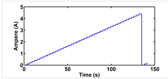
Figure 4.7: Discharge Current Behaviour
