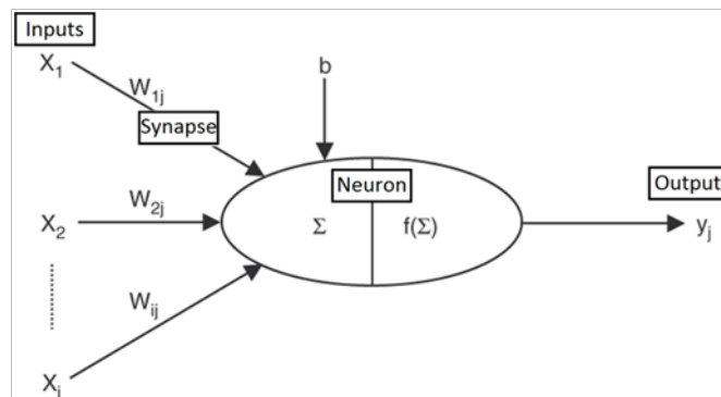
Figure 4.19: Basic Structure of an Artificial Neural Network
