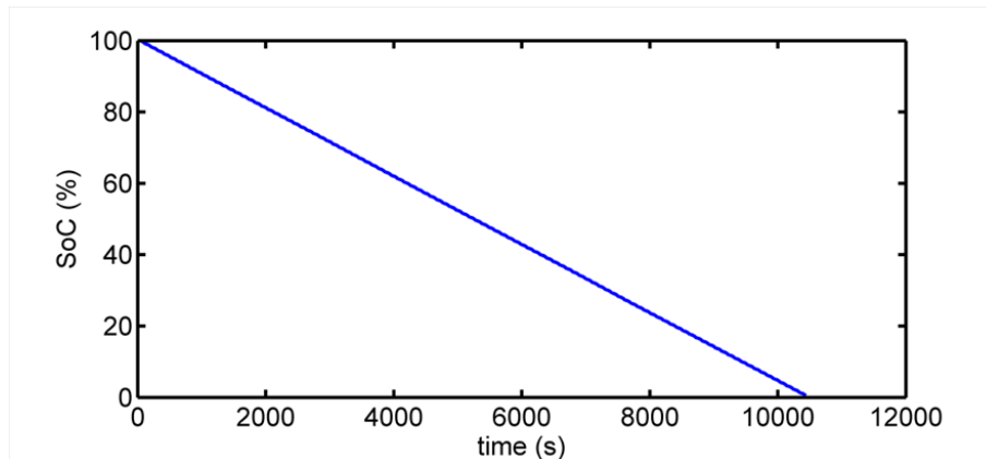
Figure 4.16: SoC Estimation Result of Pulsed Current Discharge Using the Ampere-hour Counting Method
