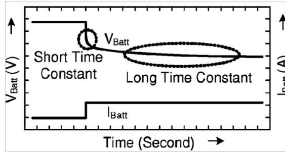
Figure 2.10: Circuit with a response to a current step [47]
