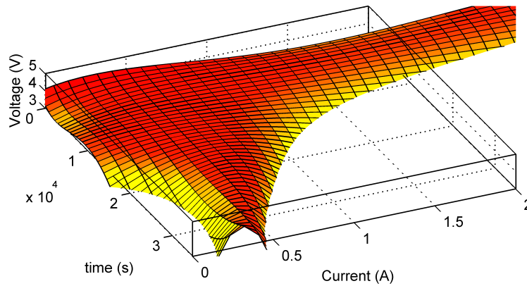
Figure 3.16: surface fitted with high-order polynomial equation
