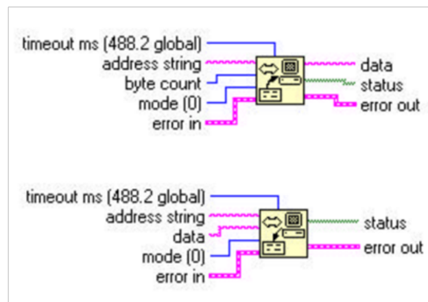
Figure 3.8: Reading and Writing Blocks of LabVIEW
