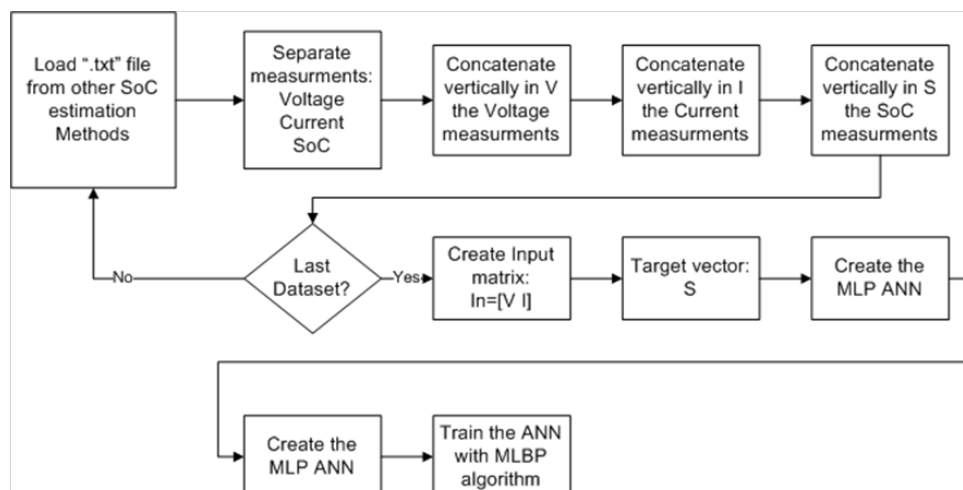
Figure 4.24: Initial Conditions for the ANN Method
