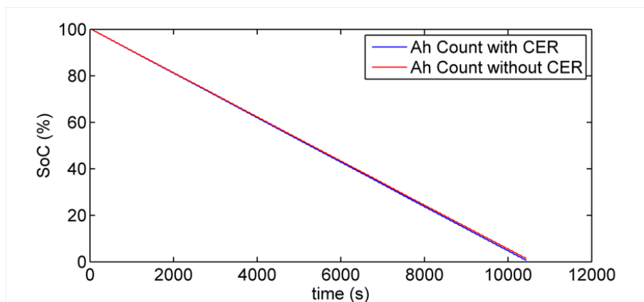
Figure 4.17: Comparison between Ampere Hour counting method with and without CER
