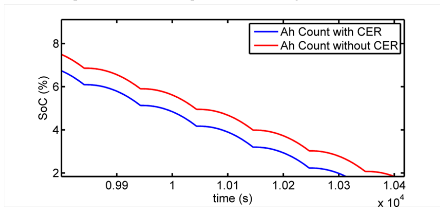
Figure 4.18: Comparison between Ampere Hour counting method with and without CER in detail
