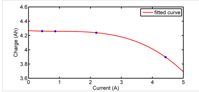
Figure 4.14: Non-linear Relation Between the Current Demanded by the Load and the Charge
