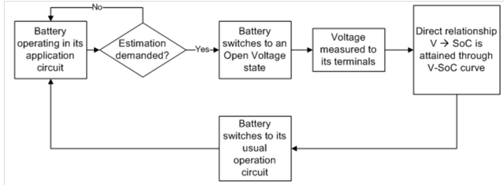
Figure 4.9: Open Circuit Voltage Software Description
