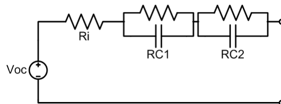
Figure 2.9: Electrical Circuit
