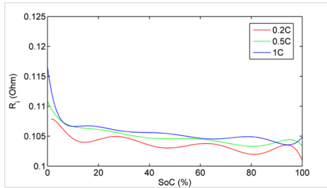
Figure 3.20: Internal Resistance
