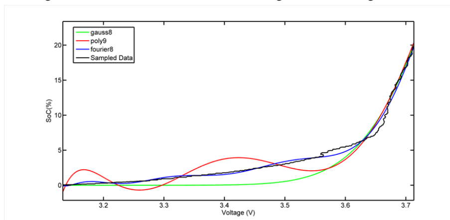
Figure 4.12: V-Soc curves in detail
