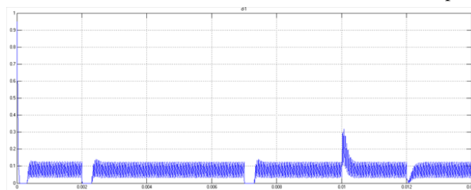
Figure 5.15: Duty-Cycle Saturation
