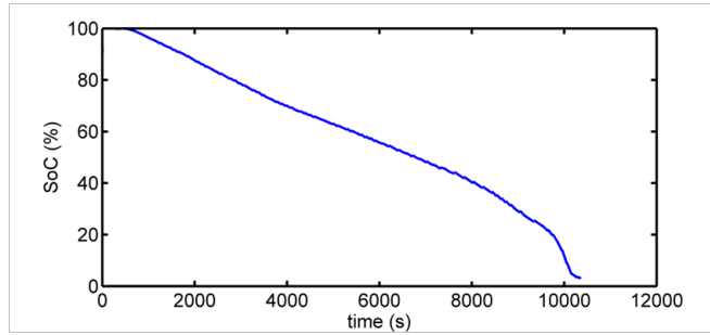
Figure 4.8: Discharge SoC
