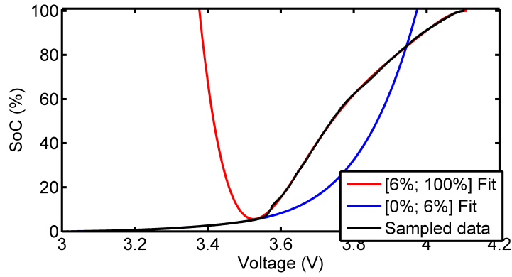
Figure 4.6: Two regions V-SoC curve determination in the Discharge Test
