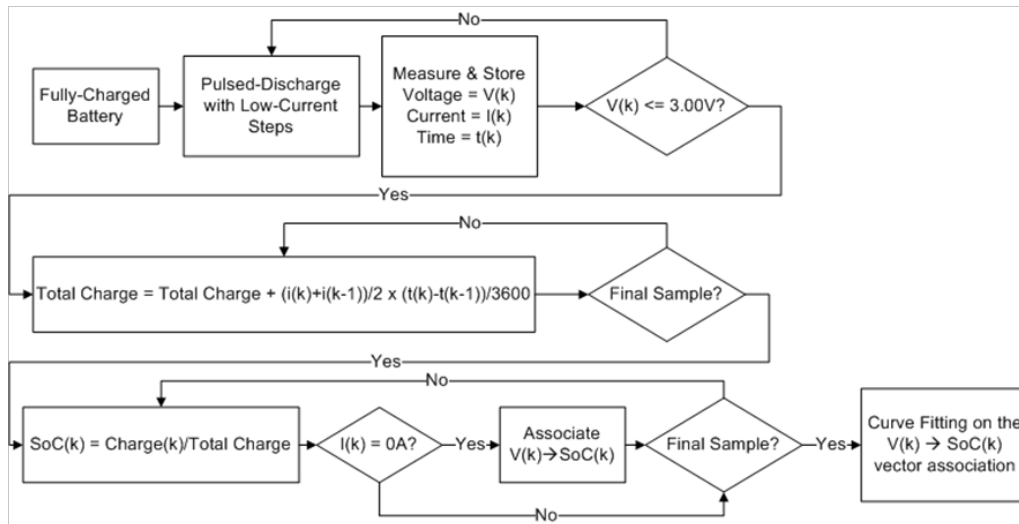
Figure 4.10: V-SoC curve determination in the Open Circuit Voltage Method
