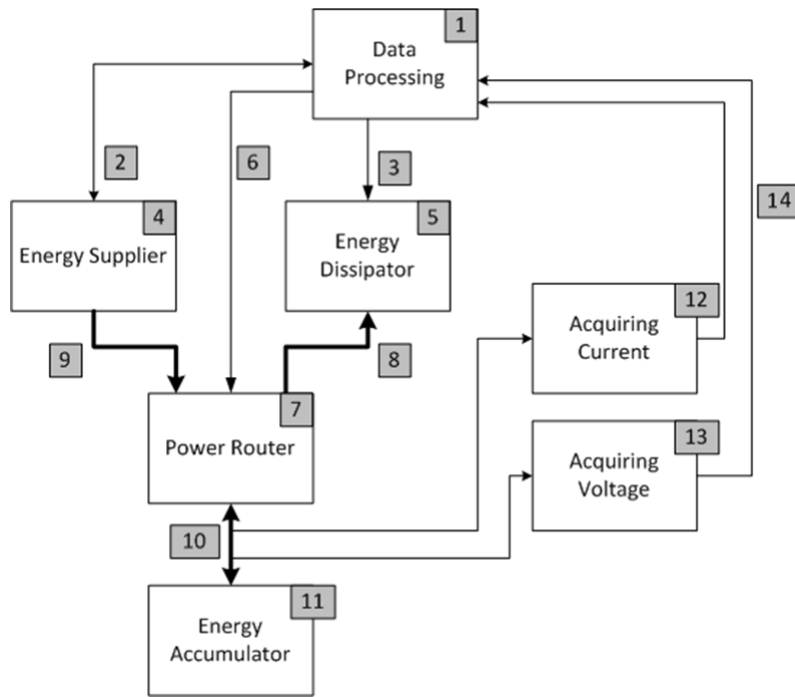
Figure 3.1: Functional Architecture
