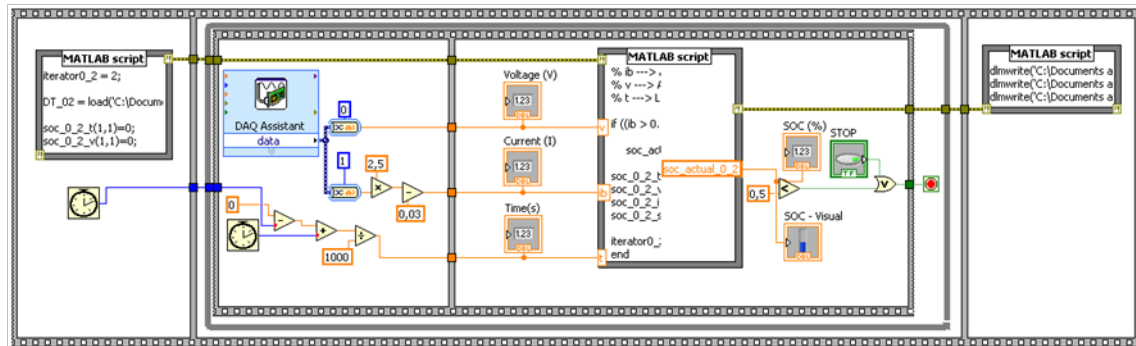
Figure 4.15: Ampere Hour Counting Labview Program
