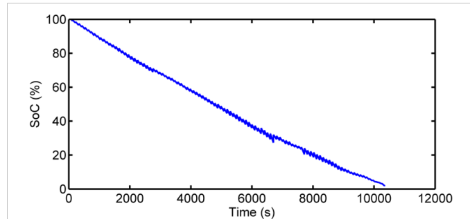
Figure 4.13: SoC obtained with the Open Circuit Voltage Method
