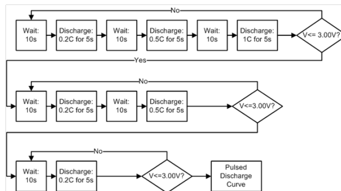
Figure 3.18: Discharge Procedure
