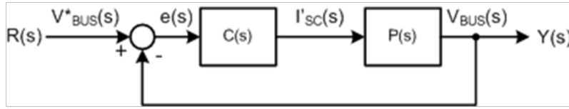
Figure 5.18: Voltage Closed-Loop Block Diagram
