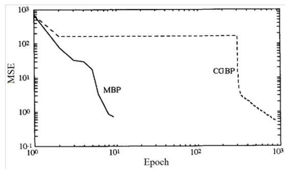
Figure 4.22: Mean Squared Error Between Output and Target on a 4-D Function Approximation with the MLBP algorithm
