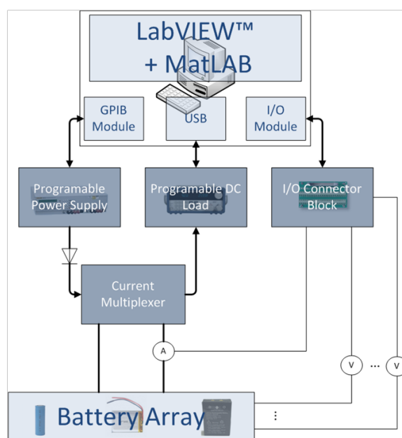
Figure 3.2: Solution Architecture
