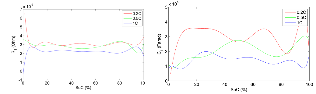
Figure 3.21: Results of the First RC Block
