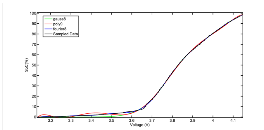
Figure 4.11: V-SoC curves obtained through various fitting methods
