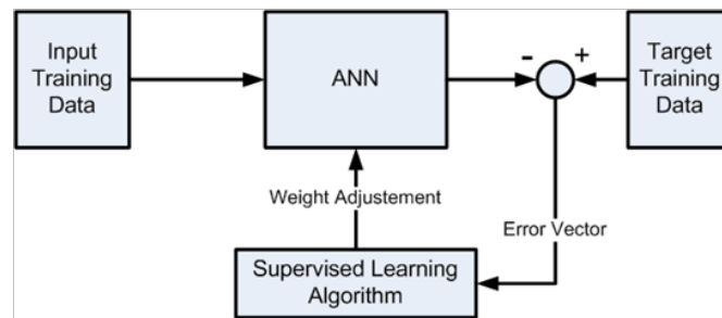
Figure 4.21: Supervised Training Method
