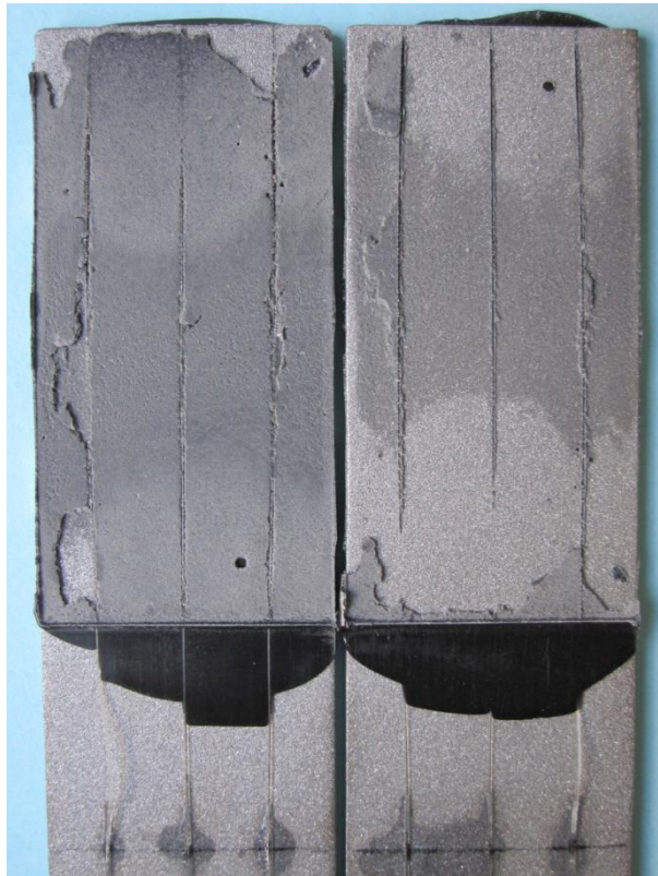
Figure 39- Fracture surface of one specimen of the fifth trial.
