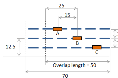
Figure 71- Sensors location.
