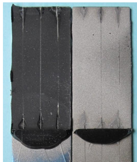
Figure 22- Fracture surface of a joint with fibers (first trial).
