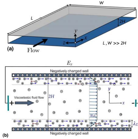
Figure 7.20: (a) Diagram of the microchannel geometry considered in the study; (b) 2D representation of electro-osmotic flow of viscoelastic fluids in the microchannel for a negatively charged wall.
