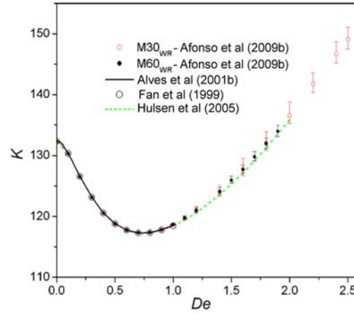
Figure 5.3: Drag force coefficient for the creeping flow of an Oldroyd-B fluid ( \beta = 0.59 ) past a cylinder. Results obtained with the \text{Log}T formulation with meshes M30_{WR} and M60_{WR} , and comparison with data from Alves et al. (2001b), Hulsén et al. (2005) and Fan et al. (1999).
