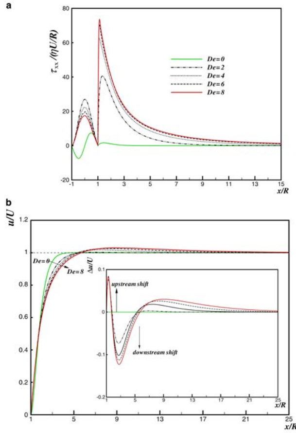
Figure 5.31: (a) \tau_{xx} and (b) u centreline profiles for the Giesekus model ( \alpha=0.02 and \beta=0.59 ). The inset shows the wake velocity difference, \Delta u/U = (u - u_{N_{ewt}})/U .
