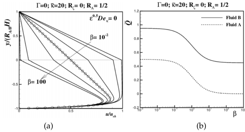
Figure 7.29: Effect of the dynamic viscosity ratio ( \beta = 10^{-2} , 10^{-1} , 1, 10 and 100) on dimensionless (a) velocity profiles and (b) volumetric flow rate for Newtonian-Newtonian flow configuration.
