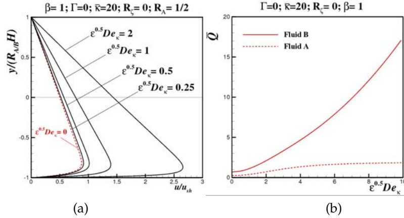
Figure 7.32: Dimensionless profiles of (a) velocity and (b) volumetric flow rate as function of \sqrt{\varepsilon} De_\kappa .
