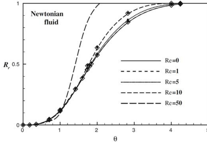
Figure 6.16: Degree of reverse flow as function of gap width, \theta , for several Reynolds numbers. Newtonian case on meshes M25 (diamond), M51 (lines) and M101 (closed circle).
