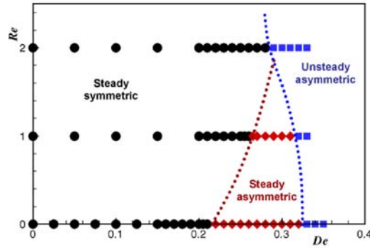
Figure 6.10: Re-De stability map for the uniaxial extension configuration ( I_o = 4 : 2 ).
