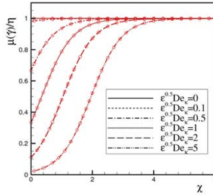
Figure 7.5: Dimensionless viscosity profiles for electro-osmotic viscoelastic flow ( \Gamma = 0 ) of a PTT fluid as function of \sqrt{\varepsilon} De_\kappa for relative microchannel ratios of \bar{\kappa} = 20 (lines) and \bar{\kappa} = 100 (lines and symbols). \chi = (1 - \bar{y}) \bar{\kappa} is the near wall variable.
