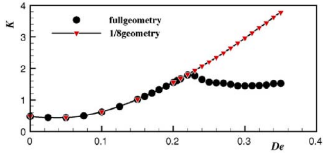
Figure 6.11: Effect of Deborah number on the dimensionless extra power dissipation ( K ) for the uniaxial extension configuration ( I_o = 4 : 2 ). Simulations with full geometry ( \bullet ) and 1/8 of the geometry (imposed flow symmetry) ( \nabla ).
