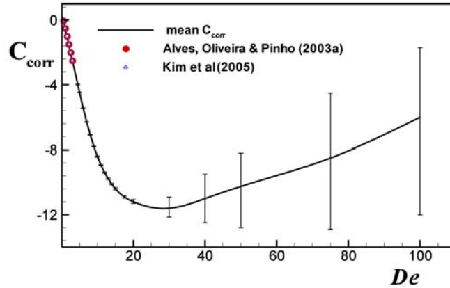
Figure 5.42: Time average Couette correction ( C_{corr} ) as function of Deborah number obtained with mesh M3C. Error bars represent the amplitude of the oscillations.
