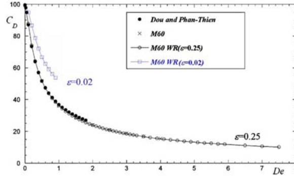
Figure 5.27: Drag force coefficient for a PTT fluid with \beta=0 . Mesh M60 WR (-○- or squares); Mesh M60 (x); and Dou and Phan-Thien (2003) data (filled circles).
