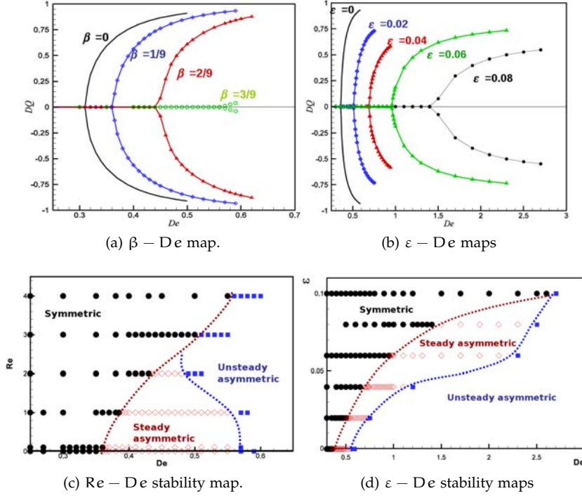
Figure 3.3: \beta - Re - De and \varepsilon - Re - De maps of flow pattern types (Poole et al., 2007a).
