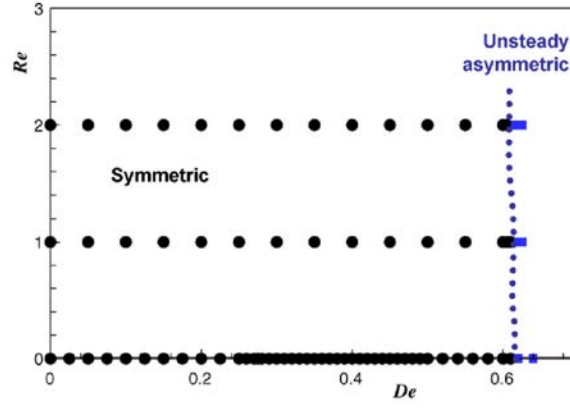
Figure 6.4: Re-De stability map for the biaxial extension flow configuration ( I_o = 2 : 4 ).
