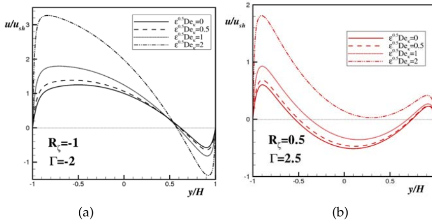
Figure 7.19: Dimensionless velocity profiles for a PTT fluid under the mixed influence of electro-osmotic/pressure driving force as function of \sqrt{\epsilon}De_{\kappa} for relative microchannel ratio of \bar{\kappa} = 20 : (a) \Gamma = -2 and R_{\zeta} = -1 and (b) \Gamma = 2.5 and R_{\zeta} = 0.5 .
