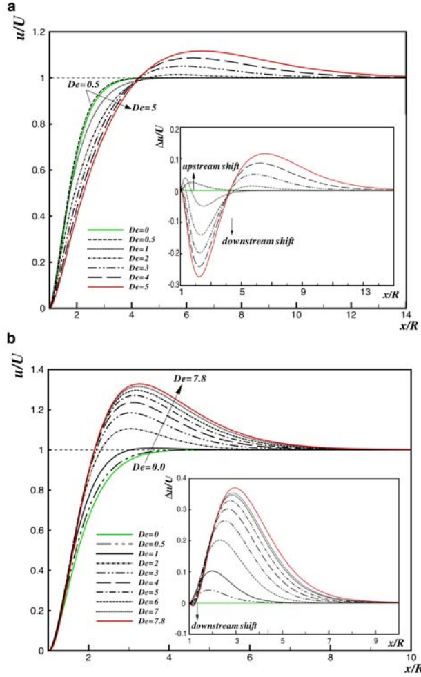
Figure 5.26: u centreline profiles for FENE-CR with (a) L^2 = 10 and (b) L^2 = 100 . The inset shows the wake velocity difference, \Delta u/U = (u - u_{\text{Newt}})/U .
