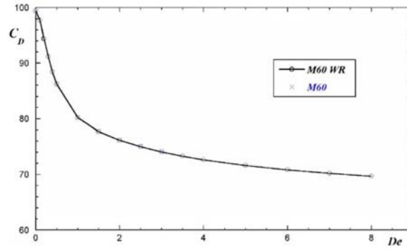
Figure 5.30: Drag force coefficient for a Giesekus fluid ( \alpha=0.02 and \beta=0.59 ). Mesh M60 WR (-○-); Mesh M60 (×).
