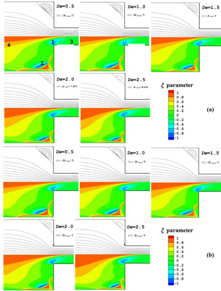
Figure 5.36: Flow patterns (top half) and maps of flow-type parameter (bottom half) as predicted on mesh M_3 (Oldroyd-B model). (a) StrT ; (b) LogT . (The values of \det(\mathbf{A})_{\min} are indicated beside each map).
