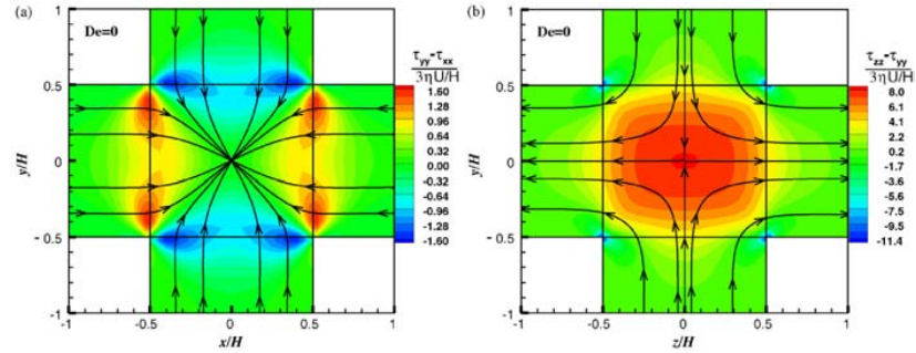
Figure 6.5: Flow patterns and contour plots of normal-stress differences for Newtonian flow for I_o = 4 : 2 at centre planes (a) xy and (b) yz .
