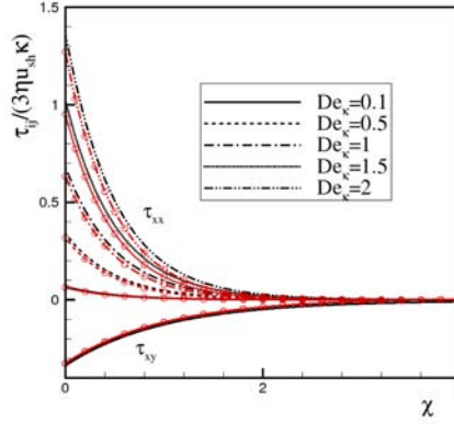
Figure 7.7: Dimensionless normal and shear stresses profiles for viscoelastic fluid under the mixed influence of electro-osmotic/pressure driving force as function of \sqrt{\varepsilon}De_\kappa for \bar{\kappa} = 100 , \Gamma = -1 (lines) and \Gamma = 2.5 (lines with symbols).
