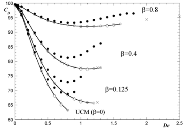
Figure 5.19: Drag force coefficient for UCM and Oldroyd-B fluids. Mesh M60 ( \times ); Mesh M60 WR (-o-); Mesh M120 WR (empty diamonds) and Dou and Phan-Thien (2003) data (filled circles).
