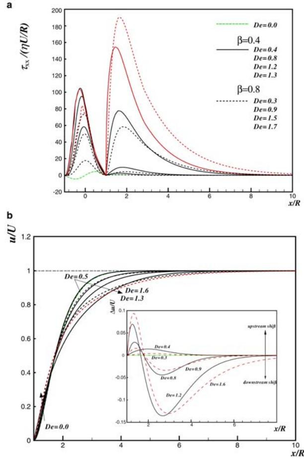
Figure 5.23: (a) \tau_{xx} and (b) u centreline profiles for Oldroyd-B fluid with \beta=0.4 and \beta=0.8 . The inset shows the wake velocity difference, \Delta u/U = (u - u_{\text{Newt}})/U .
