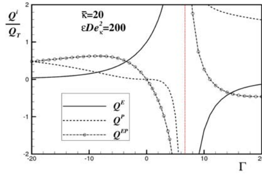
Figure 7.11: Relative contribution to the flow rate for electro-osmotic flow of a PTT fluid for relative microchannel ratios of \bar{\kappa} = 20 at large \epsilon De_{\kappa}^2 (= 200) as a function of \Gamma .
