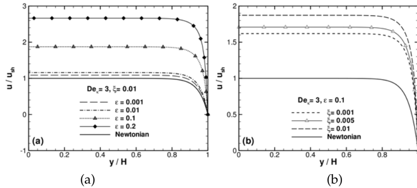
Figure 7.23: Effect of (a) variation of \epsilon at De_\kappa = 3 and \xi = 0.01 and (b) variation of \xi at De_\kappa = 3 and \epsilon = 0.1 on the non-dimensional velocity profiles for the viscoelastic fluid flow in the microchannel under the influence of electro-osmotic forces. In all cases \bar{\kappa} = 20 .
