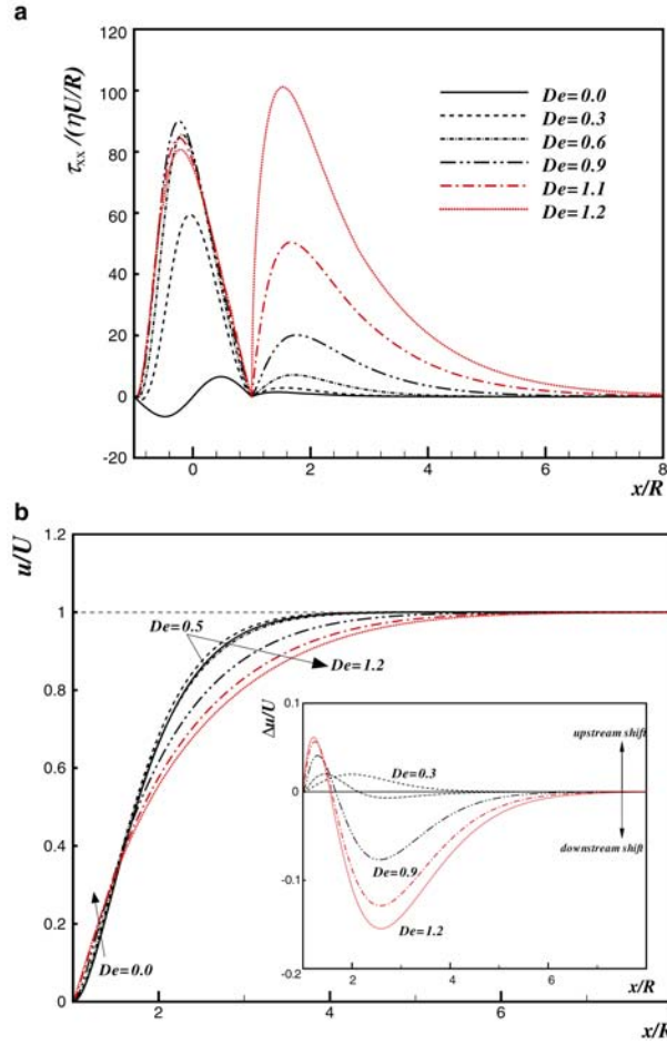
Figure 5.22: (a) \tau_{xx} and (b) u centreline profiles for Oldroyd-B fluid with \beta = 0.125 . The inset shows the wake velocity difference, \Delta u/U = (u - u_{\text{Newt}})/U .
