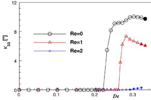
Figure 6.7: Variation of main direction angle \kappa_{33} with Deborah number at the center of the cross-slot for uniaxial extension flow ( I_o = 4 : 2 ). Full symbols represent unsteady simulations.
