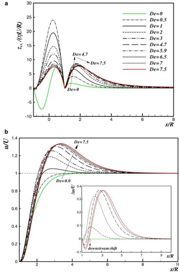
Figure 5.28: (a) \tau_{xx} and (b) u centreline profiles for the PTT model ( \epsilon=0.25 ). The inset shows the wake velocity difference, \Delta u/U = (u - u_{N_{ewt}})/U .
