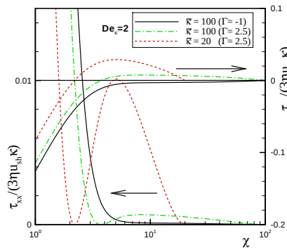
Figure 7.8: Dimensionless normal and shear stresses profiles for viscoelastic fluid under the mixed influence of electro-osmotic/pressure driving force at De_\kappa = 2 as function of the near wall variable, for \bar{\kappa} = 100 ( \Gamma = -1 and \Gamma = 2.5 ) and \bar{\kappa} = 20 ( \Gamma = 2.5 ).
