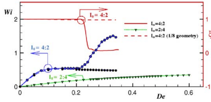
Figure 6.9: Variation with De of the local Weissenberg number ( Wi ) and flow type parameter ( \xi ) at the stagnation point for the biaxial ( I_0 = 2 : 4 ) and uniaxial ( I_0 = 4 : 2 ) extensional flow configurations. Values for the symmetry-imposed flow also included for the uniaxial configuration.
