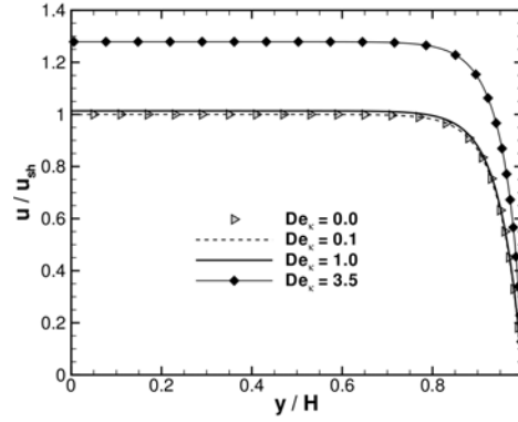
Figure 7.22: Effect of De_\kappa ( \epsilon, \xi = 0.01, \bar{\kappa} = 20 ) on the non-dimensional velocity profiles for the viscoelastic fluid flow in the microchannel under the influence of electro-osmotic forces.
