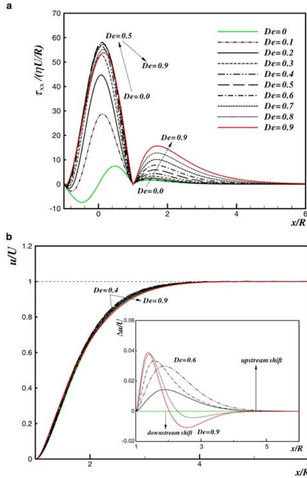
Figure 5.29: (a) \tau_{xx} and (b) u centreline profiles for the PTT model ( \epsilon=0.02 ). The inset shows the wake velocity difference, \Delta u/U = (u - u_{Newt})/U .
