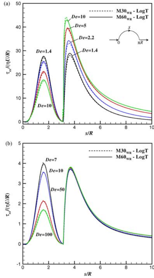
Figure 5.13: Stress profiles along cylinder wall and downstream centreline for PTT fluid with meshes M30_{WR} and M60_{WR} at (a) De = 1.4, 2.2, 5 and 10 with \varepsilon = 0.02 ; (b) De = 7, 10, 50 and 100 with \varepsilon = 0.25 .
