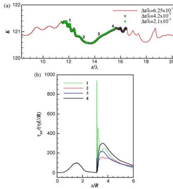
Figure 5.9: Creeping flow of an Oldroyd-B fluid ( \beta = 0.59 ) past a cylinder at De = 1.2 (Mesh M30 WR ). (a) Time evolution of the drag force coefficient for different time steps, \Delta t/\lambda . (b) Axial normal stress profiles along cylinder wall and downstream centreline at the four instants marked in (a).
