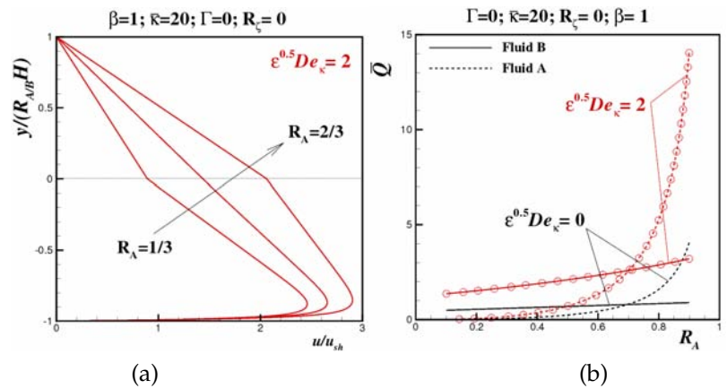
Figure 7.36: Effect of the nonconducting fluid holdup on dimensionless (a) velocity profiles ( R_\Lambda = 1/3, 1/2 and 2/3 ) and (b) volumetric flow rate for Newtonian-Viscoelastic flow configuration.
