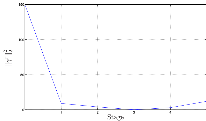
Figure 7.3: \|\gamma^r\|_2^2 for each stage.
