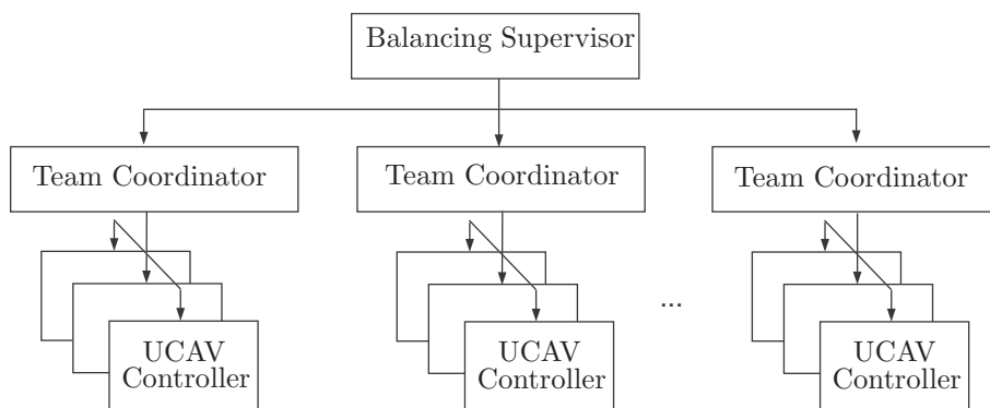
Figure 6.1: Control hierarchy.
