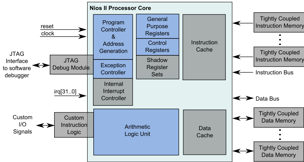
Figure 2.2: Simplified block diagram of Nios II soft-core processor
