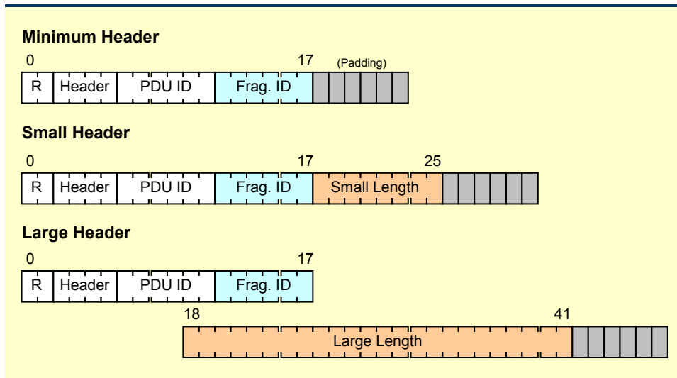
Figure 8.12: REMPLI Fragmentation Headers for Unicast Data Services
