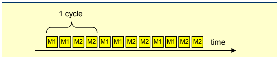
Figure 3.1: DLC1000 Network Layer time division
