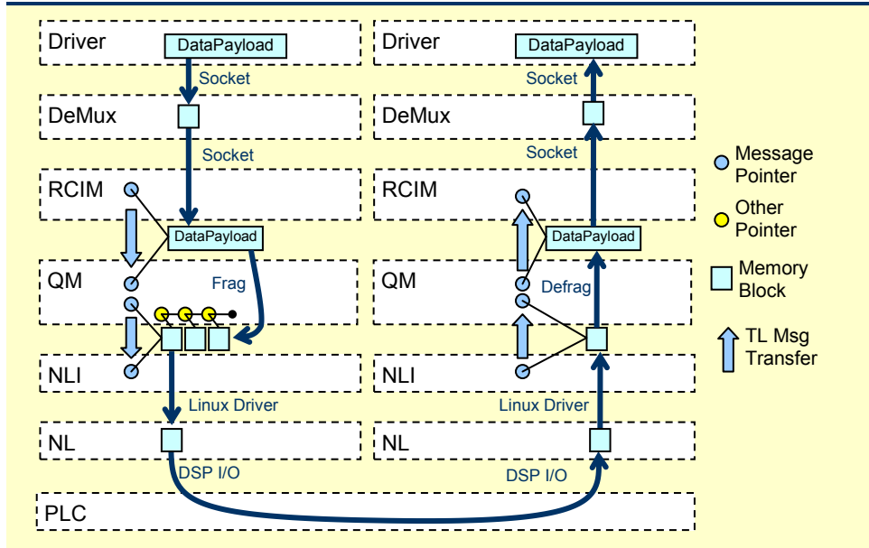
Figure 8.13: Memory Blocks in a Unicast service (Linux HyNet System)
