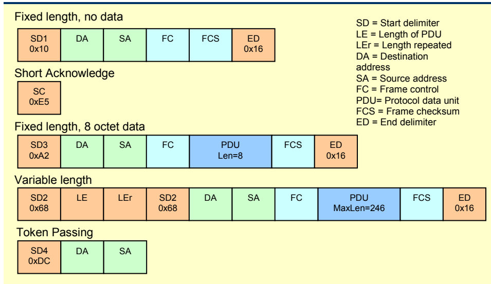
Figure 2.4: Profibus most used frame formats
