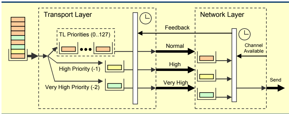
Figure 7.6: REMPLI priority queues processing
