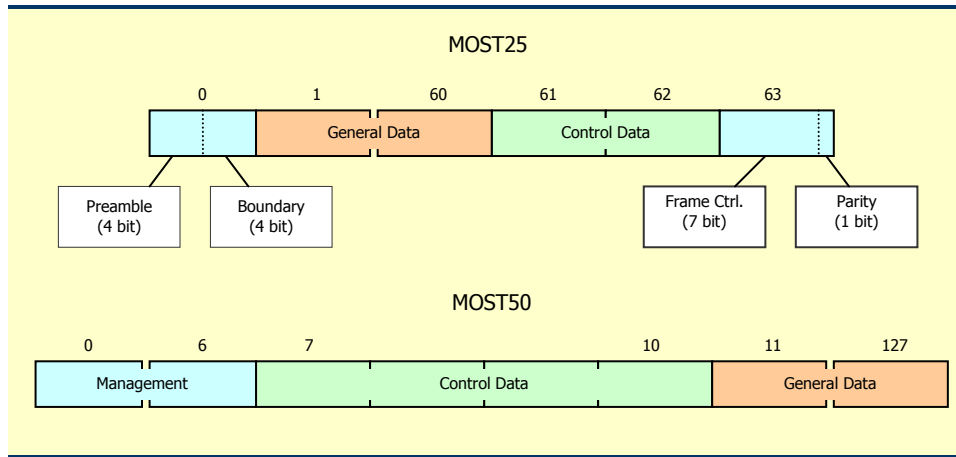
Figure 2.10: MOST Frame Structure
