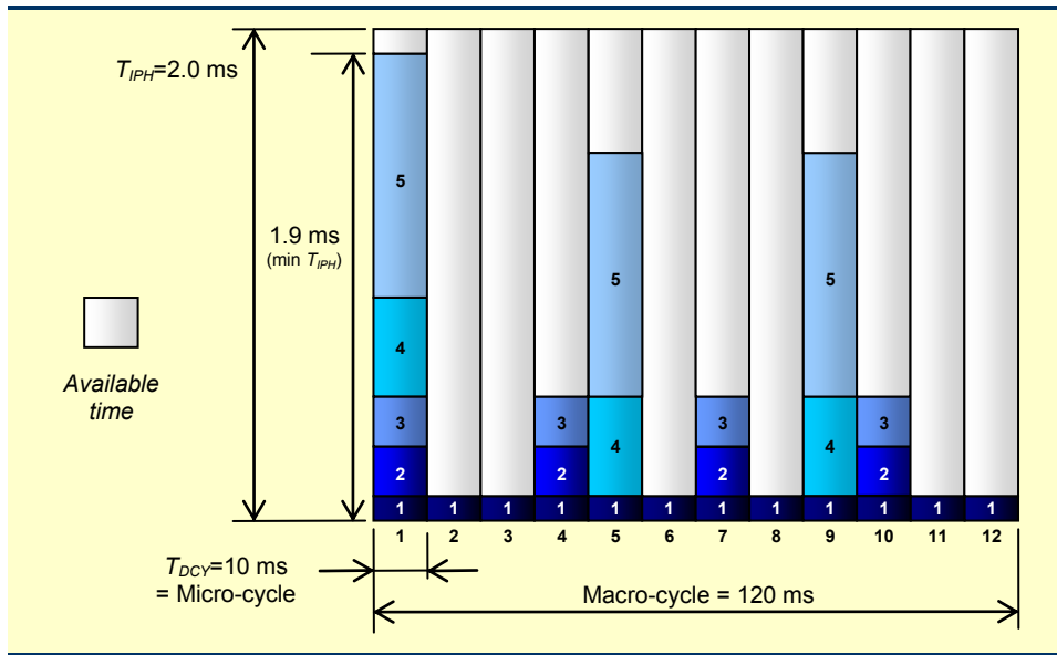
Figure 4.7: Scheduling example at IP ACS level
