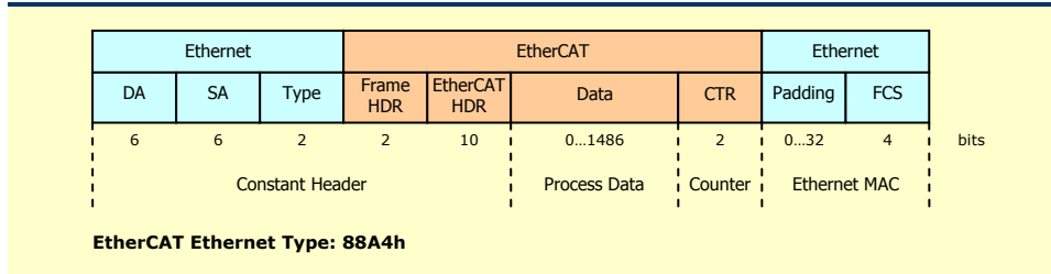
Figure 2.9: EtherCAT Ethernet PDU
