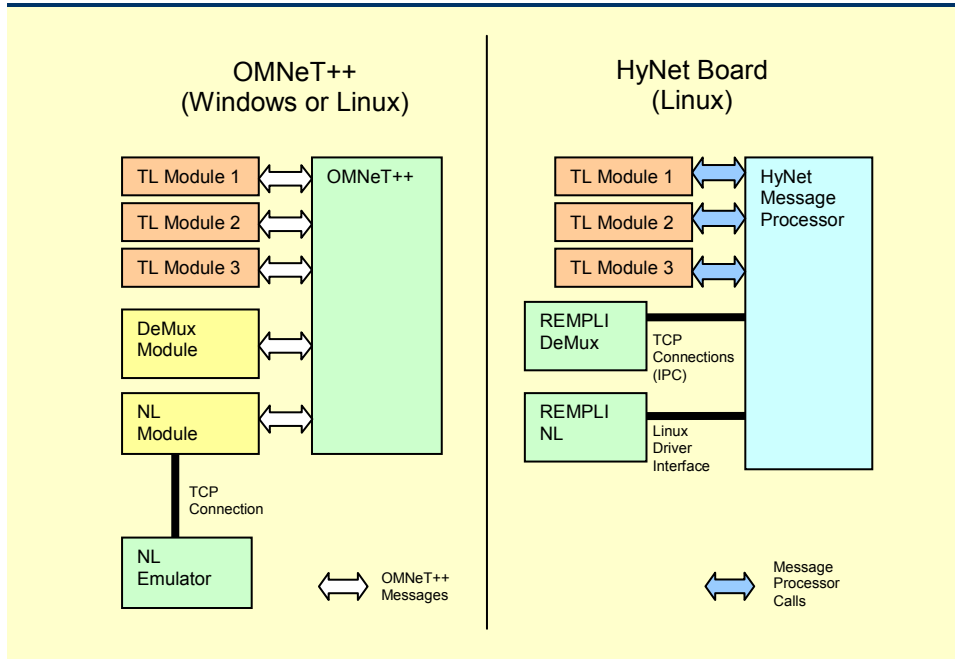
Figure 8.2: OMNeT++ simulation and HyNet implementation
