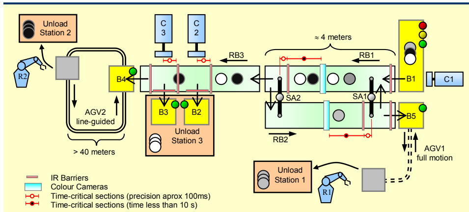
Figure 6.1: Manufacturing field trial mechanical system layout
