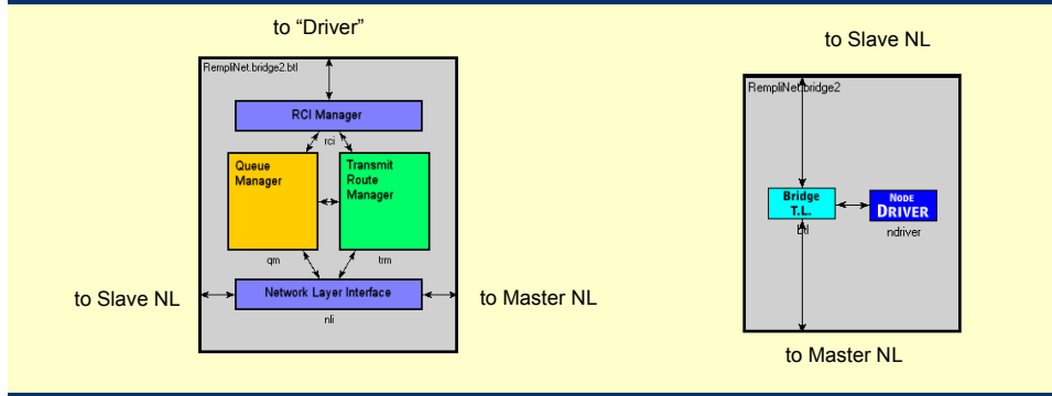
Figure 8.5: OMNeT++ Simulation “Bridge” and “TL” modules
