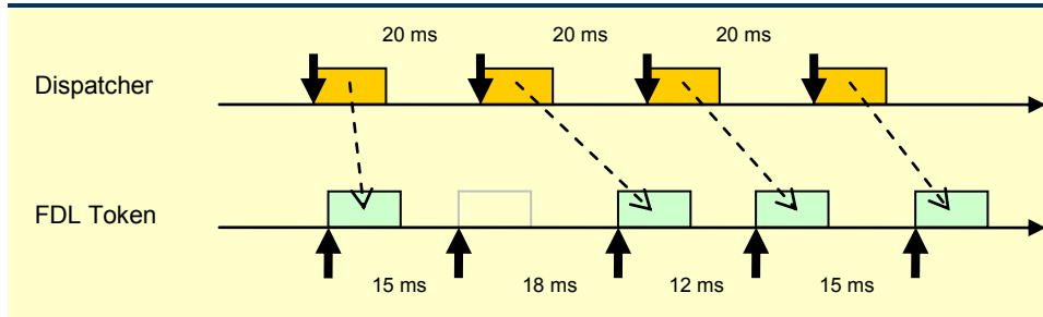
Figure 4.11: Dispatcher and token timing
