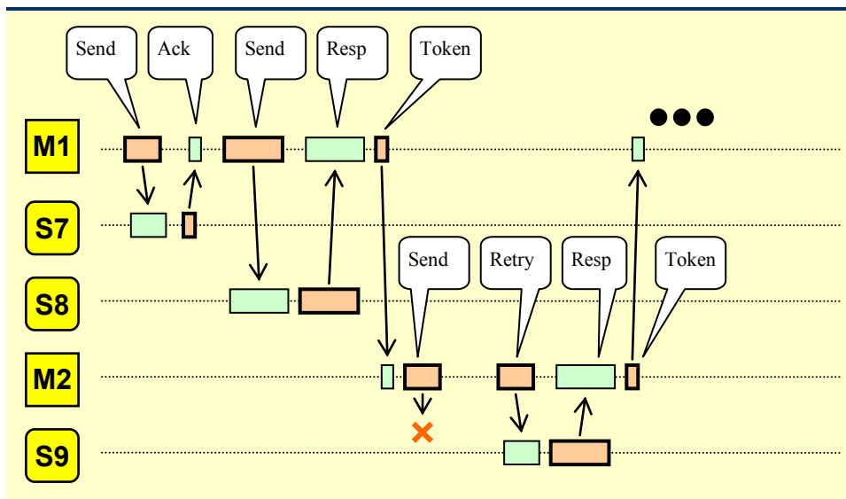
Figure 2.2: Example Profibus data exchange
