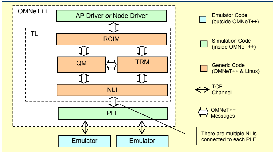
Figure 9.2: Transport Layer Simulator Architecture
