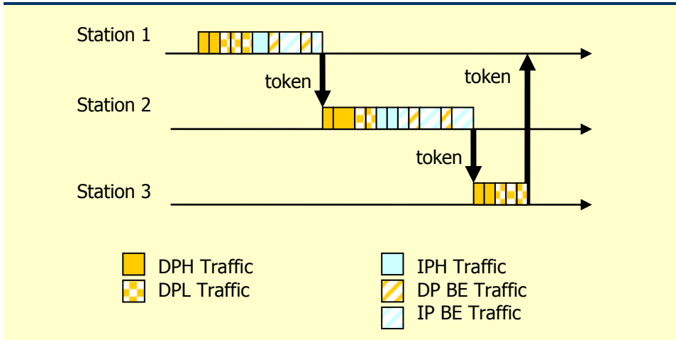
Figure 4.10: Dispatcher traffic classes and timing concepts
