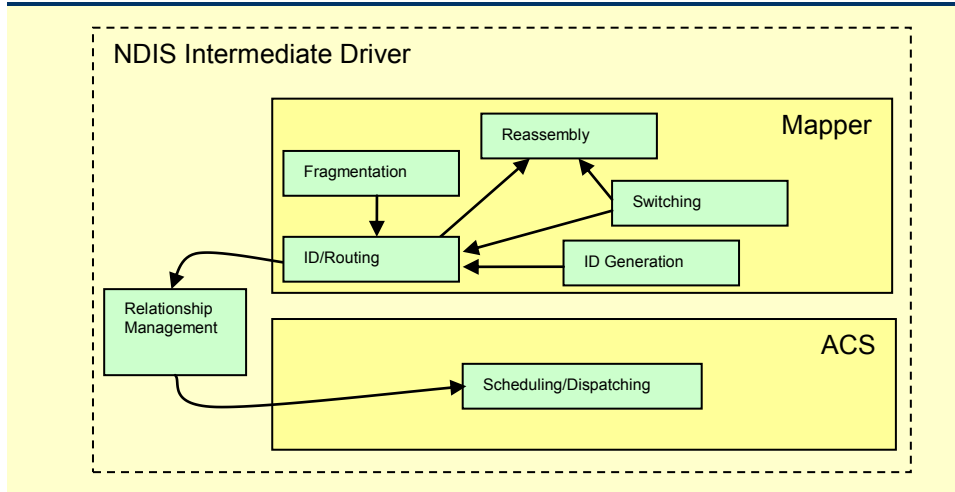
Figure 5.10: RFieldbus NDIS intermediate driver functionality
