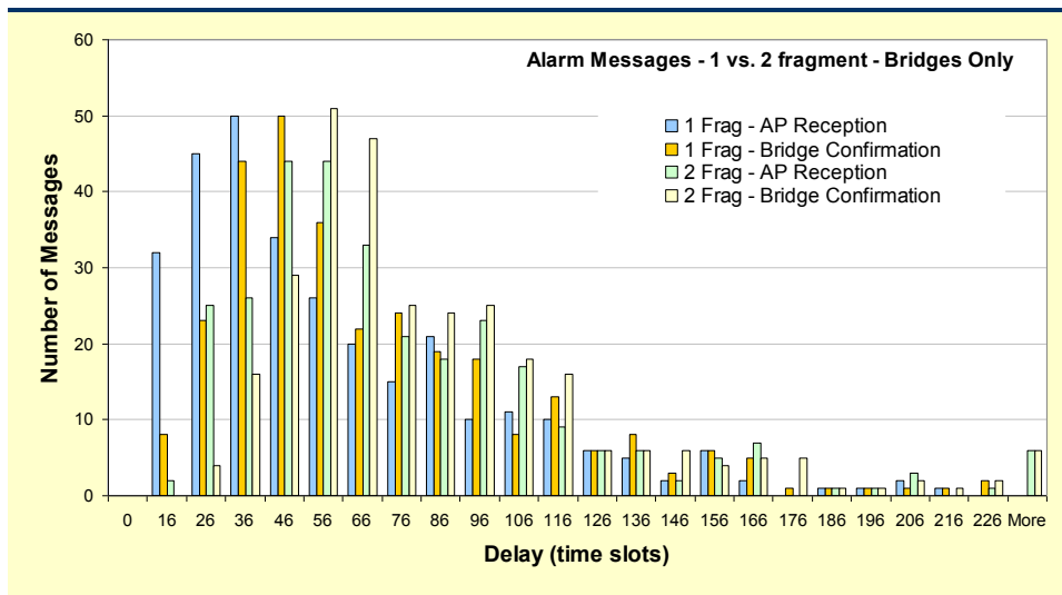
Figure 9.10: Alarm Service, 1 vs. 2 Fragments, Bridges 201 and 202
