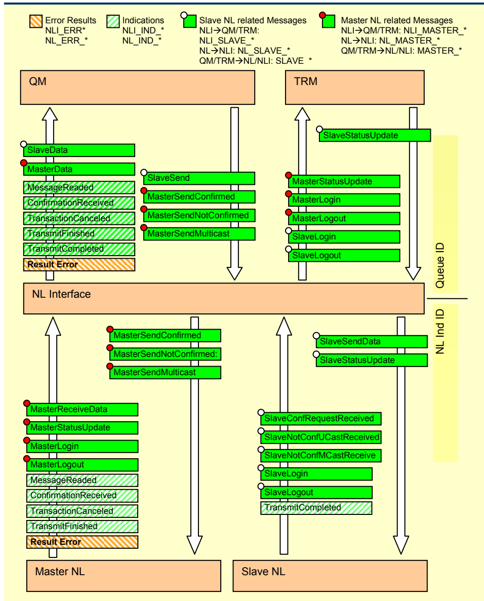
Figure 8.8: REMPLI NLI messages
