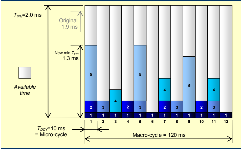
Figure 5.2: IP ACS Deferred-Release scheduling example
