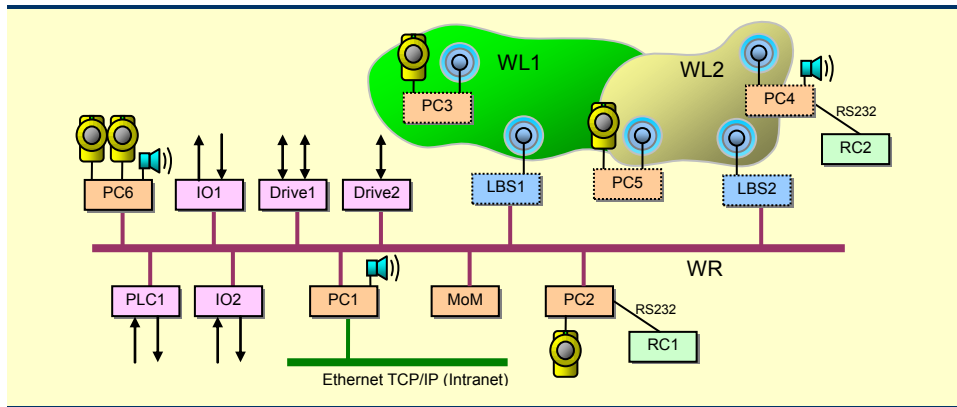
Figure 6.2: Manufacturing field trial network topology
