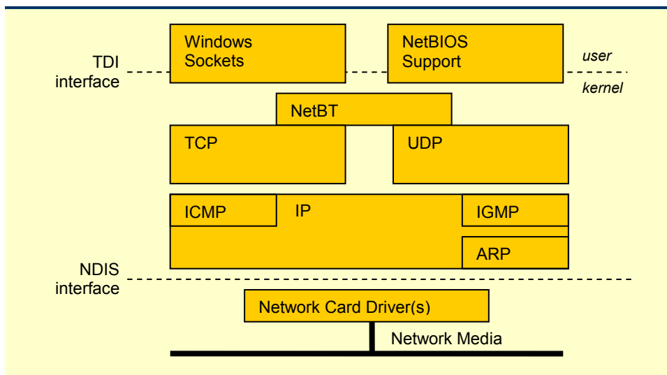
Figure 5.6: Windows NT TCP/IP network model overview
