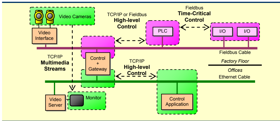
Figure 1.1: Example of a System TCP/IP services coexisting with fieldbus services
