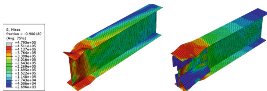
Fig. 3 Buckling behavior of a bare steel beam and a CFRP reinforced beam (Unit kPa)
