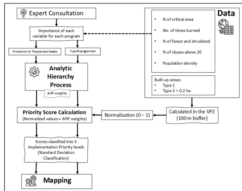
Figure 2. Methodological workflow for the spatial prioritization of villages according to wildfire mitigation objectives.
