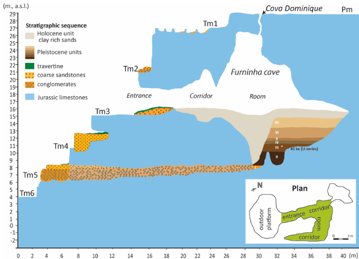
Fig. 7. Schematic representation of the marine terrace staircase and cave-karst system of the Furninha site (see Fig. 6 for cave location). Pm = culminant wave cut surface); Tm (1–6) = wave-cut platforms and associated marine deposits (the Pleistocene unit comprises a lower marine conglomerate (I) and upper layers of aeolian sands (II to VII); the Holocene unit comprises clay-rich sands). In the late 19th century, the Pleistocene and Holocene units were completely excavated (Delgado, 1884).
