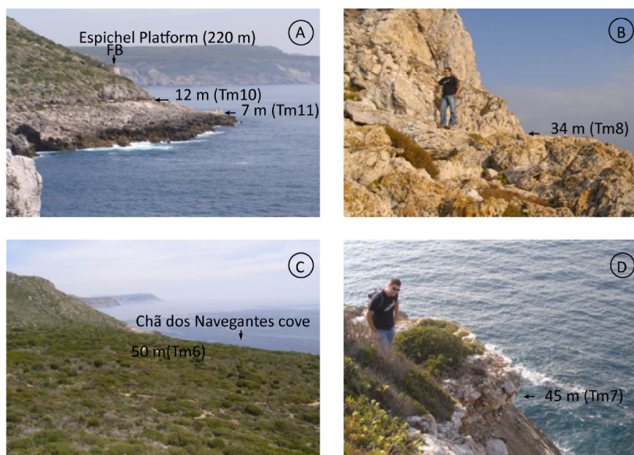
Fig. 6. A – Forte da Baralha ruins (FB) and the shoreline angles (a.s.l.) of the Tm10 (12 m) and Tm11 (7 m); B – paleo-shoreline angle of the Tm8 terrace (34 m); C – the Chã dos Navegantes cove; D – rolled limestone boulders of the Tm7 terrace (45 m).
