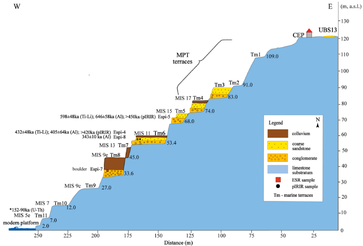
Fig. 11. Schematic cross section of the terrace staircase at Cape Espichel promontory. MPT - Middle Pleistocene Transition.
