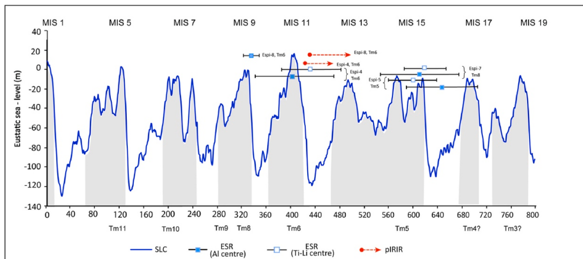
Fig. 10. Age results derived from pIRIR (minimum) and ESR methods in the Cape Espichel promontory. Eustatic sea level curve data from Spratt and Lisiecki (2016).
