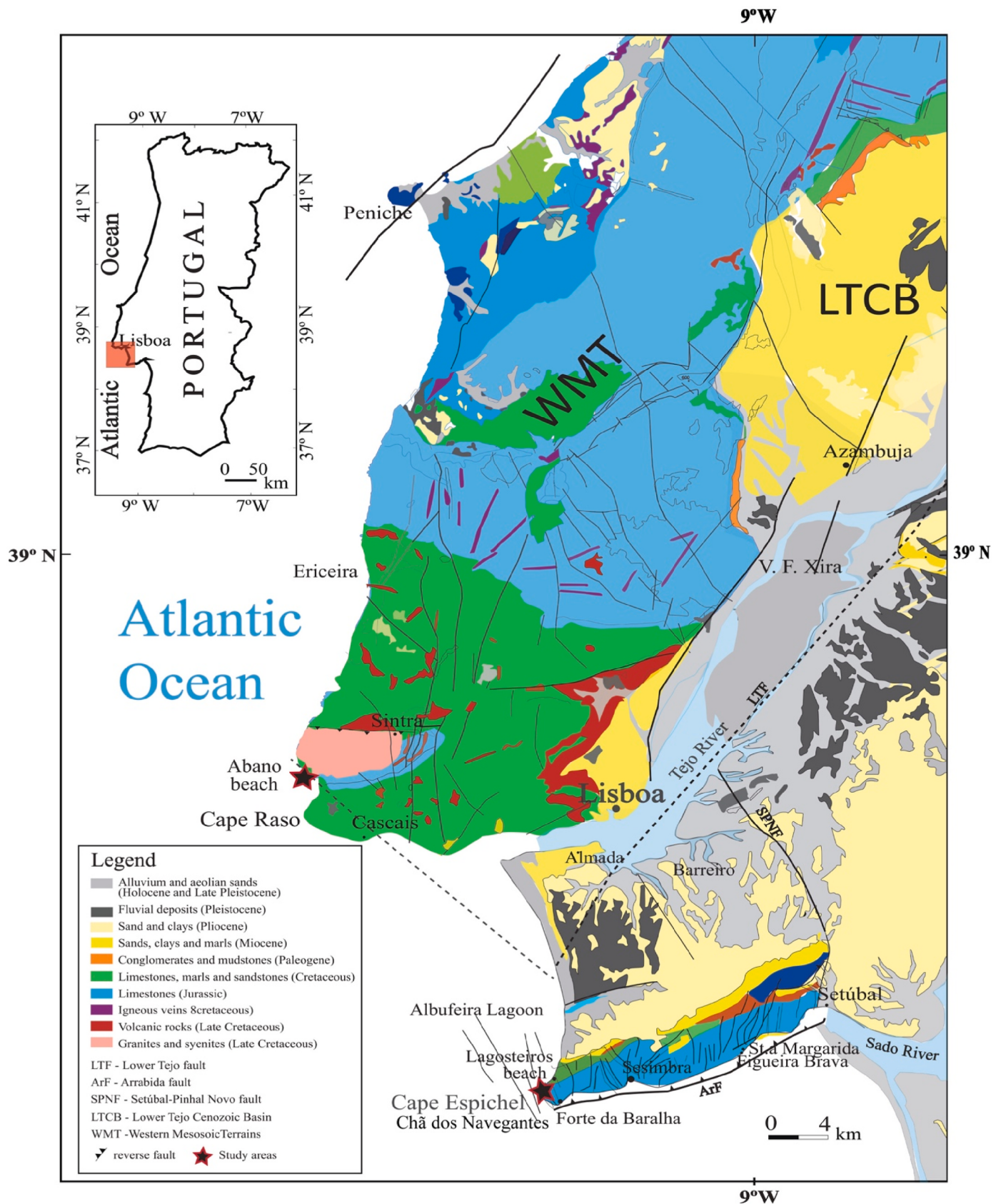
Fig. 2. Geological setting of the study area (based on the 1/500,000 geological map, LNEG).
