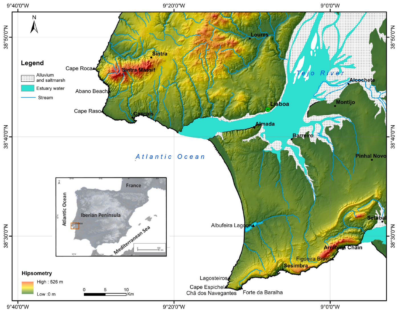
Fig. 1. Study area location map depicting the Cape Raso - Abano beach area and the Cape Espichel.
