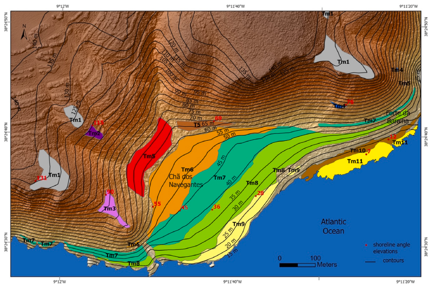
Fig. 5. Geomorphological map of the Chã dos Navegantes and Forte da Baralha sectors. Eleven emerged marine terraces and one submerged terrace (at -7 m) were recognized. The Tm10 (12 m) has a sedimentary record, but most of the shore platforms have insufficient sediment thickness for numerical dating. Red numbers represent shoreline angle elevations. (For interpretation of the references to colour in this figure legend, the reader is referred to the Web version of this article.)
