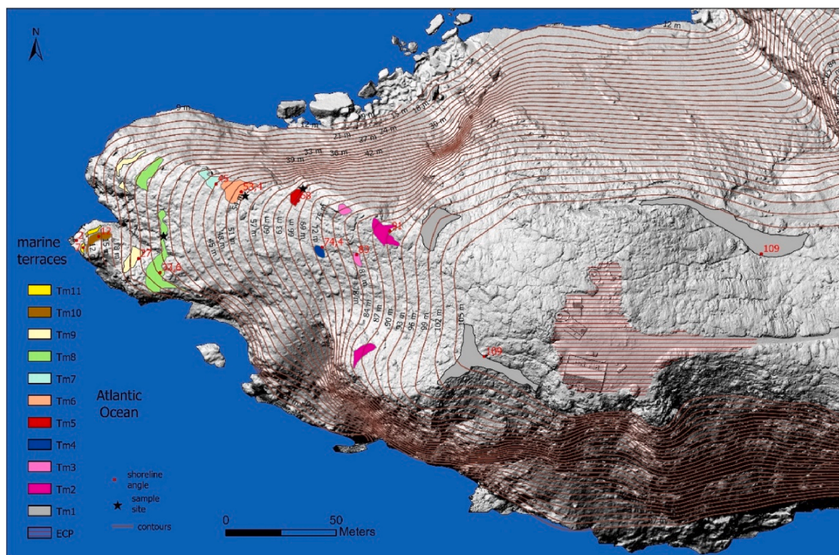
Fig. 4. The terraces staircase at the western promontory of Cape Espichel. Eleven emerged marine terraces were recognized. Some terraces, without geomorphological expression, were identified by the sedimentary record on the steep slope of the headland. Red numbers indicate the shoreline angle elevations. (For interpretation of the references to colour in this figure legend, the reader is referred to the Web version of this article.)
