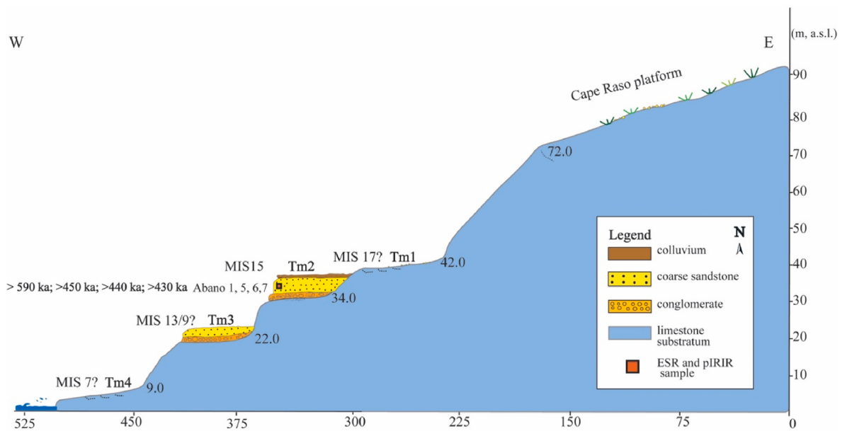
Fig. 9. – Schematic cross profile of the terrace staircase at the Cape Raso - Abano beach area.
