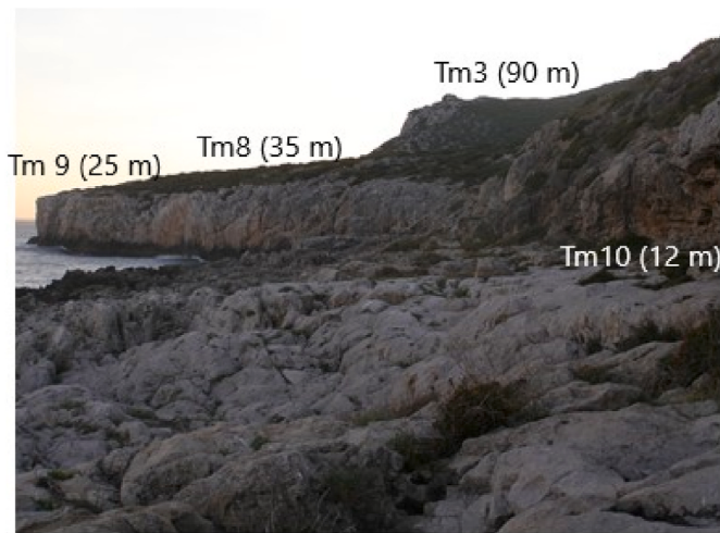
Fig. 7. Panoramic view taken from the shore platforms of the Tm10 at Forte da Baralha to the Chã dos Navegantes. Several marine platforms can be distinguished: the Tm10 (12 m), Tm9 (25 m); Tm8 (35 m) and Tm3 (90 m).
