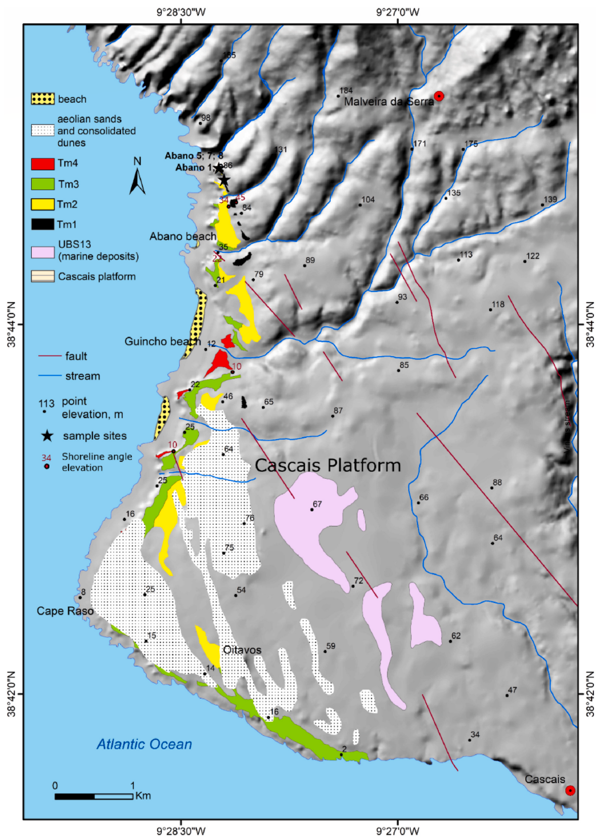
Fig. 3. Map of Cape Raso - Abano beach area, showing the Cascais Platform and the mapped marine terraces. The aeolian sand cover around Oitavos, is also shown. Shoreline angle elevations are red numbers. (For interpretation of the references to colour in this figure legend, the reader is referred to the Web version of this article.)
