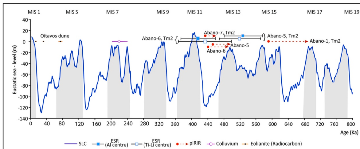
Fig. 8. Ages given by the samples measured by pIRIR (minimum) and ESR methods, collected from the sands of the Tm2 terrace in the Abano beach (Cape Raso area). Eustatic sea level curve data from Spratt and Lisiecki (2016).
