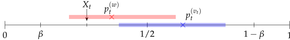
Figure 4.4 In Case 2, every time X_t falls on the left of \mathcal{I}_{q,t}^{(v_t)} (in blue), an honest node might also like a transaction w if the upper boundary of \mathcal{I}_{q,t}^{(w)} (in red) is also on the right of X_t .
