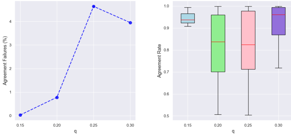
Figure 4.8 Agreement failures (in percentage) and agreement rate of a double spend \mathbb{T} = \{u, v\} where malicious nodes reply with the same opinion to a query from every node.
