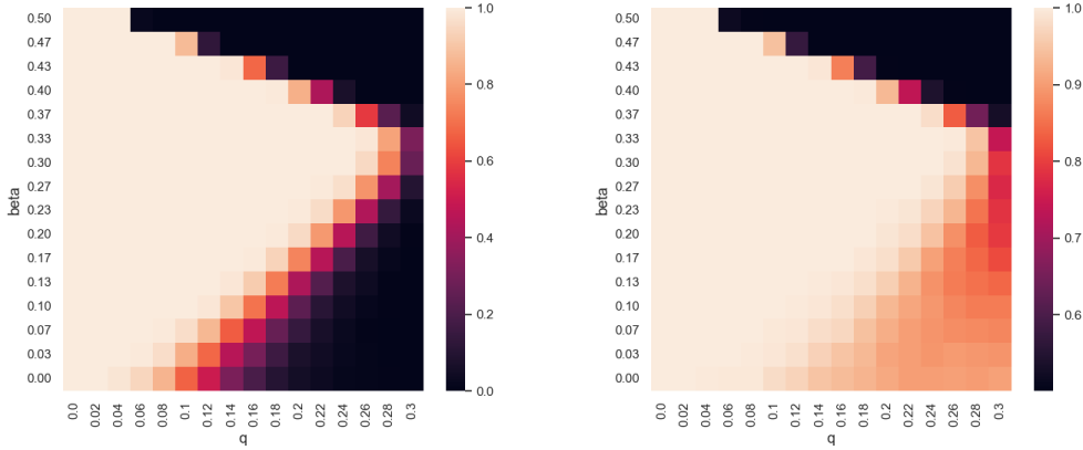
Figure 4.7 Finalization and agreement rate for different values of q and \beta .
