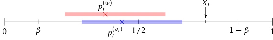
Figure 4.3 In Case 1, every time X_t falls on the right of \mathcal{I}_{q,t}^{(v_t)} (in blue), an honest node is likely to assign 0 to the auxiliary opinion of every transaction.
