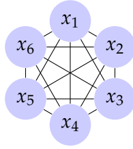
Figure 3.3 Graph representation of a set with 6 transactions where all of them are in conflict with each other.
