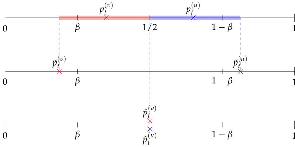
Figure 5.1 The interval of control (in blue) of a transaction u \in \mathbb{T}_t with p_t^{(u)} = 1/(2(1-q)) and of a transaction v \in N(u) . Notice that the sum of the intervals covers the whole support of X_t .
