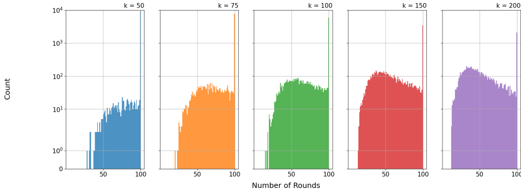
Figure 4.6 Effects of k on the performance of the protocol. Logarithmic scale.
