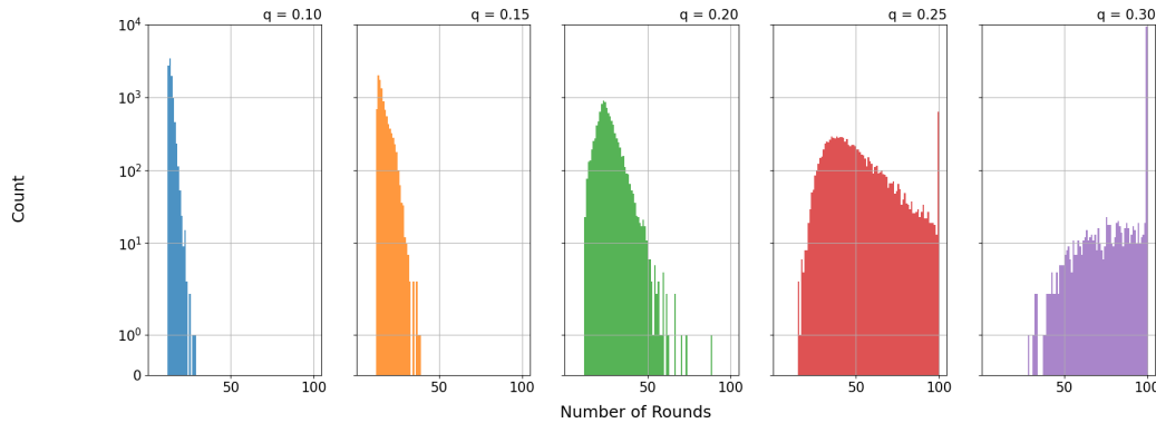
Figure 4.5 Effects of q on the performance of the protocol. Logarithmic scale.
