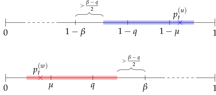
Figure 3.4 The intervals of control \mathcal{I}_{q,t}^{(u)} for a transaction u which has a proportion of likes among honest nodes p_t^{(u)} > 1 - \mu (in blue), and \mathcal{I}_{q,t}^{(w)} for a transaction w such that p_t^{(w)} < \mu (in red). Notice that these intervals are separated from the support [\beta, 1 - \beta] of X_t .
