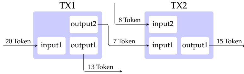
Figure 3.1 Diagram representing the general structure of two transactions.
