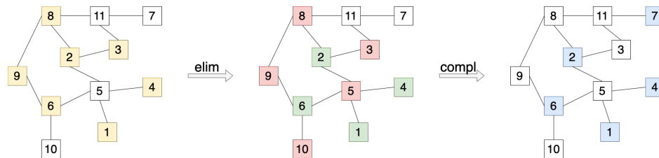
Figure 3.5 Representation of step (vi) of the protocol. The graph represents the node's vision at time t . The numbers represent the order according to the hash function. In the first subfigure, the transactions in yellow represent the set B ; in the second subfigure, transactions in green represent B' and transactions in red represent N(B', A_t^{(n)}) ; in the last subfigure, transactions in blue represent B'' , the chosen maximal independent set of the round.
