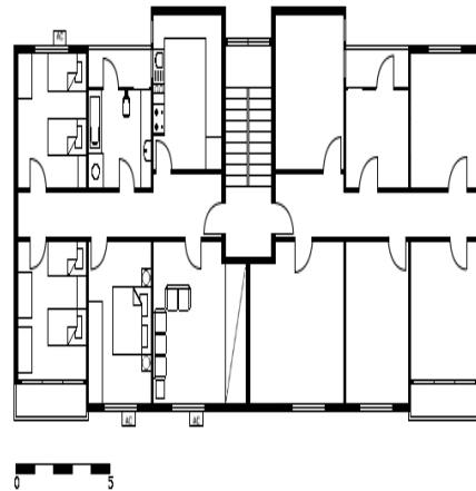
Figure 2. Typical floor plan [19].
