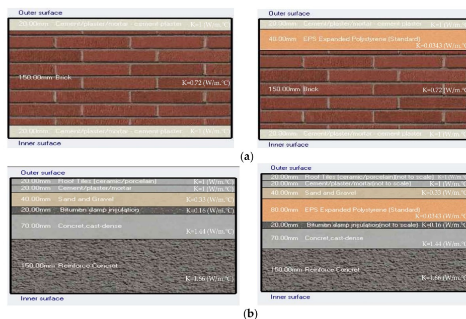
Figure 8. Construction materials layers for opaque surfaces: (a) exterior walls, (b) roof.
