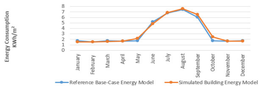
Figure 4. Building Energy Model Calibration.
