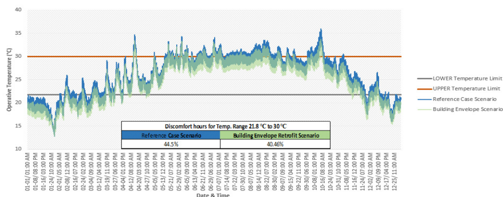
Figure 10. EREC Thermal Comfort Analysis—Thermal Comfort Zone between 21.8 °C to 30 °C (all year—8760 h).
