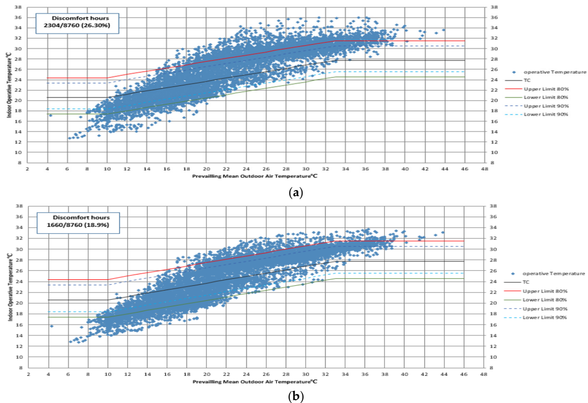
Figure 11. ASHRAE-55 adaptive thermal comfort analysis, based on 8760 h for (a) acceptable operative temperature (“Reference-Case”) and (b) acceptable operative temperature (“Building Envelope Retrofit-Case”).
