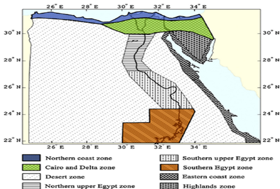
Figure 1. Egypt's climatic zones classification map, according to EREC [13].
