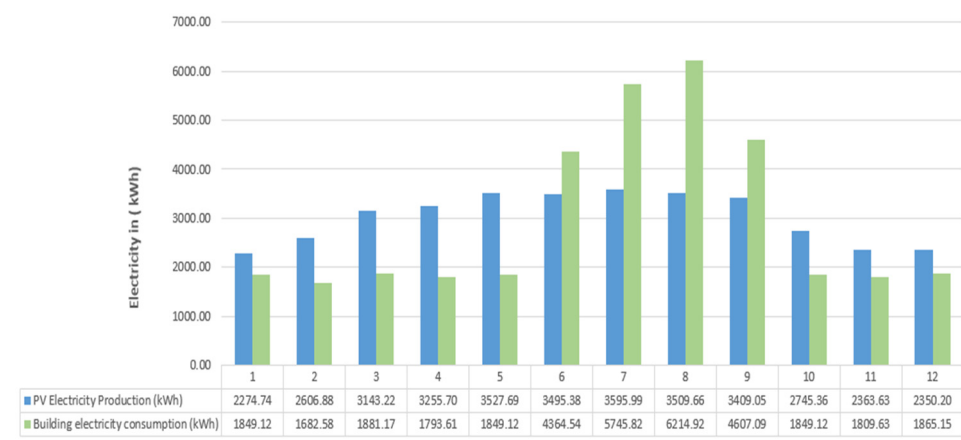
Figure 9. PV Electricity Production vs. Building Electricity Consumption.
