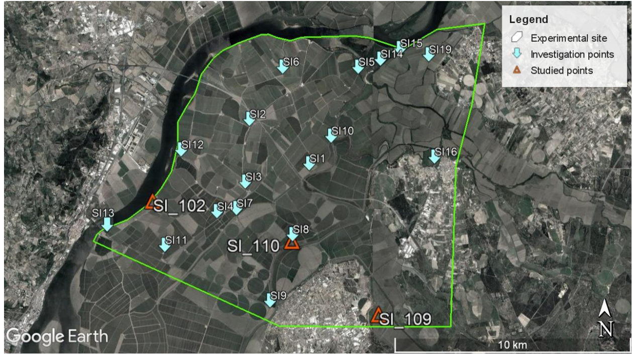
Figure 1. Map of the experimental site and location of the investigation points (after [10]).
