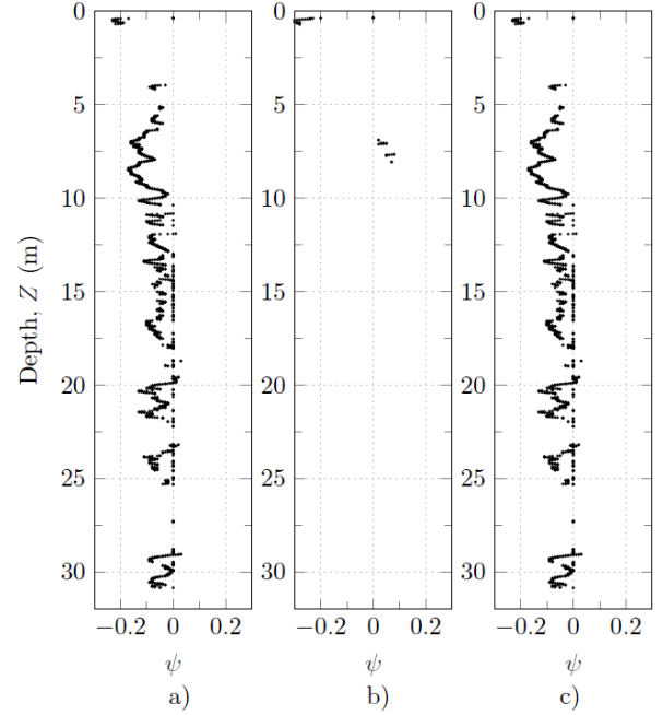
Figure 4. Soil state parameter profiles for the layers with I_c < 2.60 : a) SI102; b) SI109; c) SI110.
