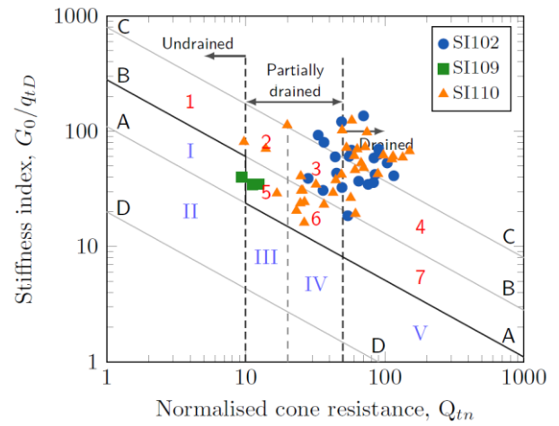
Figure 8. Soil classification in terms of drainage conditions of the soils with I_c < 2.60 after drained cone resistance correction.
