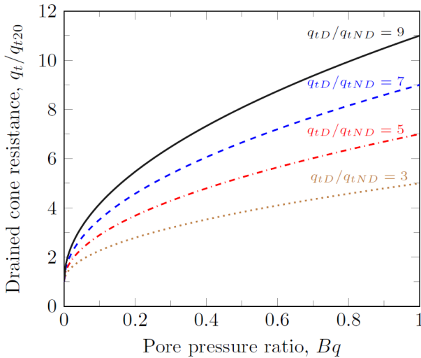
Figure 7. Drained cone resistance correction chart.
