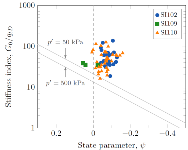
Figure 9. Results of the theoretical correlation between G_0/q_{tD} and \psi .
