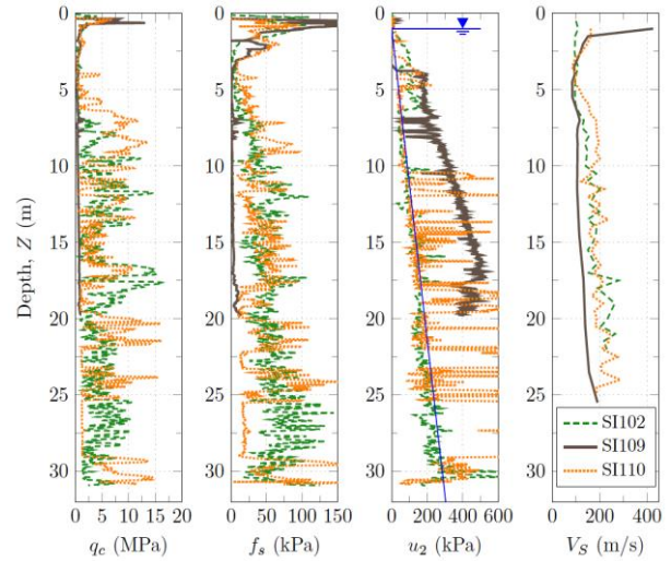
Figure 2. SCPTu results.
