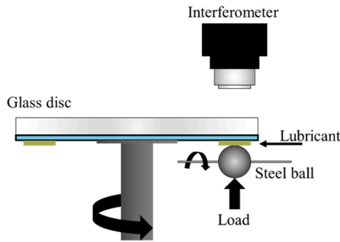
Fig. 2. Diagram of the EHD2 Ultra-Thin Measurement apparatus (PCS Instruments).
