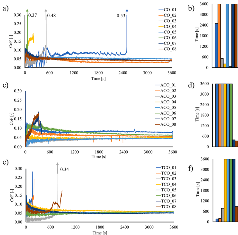
Fig. 9. Friction profile versus time and test duration for: (a, b) CO, (c, d) ACO and (e, f) TCO.
