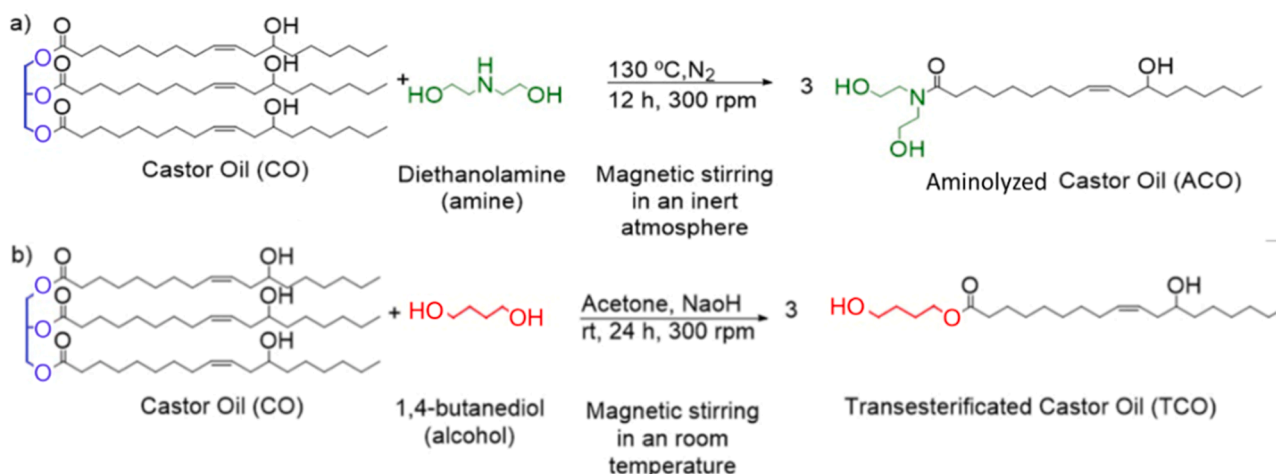
Fig. 1. Schematic of (a) aminolysis, and (b) transesterification process applied to castor oil base.
