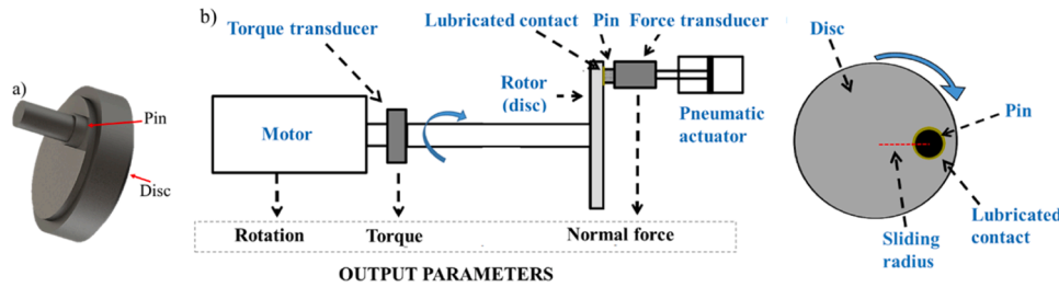
Fig. 4. Pin-on-disc setup: (a) representation of the specimens and (b) simplified diagram of the equipment.
