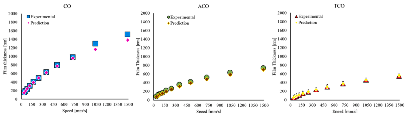
Fig. 6. Film thickness experimental measurement versus predictions ( h_{c,T} calculated) for each biolubricant in the SRR = 1 condition.
