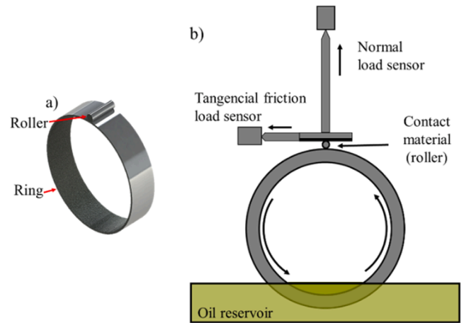
Fig. 3. Block on ring apparatus: (a) representation of the specimens and (b) simplified schematic of the equipment.
