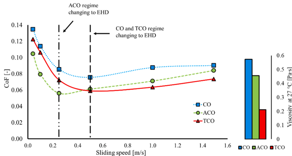
Fig. 7. Stribeck curves measured in the BoR test and viscosity in the right side.
