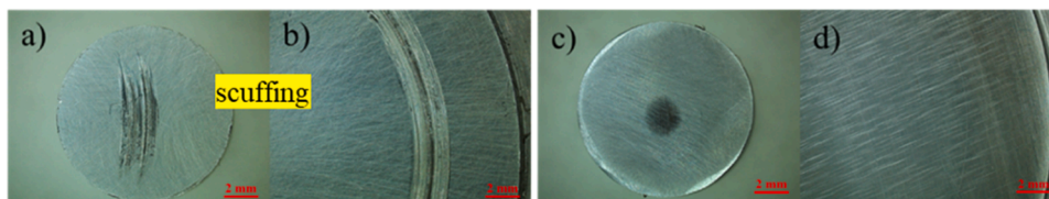
Fig. 8. Examples of contact materials showing (a,b) scuffing and (c,d) abrasion.
