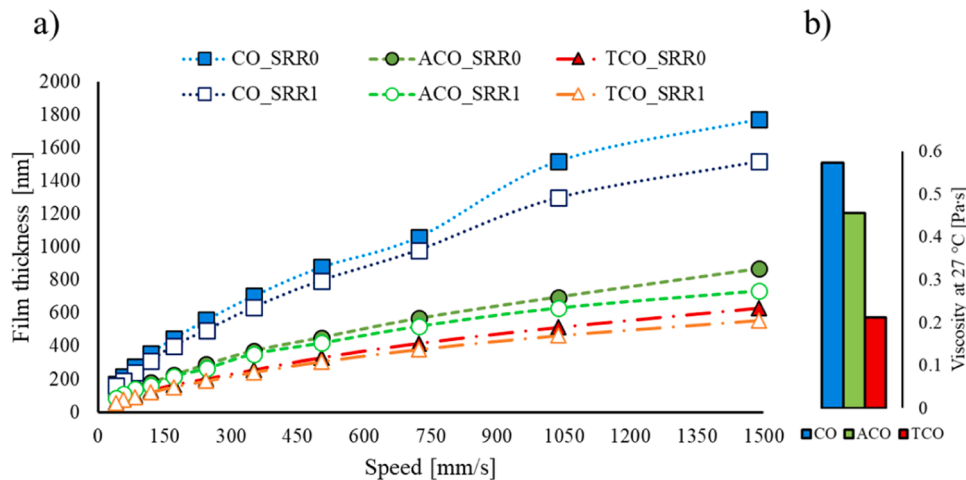
Fig. 5. Results and comparison of the average film thickness measurement tests for SRR = 0 (pure rolling) and SRR = 1 (sliding and rolling); (b) dynamic viscosity at 27 °C.
