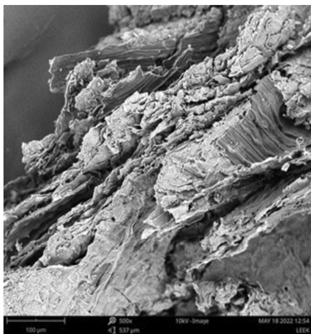
Fig. 3 SEM characterization of the LCMNFs contained in the LCB pulp prepared at HC and 6 passes with a magnification of 500×
