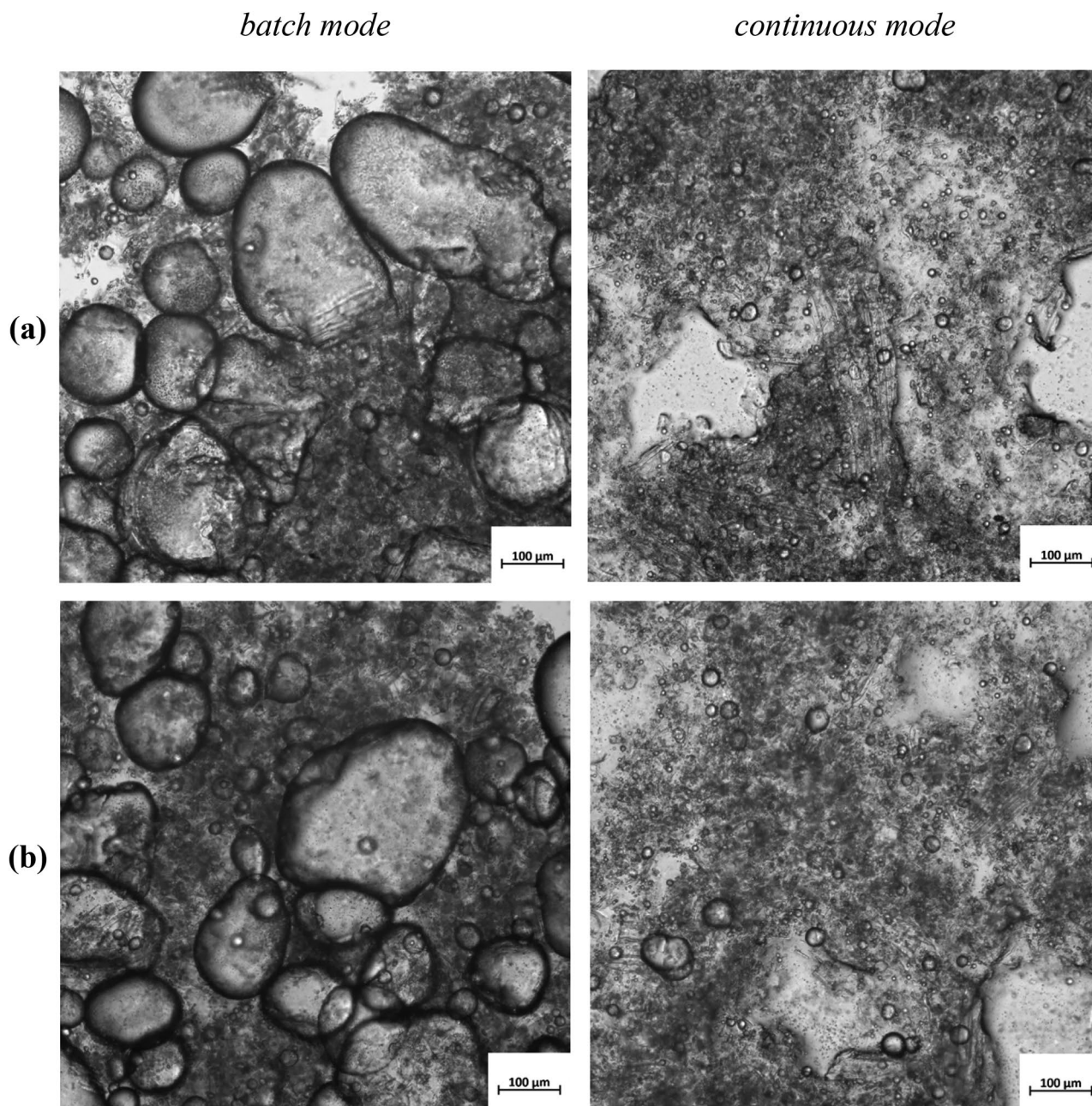
Fig. 8 OM images (10X magnification) 48 h after production in batch and continuous mode for formulations a O/W 30/70 wt.%, LCB 4.2* wt.%; b O/W 40/60 wt.%, LCB 3.6* wt.%
