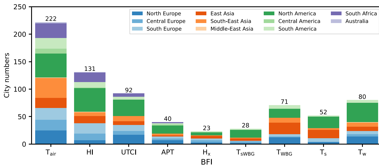
Fig. 3. The BFI [including air temperature ( T_{\text{air}} ) and HSIs] in modeling/predicting daily human mortality for 739 MCC cities. a) The indicator with the minimum qAIC when fitting to the human mortality (defined as BFI). The color of the BFI is presented based on their sensitivity to the humidity (Fig. S1, e.g. T_{\text{air}} (zero sensitivity to humidity), T_{\text{w}} (maximum sensitivity to humidity)). The number in the bracket represents the rank in the sensitivity to humidity of the HSI. b) The number of cities and their locations under each BFI group. The results are based on the daily mean value of the indicators.
