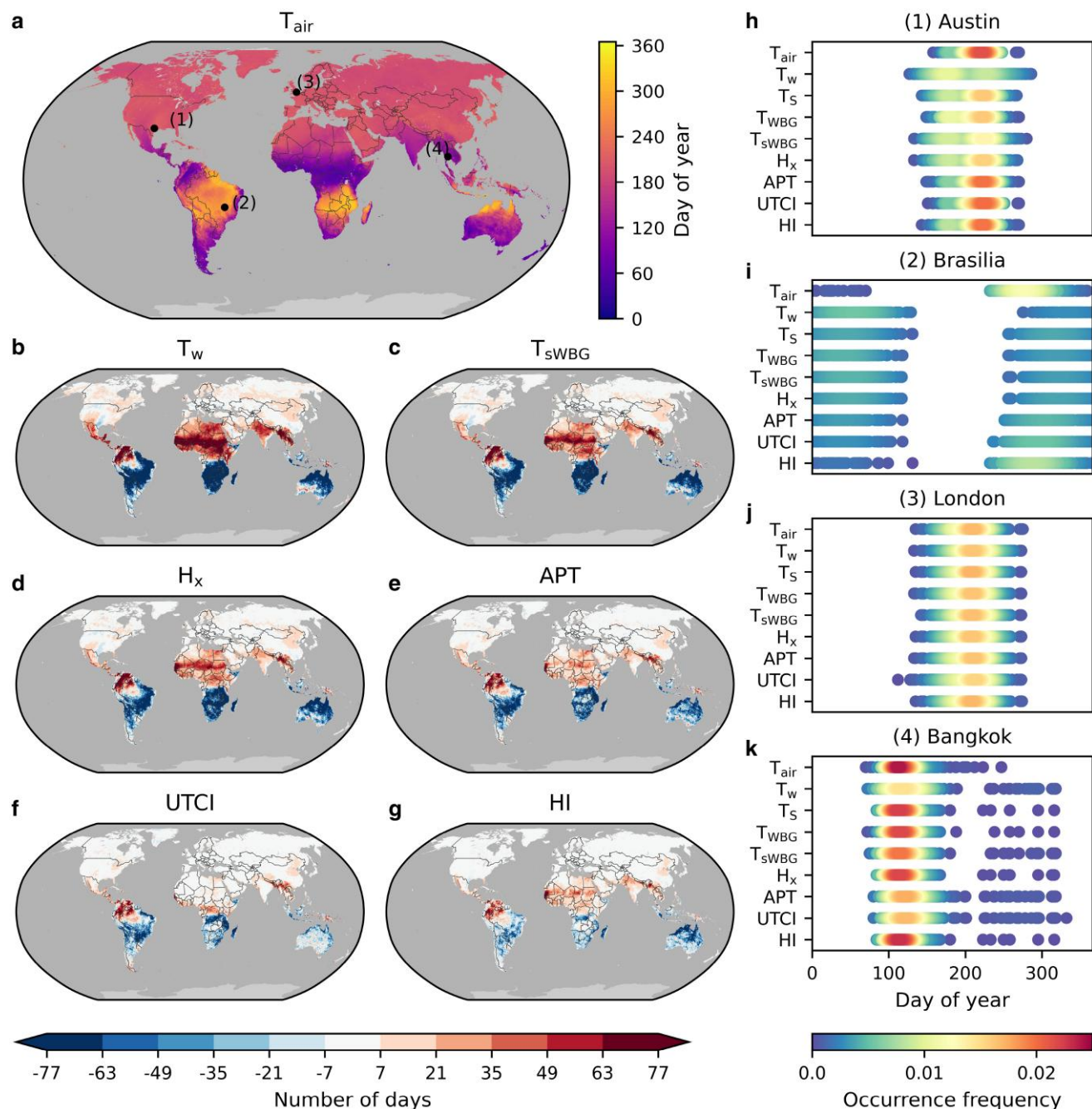
Fig. 2. Intra-annual PT difference among air temperature ( T_{air} ) and HSIs. a) Averaged intra-annual PT of T_{air} (day of year when T_{air} reaches annual peak) for 1980–2019. b–g) Difference between averaged intra-annual PT of corresponding HSI and T_{air} (the former minus the latter) for 1980–2019. h–k) Occurrence frequency of the hottest 10 days measured by T_{air} and 8 HSIs for 4 cities: Austin (h), Brasilia (i), London (j), and Bangkok (k) for 1980–2019. The occurrence frequency is obtained by Gaussian kernel density estimation.
