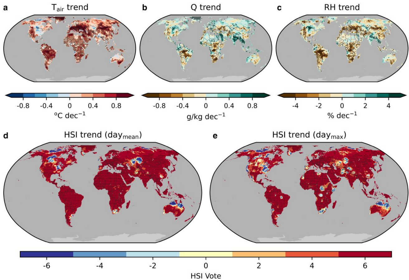
Fig. 1. Long-term trends of the extremes of six HSIs. a–c) The linear trends (per decade) of the T_{air} X99 (99 th percentile of the annual values of each year) (a), and specific humidity (Q) (b) and RH (c) of the high-temperature days (daily T_{air} > T_{air} X99) between 1980 and 2019. The results of a–c are based on the daily mean value. Stippling denotes the linear trend reaches the significant level ( P < 0.05 ). d, e) The sum of the HSI vote of T_w , T_{sWBG} , H_x , APT, UTCI, and HI. The HSI vote is set as 1 when HSI X99 shows a positive trend between 1980 and 2019 and is set as –1 when negative. Results based both on the daily mean (d) and daily maximum (e) values of HSIs are presented. Stippling denotes the linear trend of at least one HSI reaching the significant level ( P < 0.05 ).
