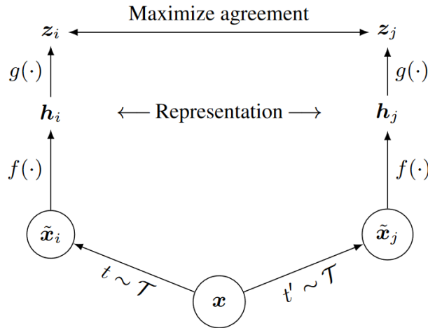
Figure 4.2: Diagram representation of the SimCLR method. Two data augmentations create correlated views of each data example. The encoder and projection head maximize agreement between these views using contrastive loss. Post-training, the projection head is discarded, and the encoder is used for downstream tasks. Source: [69]
