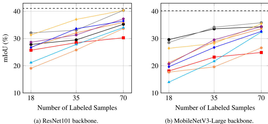
Figure 6.5: mIoU (%) comparison between the methods for KITTI using DeepLabv3 model.
