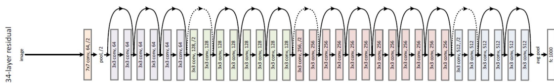
Figure 2.5: ResNet architecture. The dotted shortcuts increase dimensions. Source: [13]
