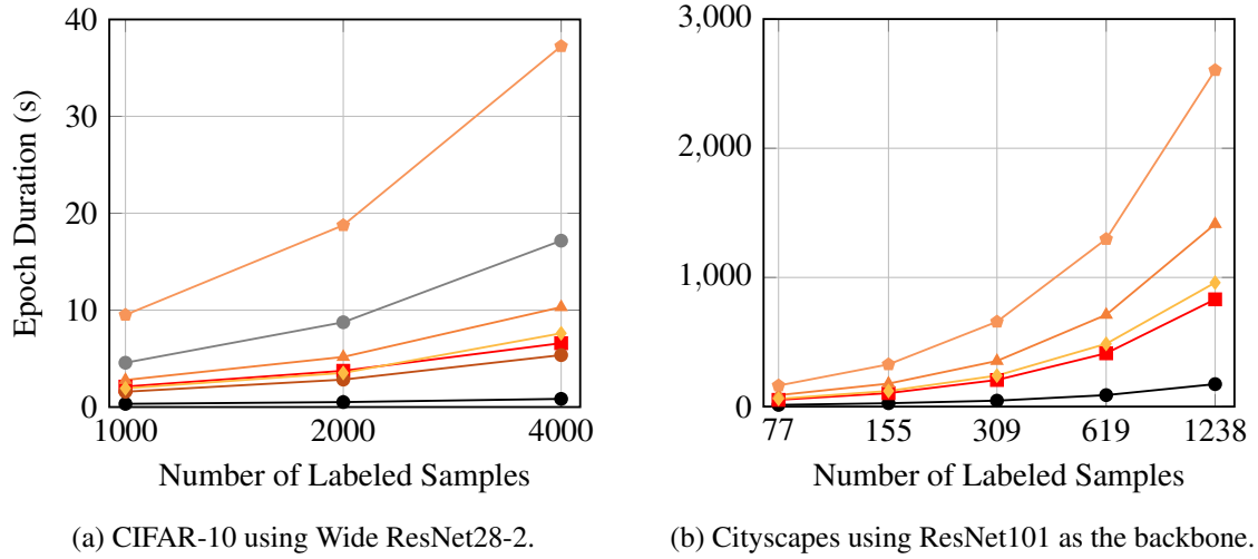
Figure 6.6: Mean epoch duration (s) comparison between the methods.
