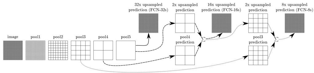
Figure 2.7: Fully Convolutional Network architecture. Source: [14]
