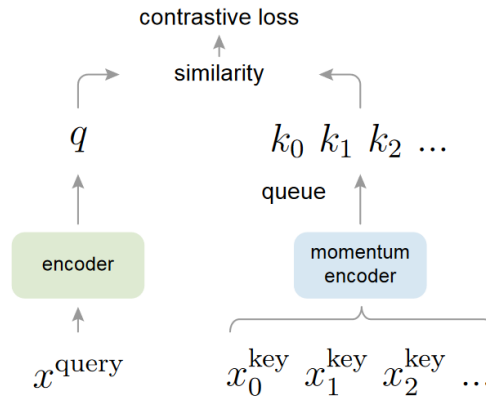
Figure 4.4: Diagram representation of the MoCo method. Source: [70]
