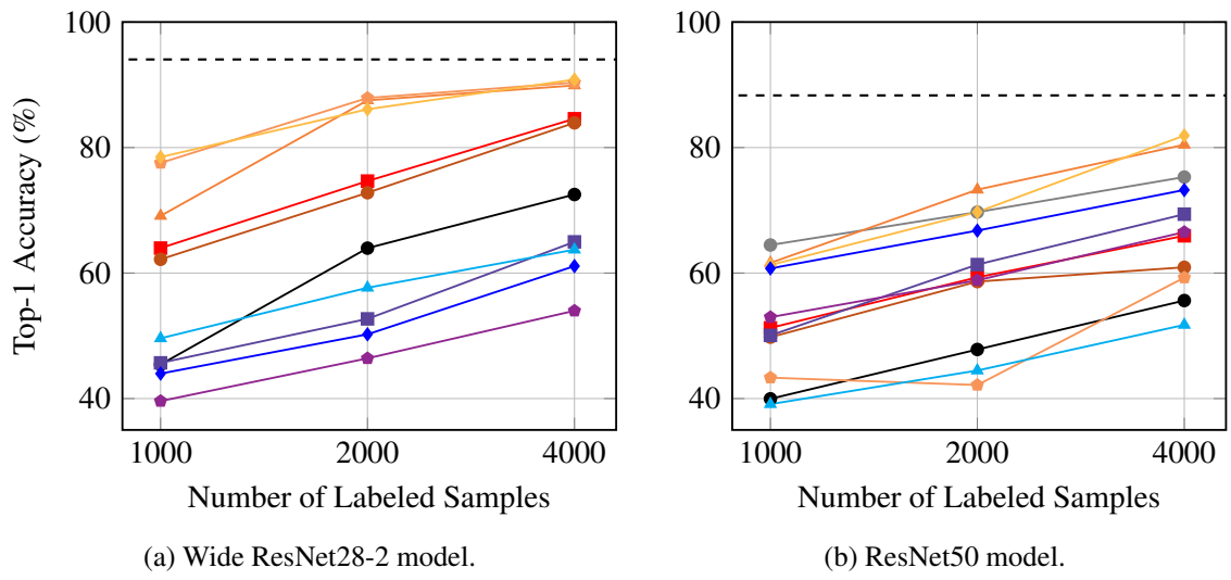
Figure 6.2: Top-1 Accuracy comparison between the methods for CIFAR-10.
