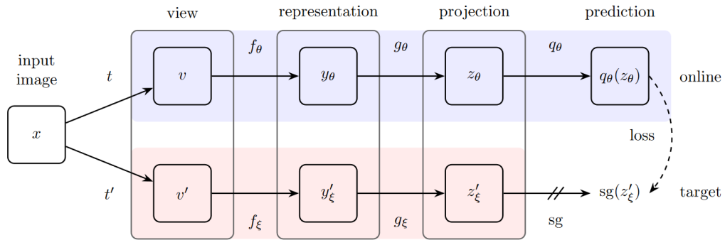
Figure 4.3: Diagram representation of the BYOL's architecture. Source: [72]
