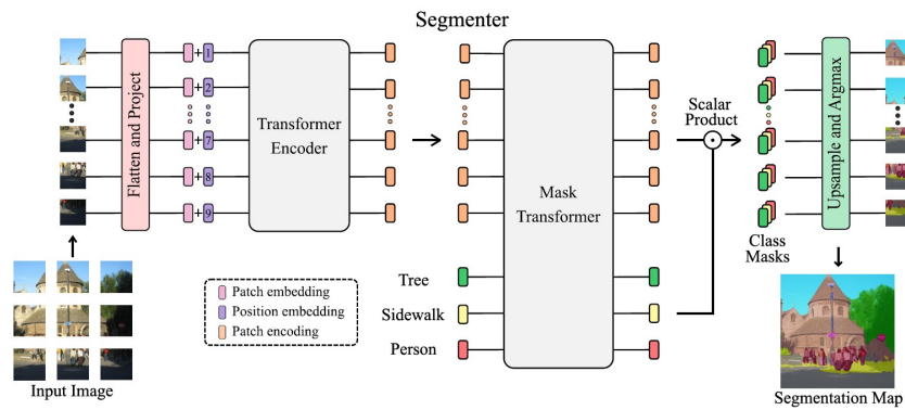
Figure 2.12: Segmenter architecture. Source: [19]
