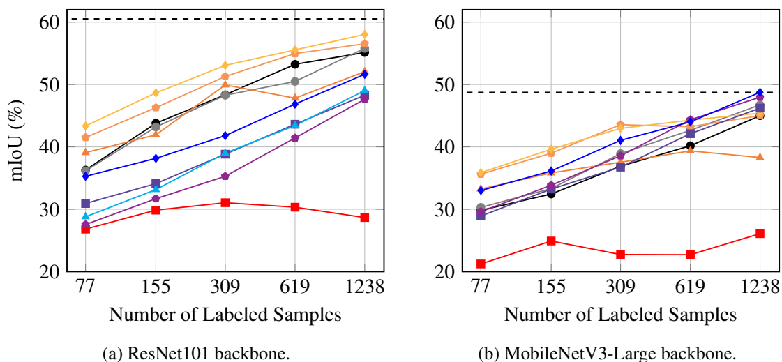
Figure 6.4: mIoU (%) comparison between the methods for Cityscapes using DeepLabv3 model.
