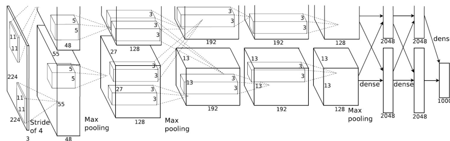
Figure 2.2: AlexNet architecture. Source: [8]
