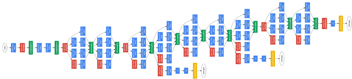
Figure 2.4: GoogLeNet architecture. Source: [12]
