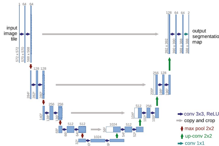
Figure 2.8: U-Net architecture. Source: [15]
