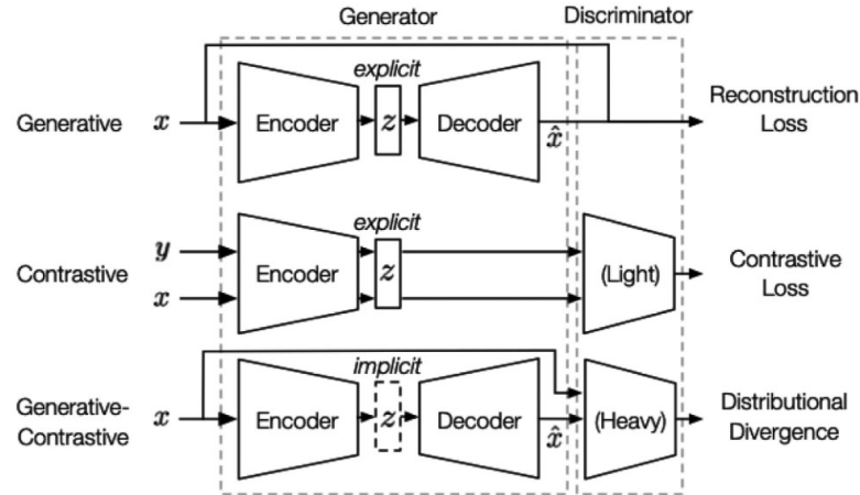
Figure 4.1: Conceptual comparison between self-supervision categories: Generative, Contrastive, and Generative-Contrastive. Source: [65]
