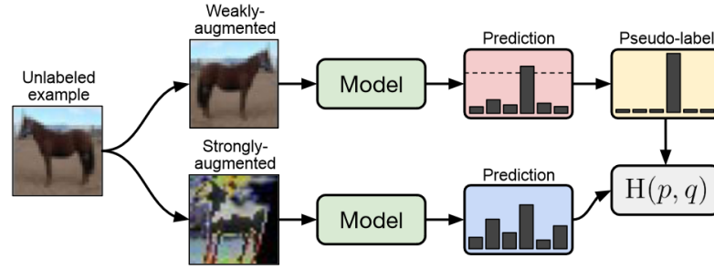
Figure 3.8: FixMatch pseudo-labeling algorithm diagram. For a single unlabeled sample, both weakly and strongly augmented images are generated using stochastic data augmentation and fed to the classifier for label prediction. The prediction from the weakly-augmented image serves as a pseudo-label and is compared with the strongly-augmented version. Source: [53]
