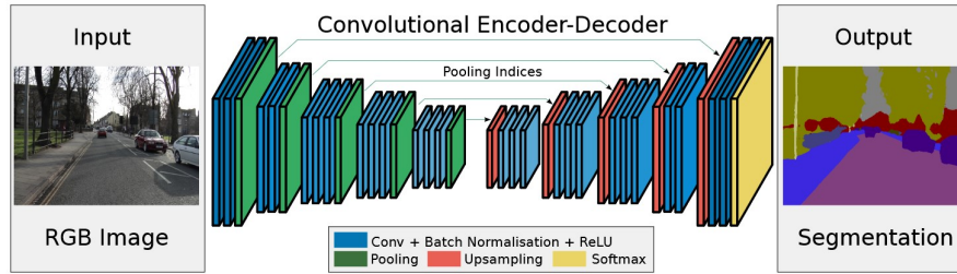
Figure 2.9: SegNet architecture. Source: [16]
