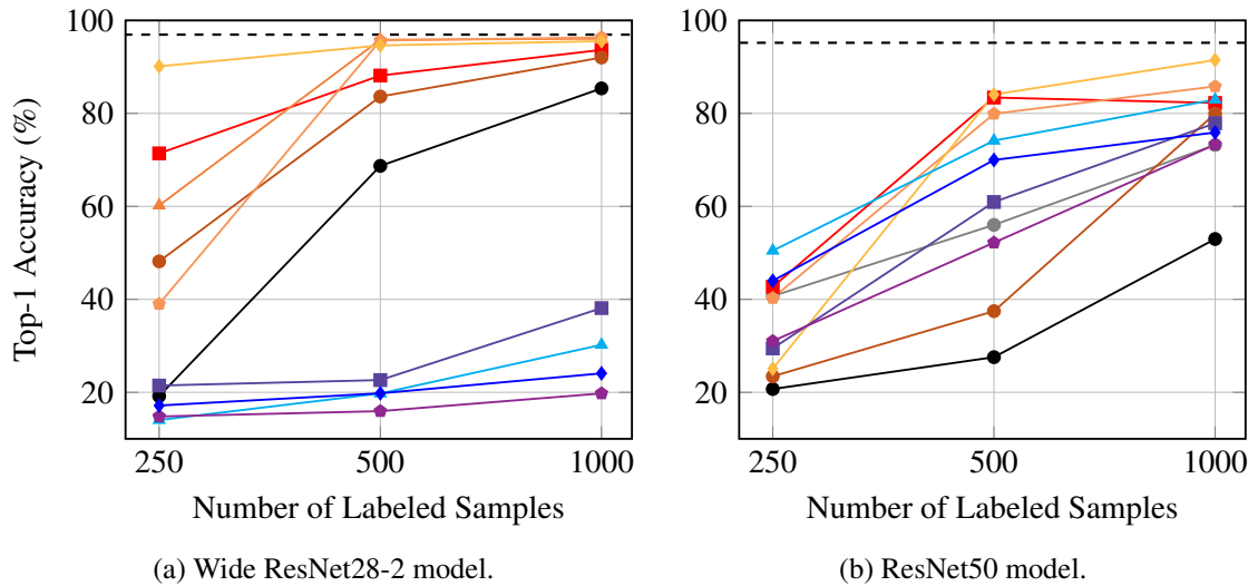
Figure 6.3: Top-1 Accuracy comparison between the methods for SVHN.
