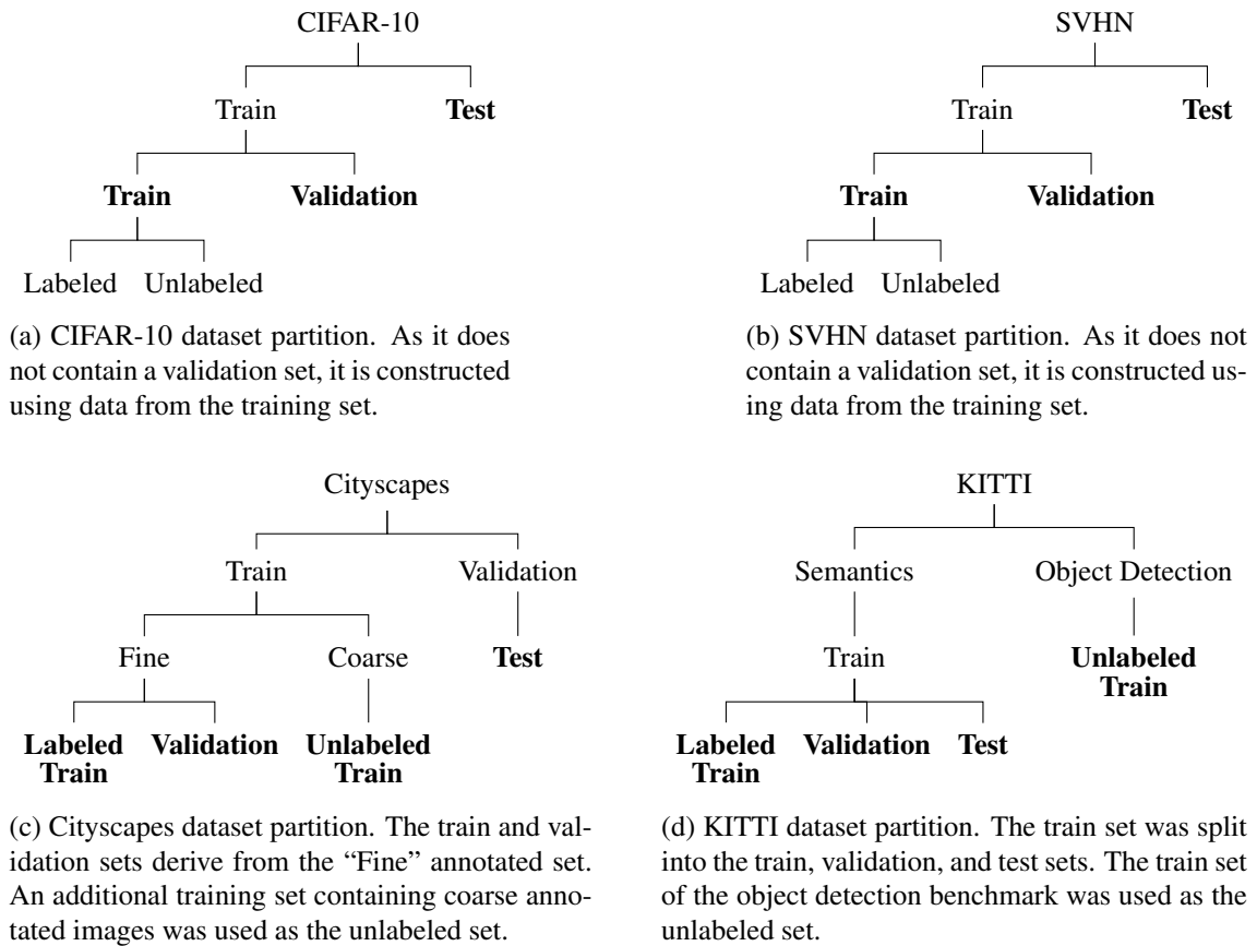
Figure 5.1: Datasets partition tree. The bold nodes represent the final train, validation, and test sets.
