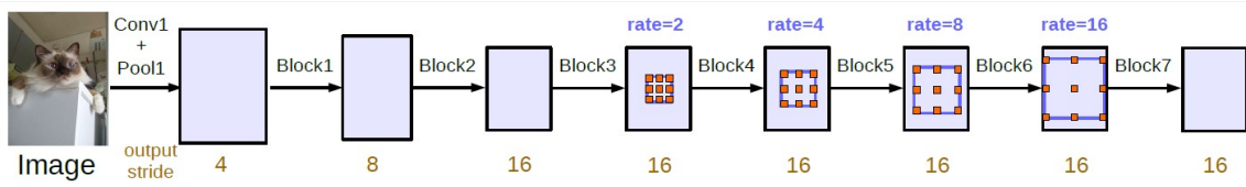
Figure 2.11: DeepLabv3 architecture. Source: [18]
