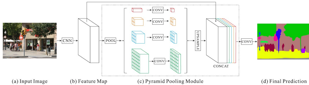
Figure 2.10: Pyramid Scene Parsing Network architecture. Source: [17]
