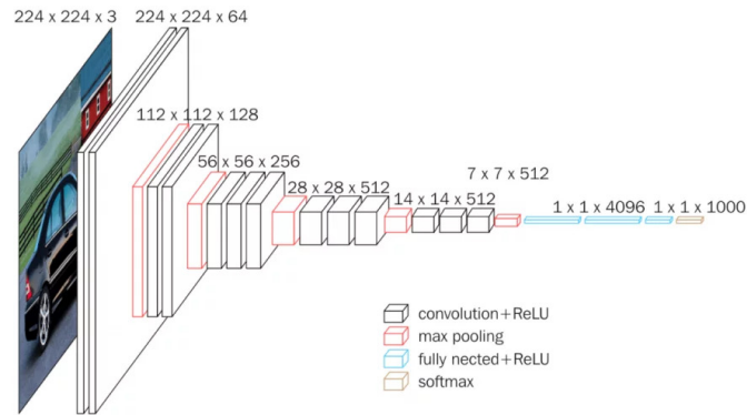
Figure 2.3: VGG16 architecture. Source: [11]
