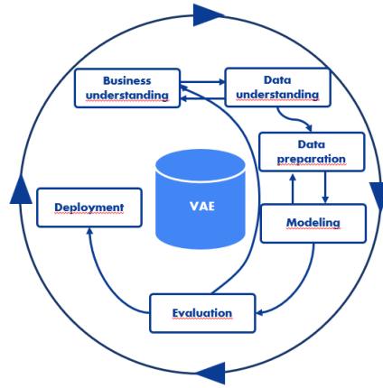
Figure 1.1: CRISP-DM Framework
