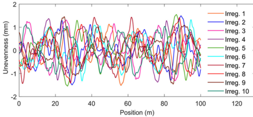
Figure 3.5: Simulation of 10 unevenness rail profiles for wavelengths between 1 m to 30 m
