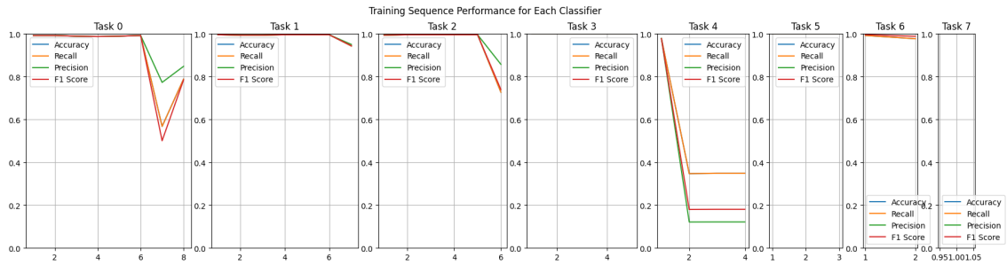
Figure 5.15: Performance throughout different tasks scenario four
