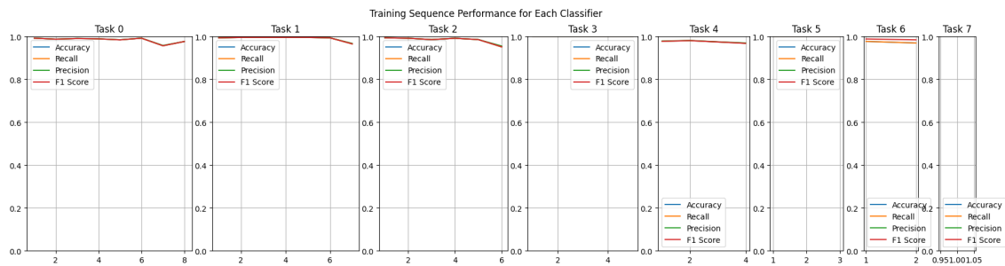
Figure 5.12: Performance throughout different tasks scenario one
