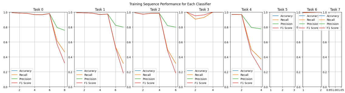
Figure 5.11: Performance throughout different tasks scenario zero
