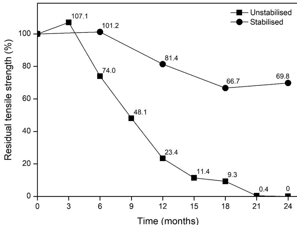
Figure 3. Residual tensile strength of geotextiles exposed to field weathering: unstabilised geotextile vs. stabilised geotextile. The stabilised geotextile data was collected from Carneiro & Lopes (2022).
