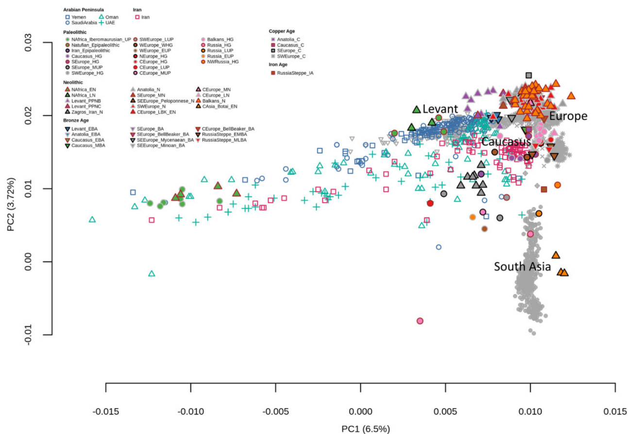
Fig. 1. —PCA of present-day samples from the AP (western AP in blue and eastern AP in green), Iran (red) and neighboring populations (gray, to avoid visual clutter) with projected ancient samples in different colors and formats according to the legend. Abbreviations: E, Early; M, Middle; L, Late; HG, hunter-gatherer; N, Neolithic; C, Chalcolithic; BA, Bronze Age; IA, Iron Age; UP, upper Paleolithic.
