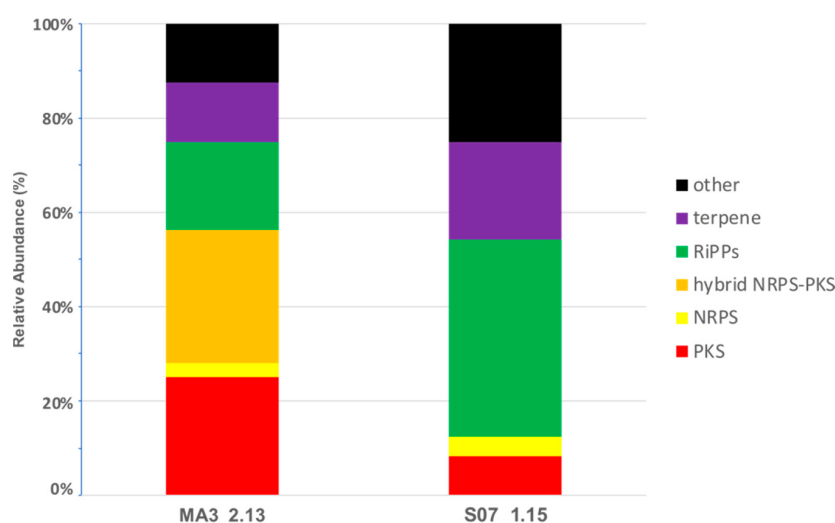
Figure 3. Occurrence of BGCs types in both strains as predicted by antiSMASH. Data were retrieved from Supplementary Tables S6 and S7.
