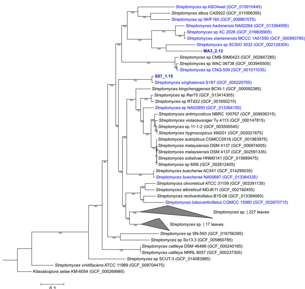
Figure 2. WGS phylogenetic tree of 280 NCBI RefSeq Streptomyces strains and isolates MA3_2.13 and S07_1.15 (highlighted in bold), generated using the GToTree workflow and visualized with the web-based tool Interactive Tree of Life ( https://itol.embl.de/ (accessed on 10 October 2021)). Portions of the tree collapsed are labelled and numbers represent the number of leaves/genomes in the collapsed subtrees. Strains name in blue indicate strains isolated from marine samples.
