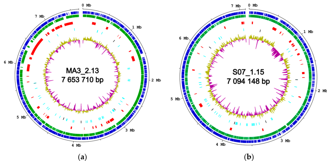
Figure 1. Schematic representation of the chromosomes of isolates MA3_2.13 (a) and S07_1.15 (b) generated by DNAPlotter v 18.1.0. The chromosomes are represented as open circles and for S07_1.15, only the large contig is shown. From outside to inside, the concentric circles represent: genome coordinates, coding sequences (CDS) in the forward strain (in blue) and in the reverse strain (in green), regions of putative BGCs (in red), tRNA and rRNA genes (in cyan and in black, respectively); GC percentage plot with default settings (above average in olive and below average in purple).
