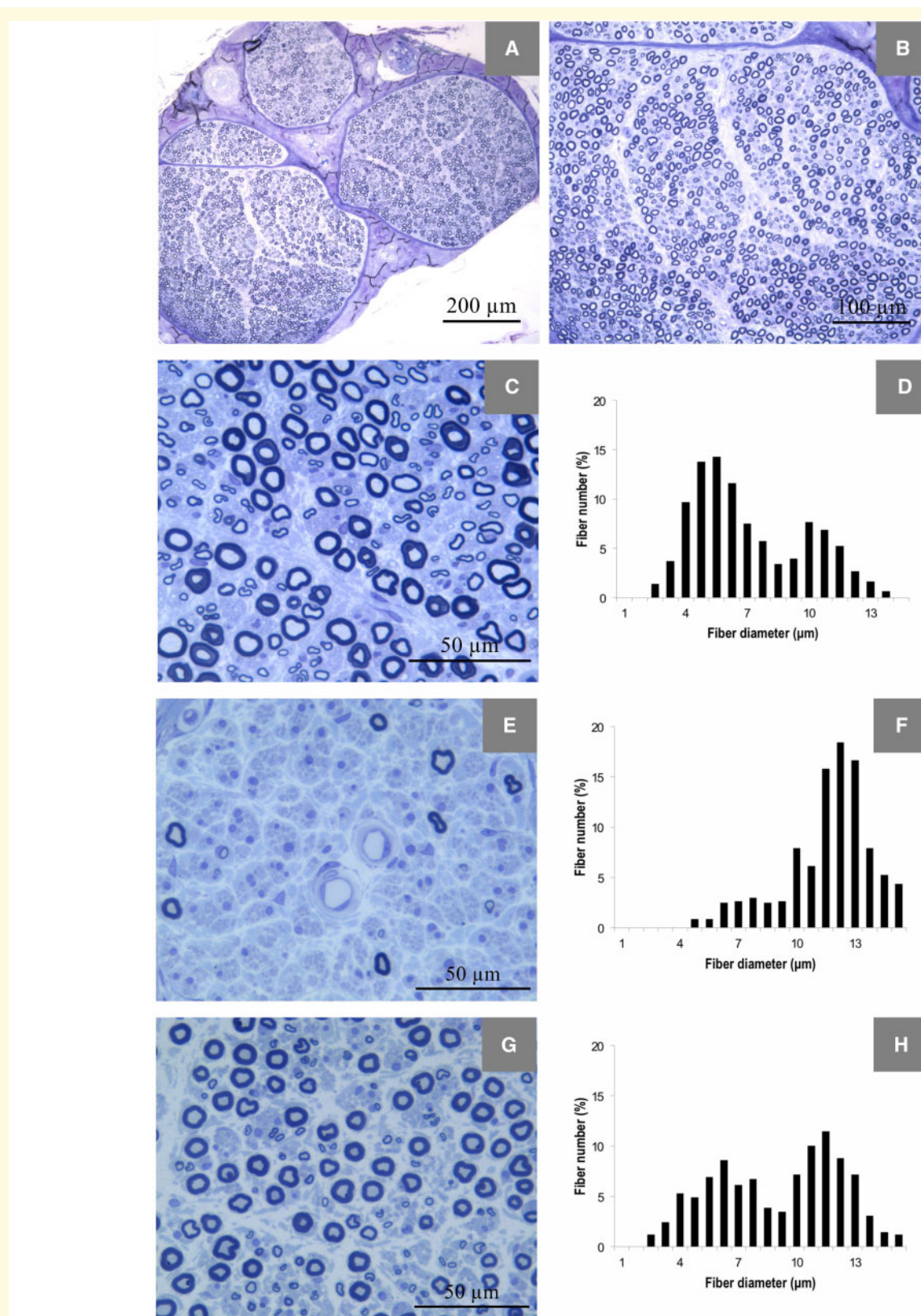
Figure 4 Morphometric findings in sural nerve specimens. Representative example photomicrographs of 1 μm transversal sections of sural nerve (stained with toluidine blue) from a control (A–C), a patient with familial amyloid polyneuropathy with transthyretin mutation (E) and an asymptomatic mutation carrier (G). In E, there is a severe depletion of both small and large myelinated fibres, and in G, there is a moderate loss of small myelinated fibres. Graphics show representative examples of diameter frequency histograms of myelinated fibres in sural nerve from a control (D), exhibiting a typical bimodal distribution of fibre diameters, with higher proportion of small myelinated fibre than of large myelinated fibres, a patient with familial amyloid polyneuropathy with transthyretin mutation (F), exhibiting loss of the bimodal distribution of fibre diameters, and an asymptomatic mutation carrier (H), presenting a higher peak of large than of small myelinated fibres, in contrast to the fibre size distribution in controls.
