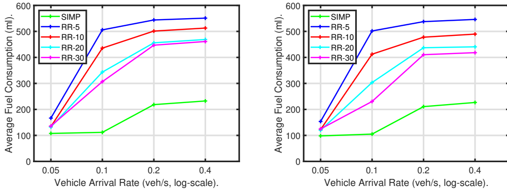
(a) Average fuel consumption at 30\text{km/h} . (b) Average fuel consumption at 50\text{km/h} .
