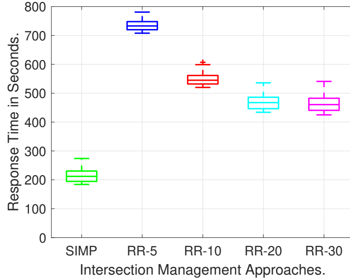
Figure 7.3: Observed response time of 50 vehicles for 100 simulation runs, with an average traffic injection rate of 0.2veh/s .
