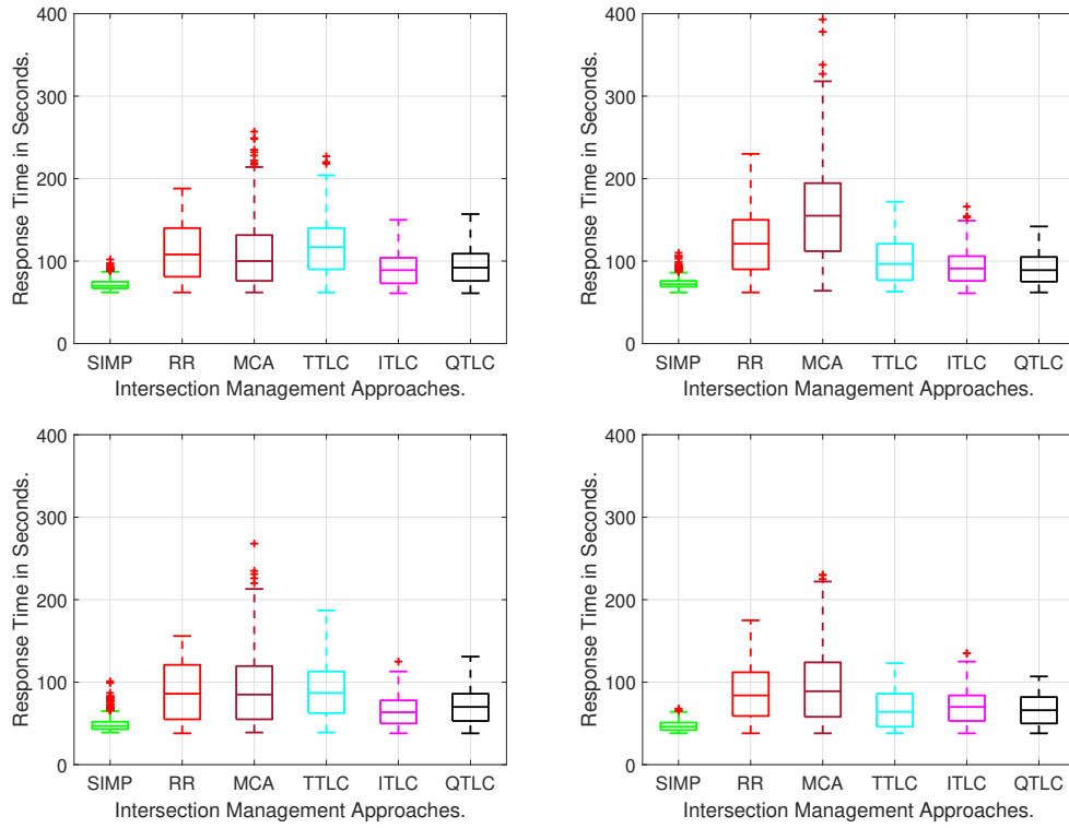
Figure 7.12: Observed response time (s) of 1000 vehicles for 30km/h (top) and 50km/h (bottom), L-crossing (left) and S/R-crossing (right) lanes at \lambda = 0.033veh/s and 0.067veh/s respectively, and C = 50veh (non-saturated traffic).
