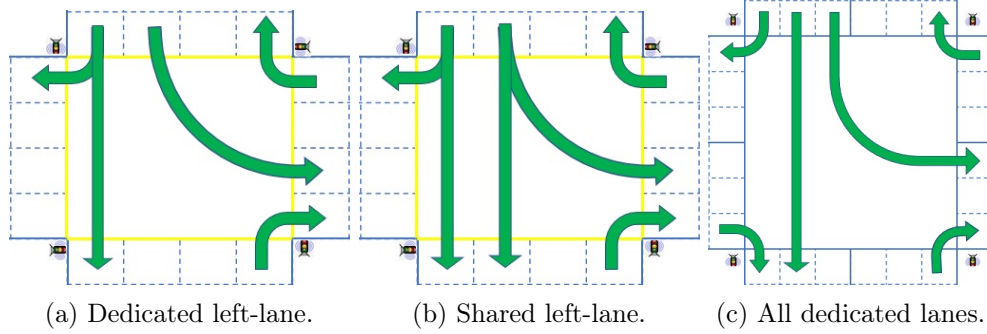
Figure 3.4: RR IM approach green phase layout for a). dedicated and b). shared left-lane intersections with two inflow/outflow lanes, and c). every lane is dedicated to a specific crossing direction in a three-lane intersection.
