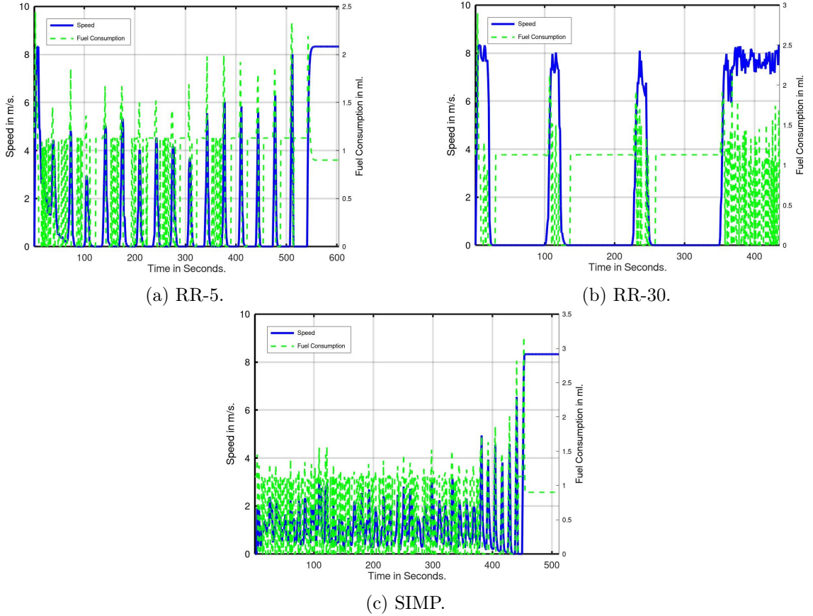
Figure 8.1: Speed and fuel consumption of 500 th vehicle an AV in RR-5, RR-30, and SIMP protocol in which all vehicles cross their left.
