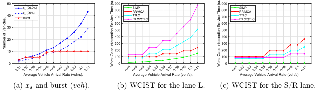
Figure 7.8: Maximum burst x_s (left) and WCIST against the long-term average vehicle arrival rate in \text{veh/s} considering x_s values with 99.9% confidence for left lanes (center) and right lanes (right).
