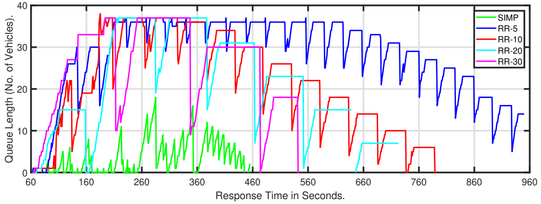
Figure 7.4: Queue length (number of vehicles) along time, with an average traffic injection rate of 0.2veh/s.
