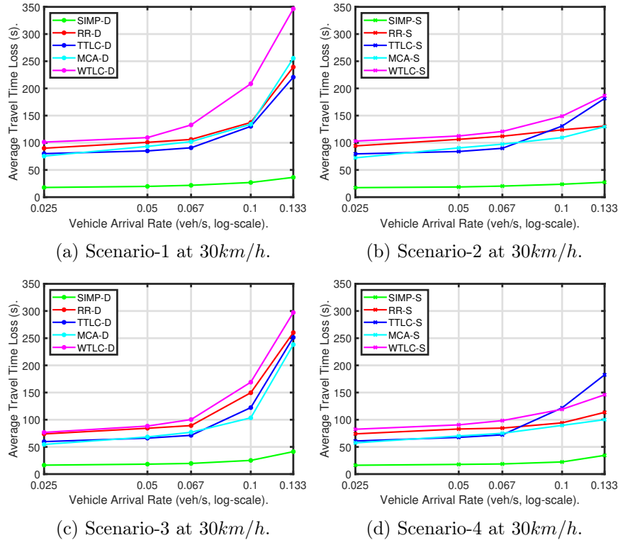
Figure 6.8: Average travel time loss ( s/veh ) of 2500 vehicles for homogeneous (top plots) and heterogeneous (bottom plots) road networks at 30 \text{ km/h} maximum speed imposed by the comparing IM approaches in both dedicated and shared left lane intersections.
