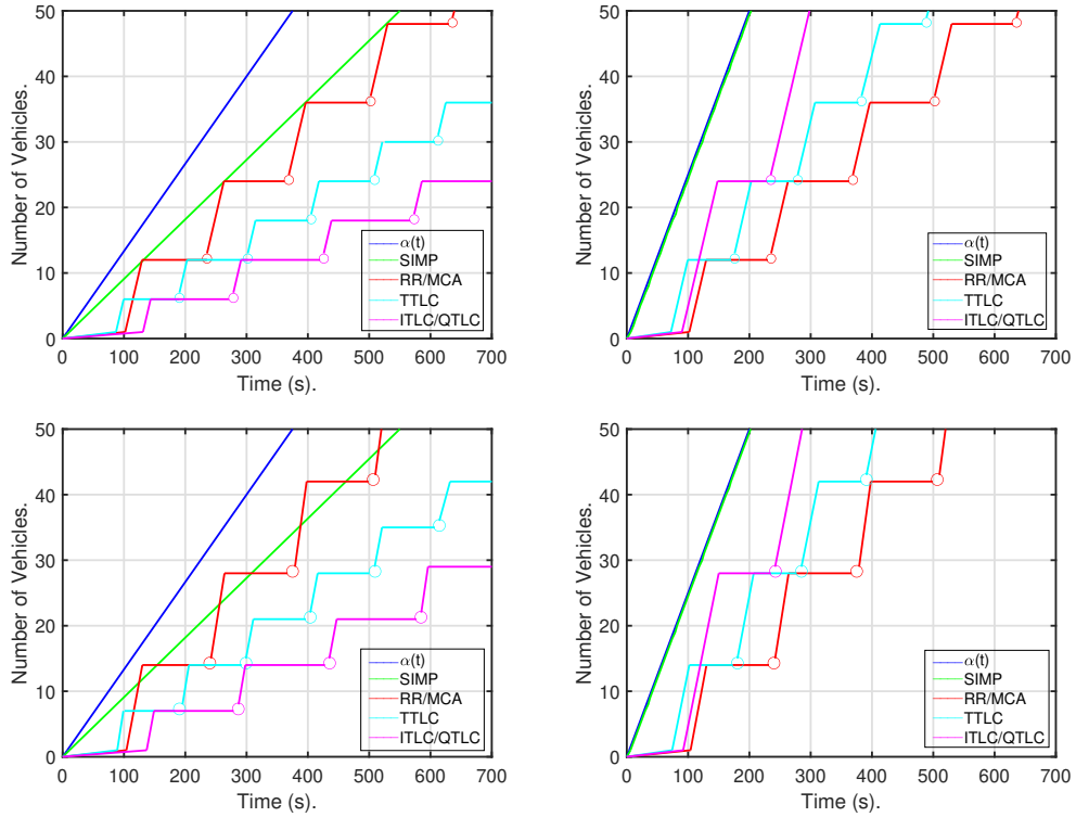
Figure 7.5: Arrival and service curves at 30km/h (top) and 50km/h (bottom), for the dedicated left lane (left) with s = 0.133veh/s , and a shared right lane (right) with s = 0.266veh/s .
