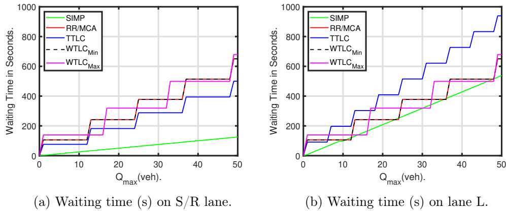
Figure 7.15: Waiting time delay (s) for various IM approaches with C = 50 on S/R- and L- lanes.
