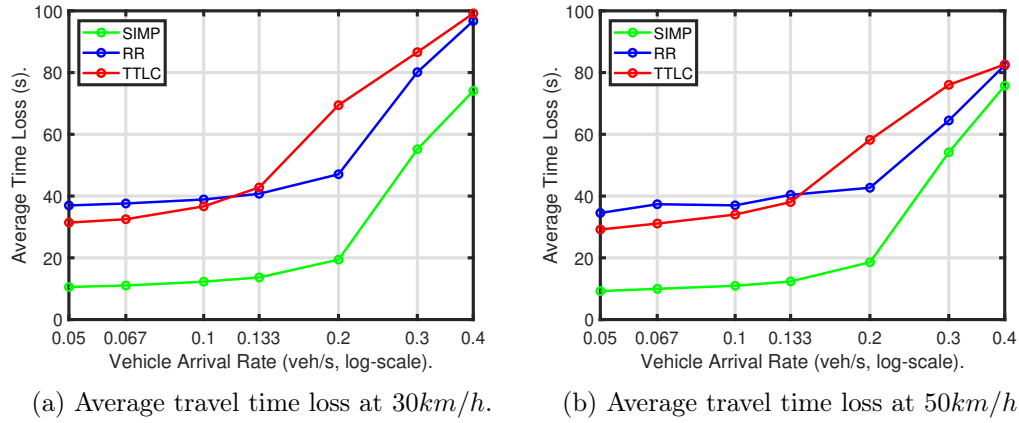
Figure 5.9: Average travel time loss results in s/\text{veh} for various arrival rates and vehicle count of the comparing IM approaches for 30\text{km/h} and 50\text{km/h} maximum speeds.
