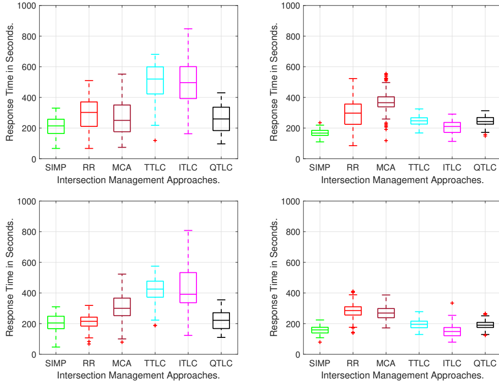
Figure 7.13: Observed response time (s) of 50^{th} vehicle for 30\text{km/h} (top) and 50\text{km/h} (bottom), L-crossing (left) and S/R-crossing (right) lanes at \alpha(t) = 0.4\text{veh/s} and C = 50\text{veh} (saturated traffic).
