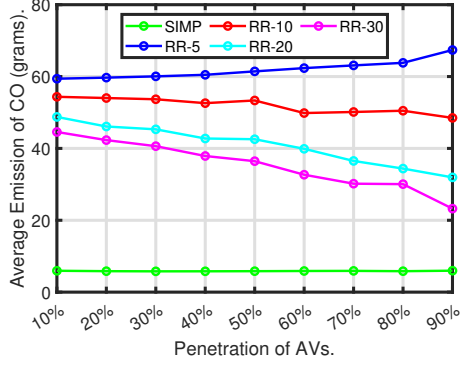
(a) Average emission of CO ( grams ).
