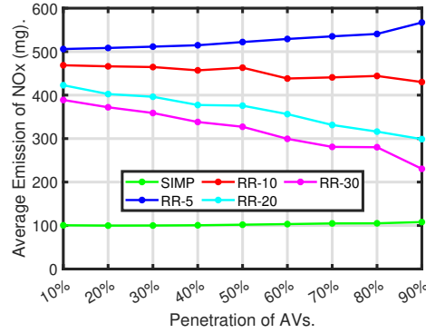
(c) Average emission of NO x ( mg ).
