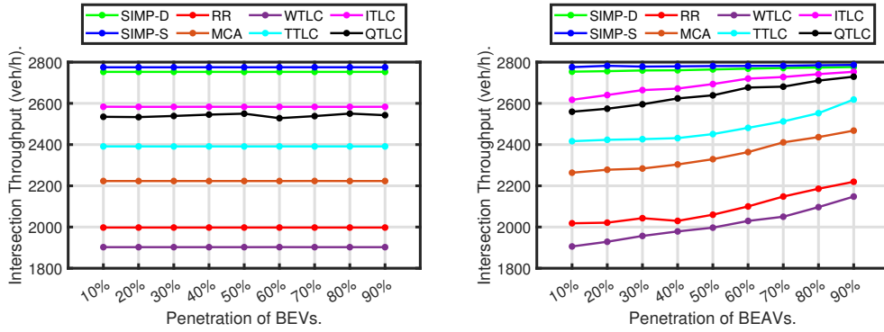
(a) Throughput for growing rates of BEVs. (b) Throughput for growing rates of BEAVs.
