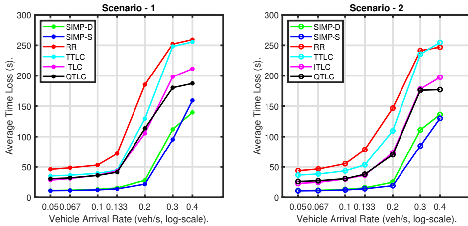
Figure 5.6: Average travel time loss ( s ) of 1000 vehicles for Scenario-1 and Scenario-2 at 30km/h maximum speed.
