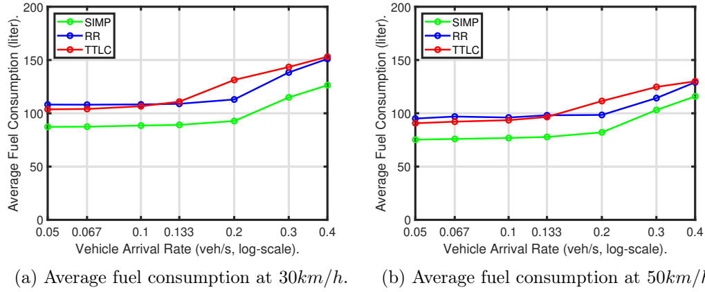
Figure 5.10: Average fuel consumption results in liters for various arrival rates and vehicle count of the comparing IM approaches for 30km/h and 50km/h maximum speeds.
