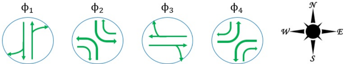
Figure 4.11: Best possible composition of green phases.
