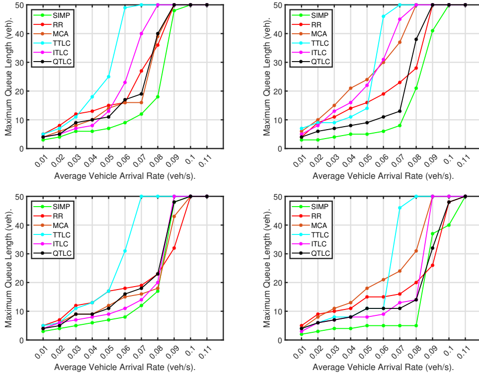
Figure 7.9: IM induced Q_{max} in \text{veh} against the long-term average vehicle arrival rate in \text{veh/s} for the left-crossing lane (left) and right lane (right) at 30 \text{ km/h} (top) and 50 \text{ km/h} (bottom) maximum speeds and capacity C = 50 \text{ veh} .
