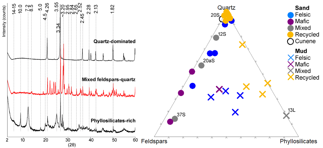
FIGURE 4 XRD bulk mineralogy obtained for sand and mud deposits. Samples with mixed source are identified. Note the strong quartz-domain in sands with an important recycled component, quartz to quartz-feldspar (mainly K-feldspar) if sources are predominantly felsic and high feldspar (mainly plagioclase) if sources are predominantly mafic. Muds contain substantially more quartz than feldspar only where the source area comprises sedimentary units.
