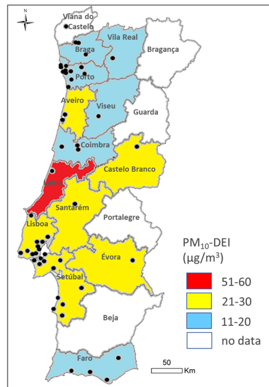
Fig. 6. Additional population exposure to PM 10 (mean Daily Exposure Increments - DEI) during the 24 smoky days (with dust and dust-free) in October 2017 as estimated from the air quality monitoring data. Additional information in Table 2.
