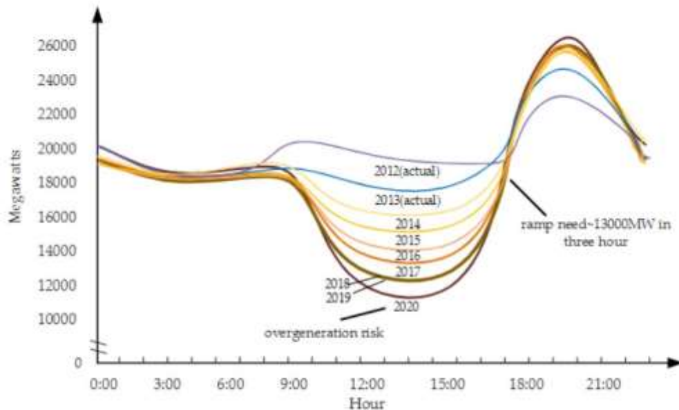
Fig. 1.6 - “The CAISO predicted duck curve” [Q. Wang et al., “Mitigation strategy for duck curve in high photovoltaic penetration power system using concentrating solar power station,” Energies , vol. 12, no. 18, Sep. 2019]
