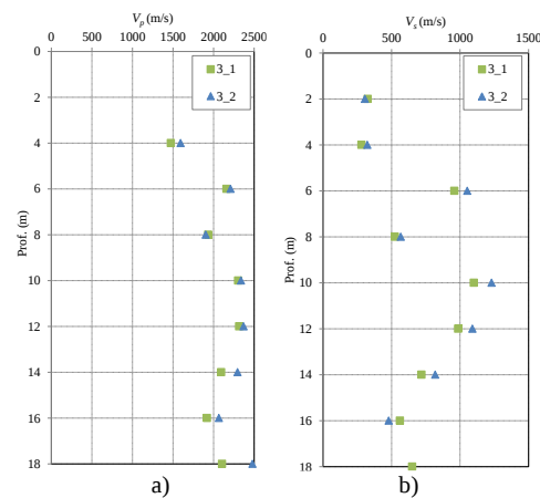
Figure 4. Results from CH sections using a S-wave sparker source: a) V_P ; b) V_S .
