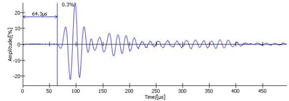
Figure 17. P-wave velocity measurement with ultrasonic transducers in sample 5 Pundit® (82 kHz).
