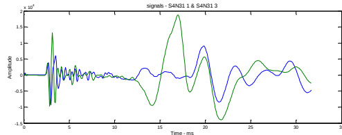
Figure 9. Seismograms S4N31_1 and S4N31_3.
