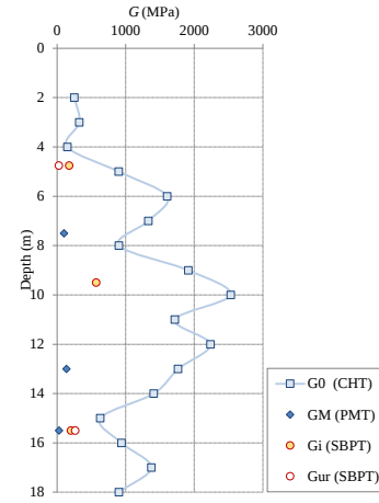
Figure 20. Shear modulus, G_0 , from in situ tests.
