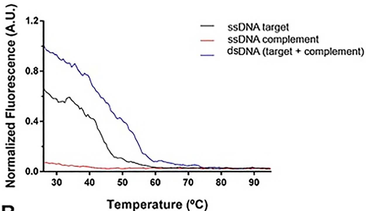
Fig 4. High resolution melt curve. (A) dsDNA(Target+capture): T_m = 78^\circ\text{C} ; dsDNA(target+capture-(TEG)Biotin): T_m = 82^\circ\text{C} ; (B) and dsDNA(target+complement): T_m = 53^\circ\text{C} . All analyzes are compared to the corresponding ssDNA (ssDNA target or complement).
