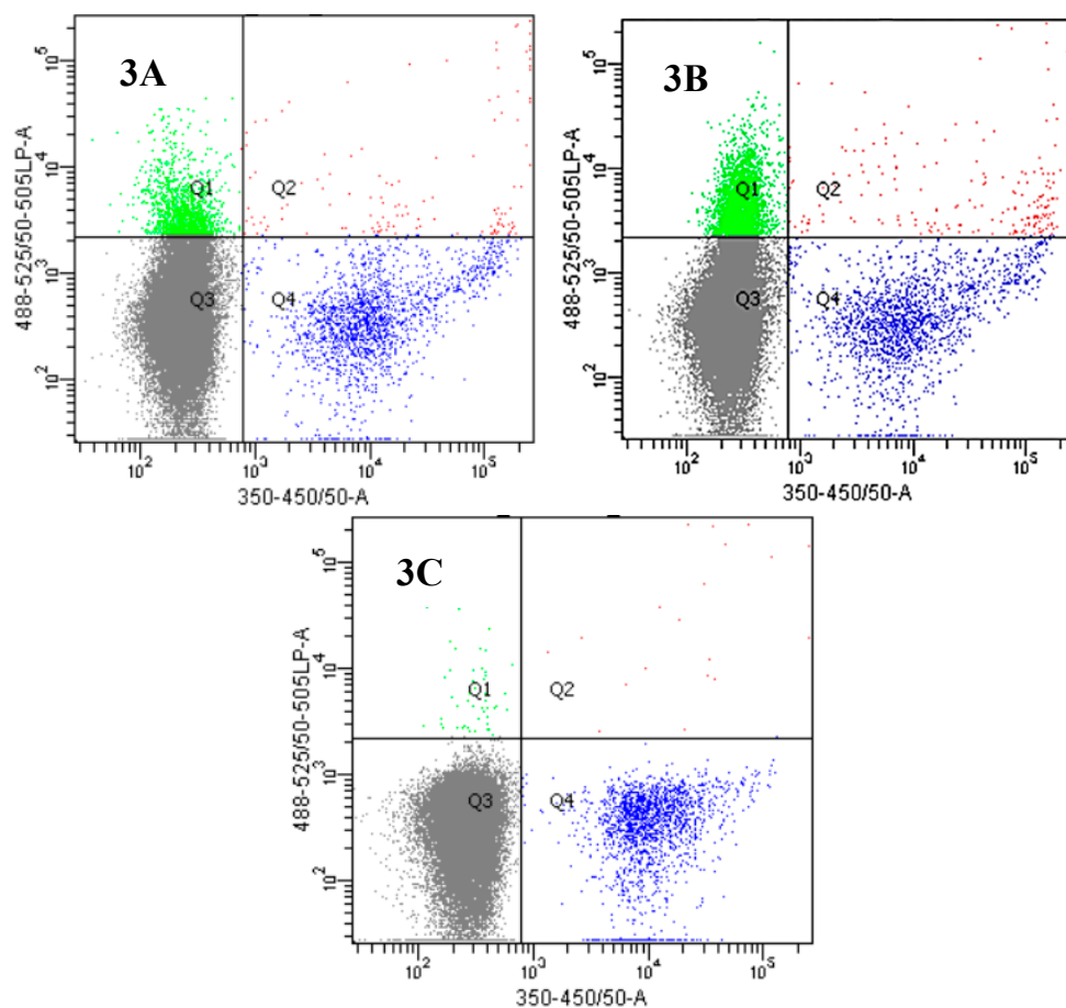
Figure 3. Flow cytometry analysis of the interaction between hRBC/PiRBC and CF-labelled (A) TP10, (B) Cq-C4-TP10, and (C) Cq-C4-TAT. Upper quadrants (Q1 and Q2) refer to compound-bound cells (green CF fluorescence) and right-hand quadrants (Q2 and Q4) refer to PiRBC (blue Hoechst fluorescence). Q3 includes hRBC, which were not internalized by the CF-labelled test compounds.
