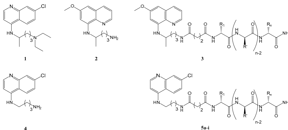
Figure 1. Structures of CQ ( 1 ), PQ ( 2 ), PQ-CPP conjugates previously disclosed by us ( 3 ) [20], and the chloroquine analogue (Cq, 4 ) bearing a free primary amine to be linked to CPP (Table 1), and afford the first generation of Cq-CPP conjugates (Cq-C4-CPP, 5a–i ).
