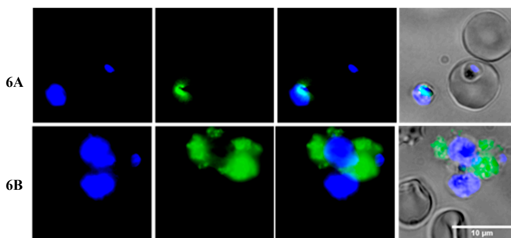
Figure 6. Microscopy fluorescence images showing an apparent co-localization of (A) CF-labeled TP10 (15) and DNA of parasites released after PiRBC disruption, or of (B) CF-labeled Cq-C4-TP10 (16) and what appears to be PiRBC debris surrounding nuclei of released parasites.
