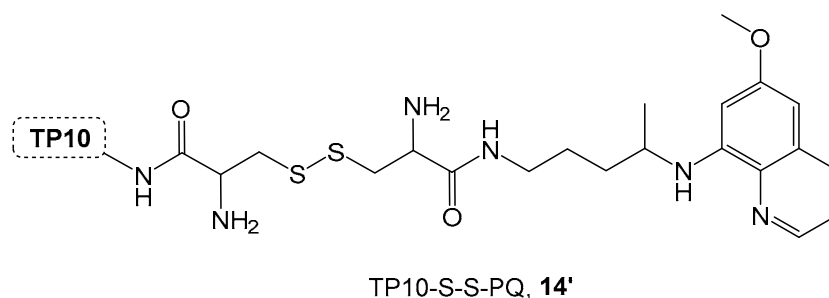
Figure 2. Structure of conjugate 14' , TP10-S-S-PQ.
