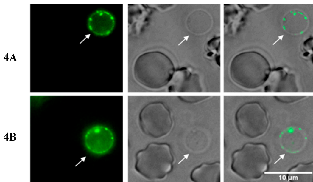
Figure 4. Microscopy fluorescence images showing the interaction between hRBC and (A) CF-labeled TP10 (15) and (B) CF-labeled Cq-C4-TP10 (16). Arrows depict “ghost” uninfected erythrocytes.
