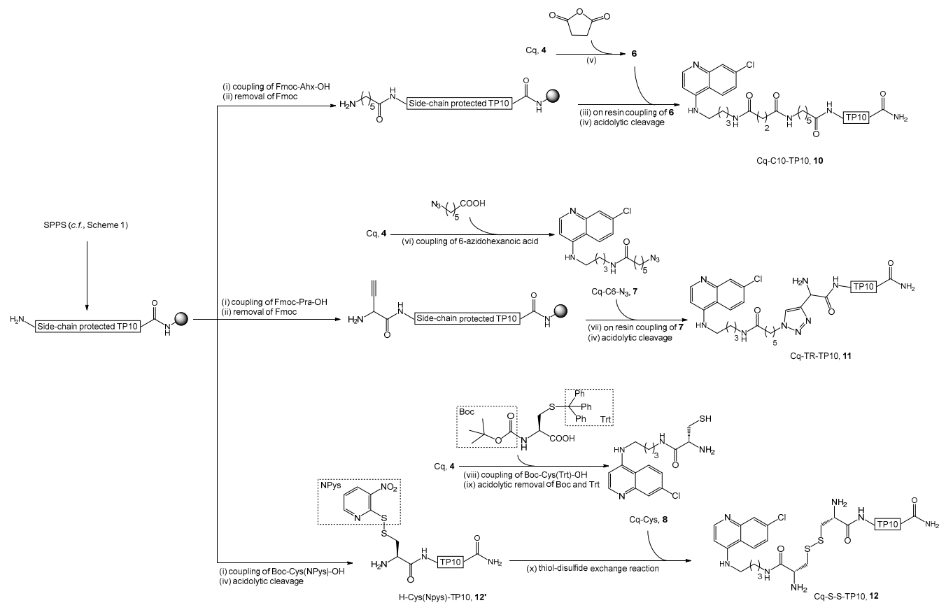
Scheme 2. Synthesis of conjugates 10–12 : (i) 5 eq, respective to the resin reactive groups, of the fluorenylmethoxycarbonyl (Fmoc) or tert-butyloxycarbonyl (Boc)-AA-OH in DMF (0.2 M), 5 eq of 0.5 M HBTU/HOBt in DMF, and 10 eq of 2 M DIPEA in N -NMP, MWI for 5 min at 35 W; (ii) 20% piperidine in DMF containing 0.1 M of HOBt, MWI for 30 s at 24 W plus 3 min at 28 W; (iii) 5 eq of 6 and of PyBOP, 10 eq DIPEA in DMF, RT, overnight; (iv) TFA/water/TIS 95:2.5:2.5 v/v/v (1 mL/100 mg of resin), RT, 120 min; (v) 1.2 eq of succinic anhydride and of DIPEA in DMF, RT, 120 min; (vi) 6-azido hexanoic acid (1.2 eq), HBTU (1.2 eq), DIPEA (2.4 eq) in DMF, 0 °C → RT, 3 h; (vii) copper(I) bromide (1.2 eq), 2,6-lutidine (10 eq), sodium ascorbate (3 eq), and DIPEA (10 eq), solubilized in a mixture of acetonitrile (ACN) and DMF (1:2 v/v ), RT, overnight; (viii) Boc-Cys(Trt)-OH (1.2 eq), HBTU (1.2 eq), DIPEA (2.4 eq) in DMF, 0 °C → RT, 3 h; (ix) TFA:TIS:H 2 O 95:2.5:2.5 ( v/v/v ), 1 h, 0 °C → RT; (x) 1 M aqueous acetic acid, RT, 36 h. Grey sphere stands for the Rink-amide resin used as polymer support used for SPPS. Ph, phenyl group.
