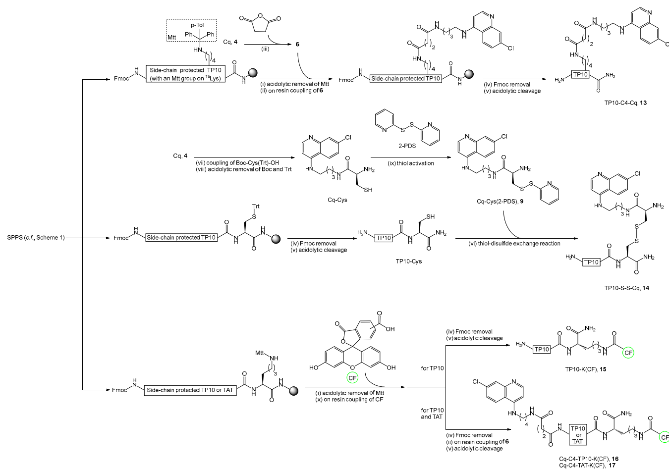
Scheme 3. Synthesis of conjugates 13–17: (i) resin treated with 1% TFA in DCM, RT, until no yellow color detected in filtrate; (ii) 5 eq of 6 and of PyBOP, 10 eq DIPEA in DMF, RT, overnight; (iii) 1.2 eq of succinic anhydride and of DIPEA in DMF, RT, 120 min; (iv) 20% piperidine in DMF containing 0.1 M of HOBt, MWI for 30 s at 24 W plus 3 min at 28 W; (v) TFA/water/TIS 95:2.5:2.5 v/v/v (1 mL/100 mg of resin), RT, 120 min; (vi) 1 M aqueous acetic acid, RT, 36 h; (vii) Boc-Cys(Trt)-OH (1.2 eq), HBTU (1.2 eq), DIPEA (2.4 eq) in DMF, 0 °C → RT, 3 h; (viii) TFA:TIS:H 2 O 95:2.5:2.5 (v/v/v), 1 h, 0 °C → RT; (ix) 2,2'-dithiopyridine (2-PDS, 2.0 eq), glacial acetic acid (0.3 eq), anhydrous MeOH, 18 h, RT; (x) 5(6)-carboxyfluorescein (CF; 5.0 eq), PyBOP (5.0 eq), DIPEA (10 eq), DMF, 2 h, RT.
