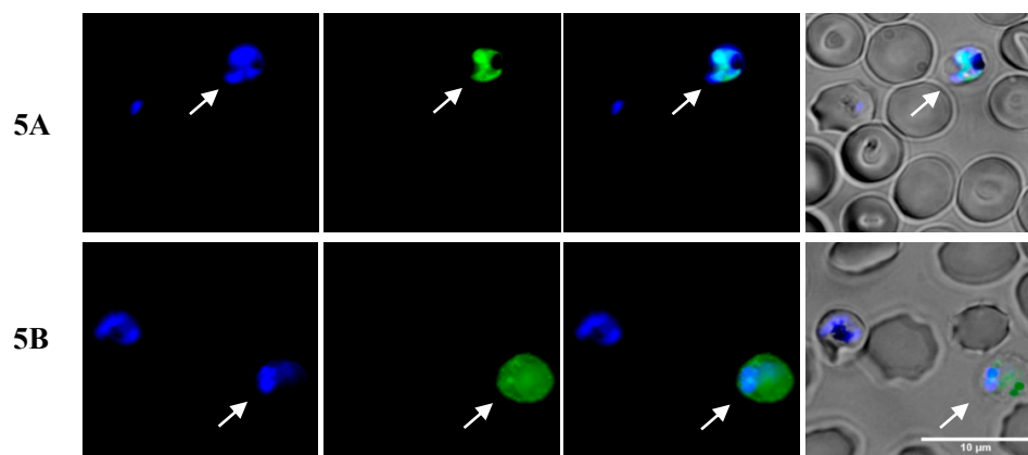
Figure 5. Microscopy fluorescence images showing the interaction between PiRBC (distinguished by the blue staining of parasites' nuclei) and (A) CF-labeled TP10 (15) and (B) CF-labeled Cq-C4-TP10 (16). Arrows depict “ghost” Plasmodium -infected erythrocytes.
