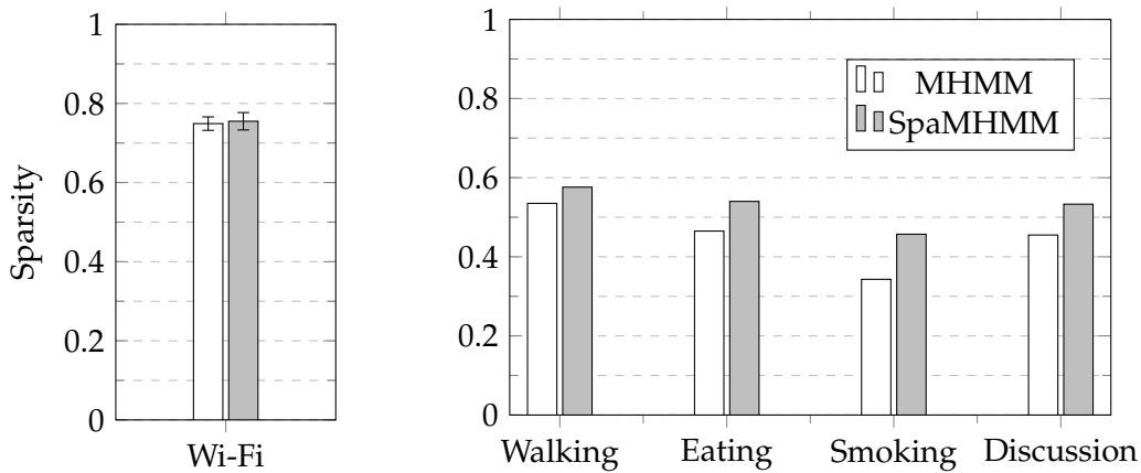
FIGURE 3.7: Relative sparsity (number of coefficients equal to zero / total number of coefficients) of the obtained MHMM and SpaMHMM models on the Wi-Fi dataset (left) and on the Human3.6M dataset for different actions (right). For the Wi-Fi dataset, the average value over the 10 training runs is shown together with the standard deviation. Both models for the Wi-Fi dataset have 150 coefficients. All models for the Human3.6M dataset have 396 coefficients.
