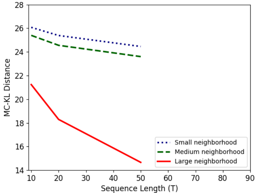
FIGURE 3.3: Monte Carlo approximation of the Kullback-Leibler divergence between the random and reference HMMs with different neighborhood sizes and sequence lengths.
