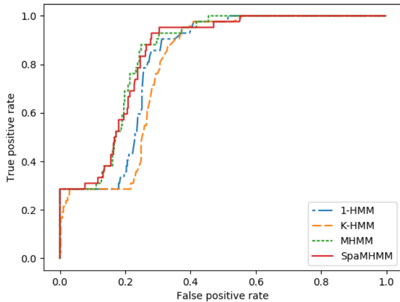
FIGURE 3.6: ROC curves for each model on the Wi-Fi dataset, for one of the 10 runs.
