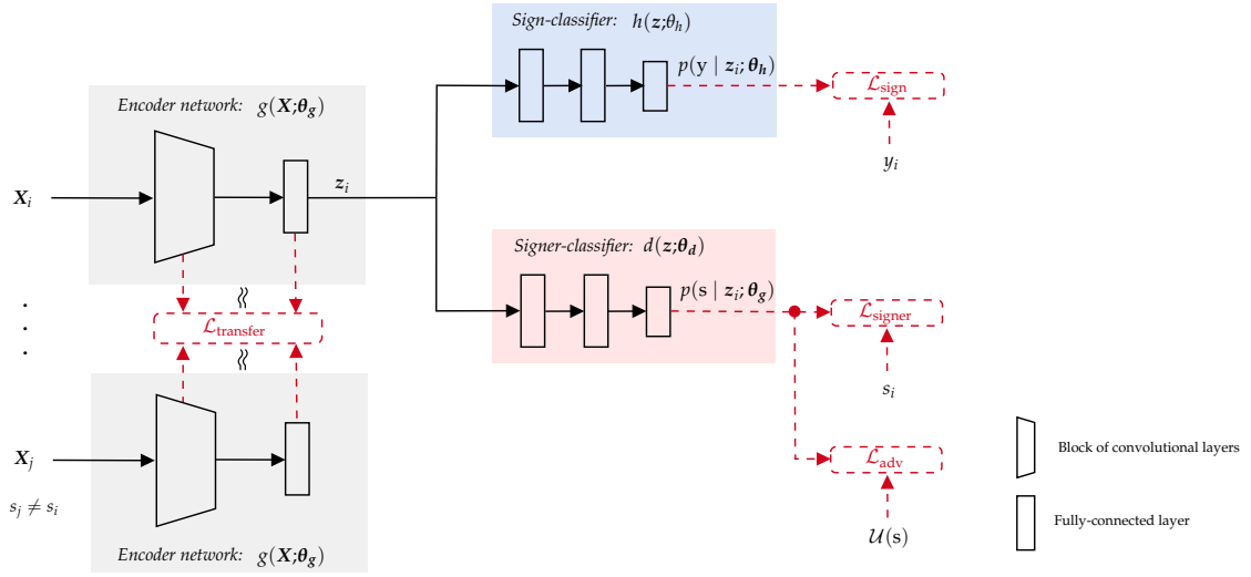
FIGURE 5.2: The architecture of the proposed signer-invariant neural network. It comprises three main sub-networks or blocks, i.e. an encoder, a sign-classifier and a signer-classifier.
