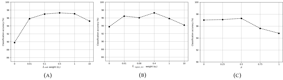
FIGURE C.5: Hyperparameter sensitivity analysis: (A) DeSIRE accuracy on the Jochen-Triesch dataset with varying values of \lambda_1 \in [0, 10] while \alpha_2 = 0.4 and \rho = 0.5 ; (B) DeSIRE accuracy on the Jochen-Triesch dataset with varying values of \alpha_2 \in [0, 10] while \lambda_1 = 0.5 and \rho = 0.5 ; and (C) DeSIRE accuracy on the Jochen-Triesch dataset with varying values of \rho \in [0, 1] while \lambda_1 = 0.5 and \alpha_2 = 0.4 .
