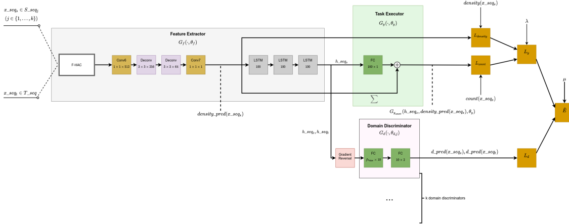
FIGURE 4.9: CommonLSTM model. Reprinted from de Andrade [63].
