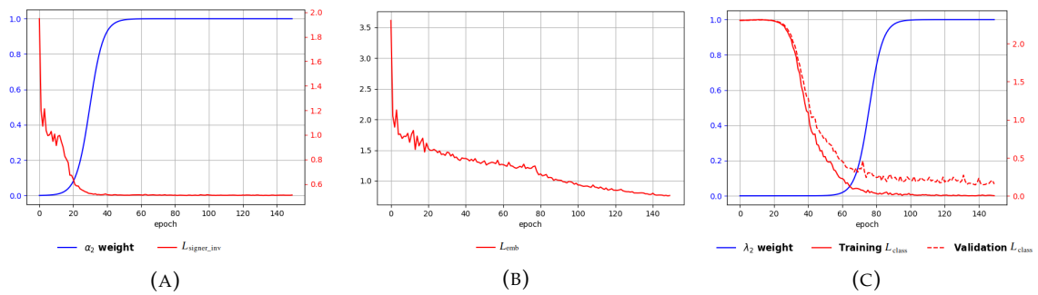
FIGURE C.4: Training behavior of the proposed DeSIRe model: (A) evolution of the L_{\text{signer\_inv}} loss term alongside the corresponding weight \alpha_2 according to a sigmoid annealing schedule; (B) evolution of the L_{\text{emb}} term value; and (C) evolution of training and validation L_{\text{class}} curves alongside the corresponding weight \lambda_2 according to a sigmoid annealing schedule.
