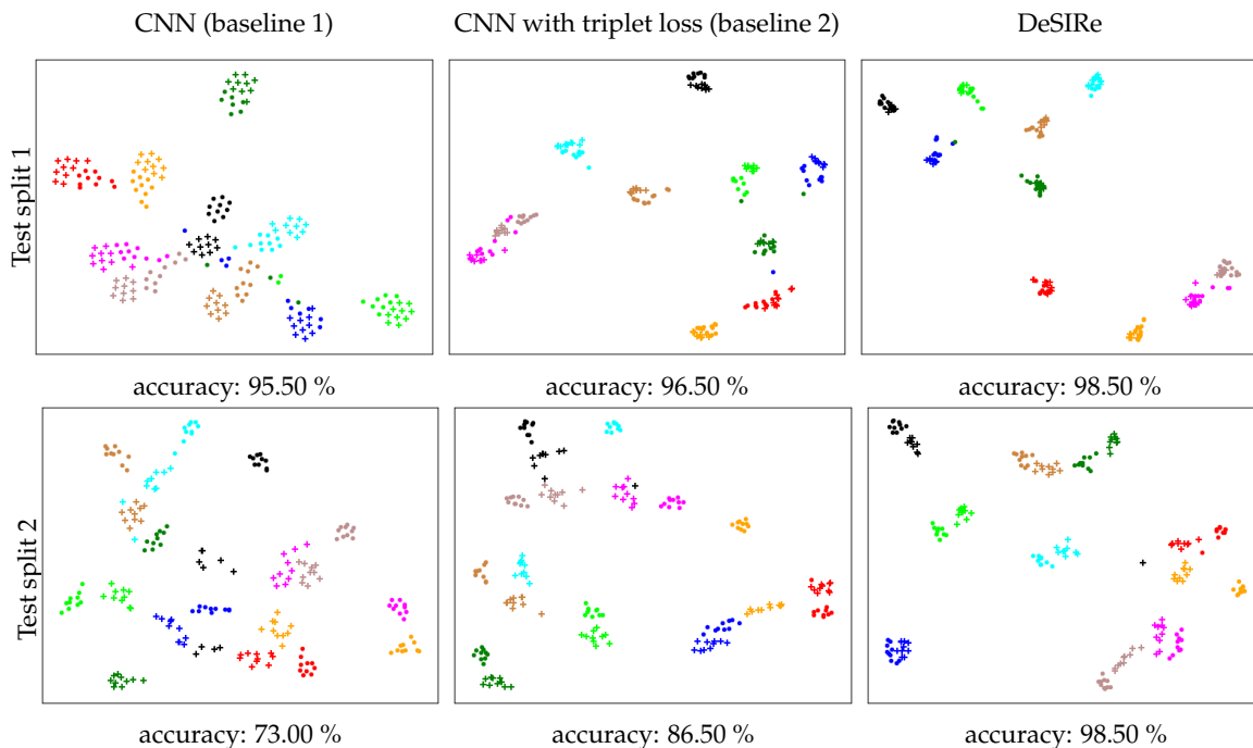
FIGURE C.2: Two-dimensional projection of the latent representation space provided by DeSIRe and both baselines, using t-SNE [185]. Markers \bullet and + represent two different test signers from the MKLM dataset and the different colors correspond to the 10 sign classes. The accuracy of each model on each split is shown below each picture.
