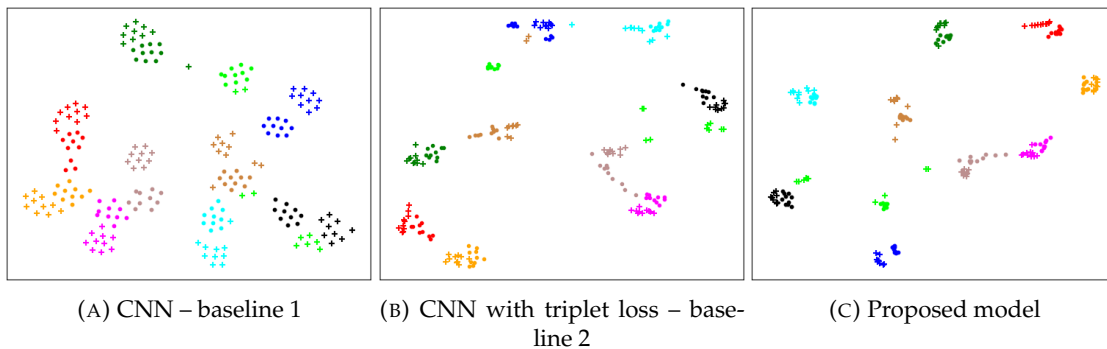
FIGURE 5.4: Two-dimensional projection of the latent representation space using the t-distributed stochastic neighbor embedding (t-SNE). Markers \bullet and + represent 2 different test signers, while the different colors denote the 10 sign classes.
