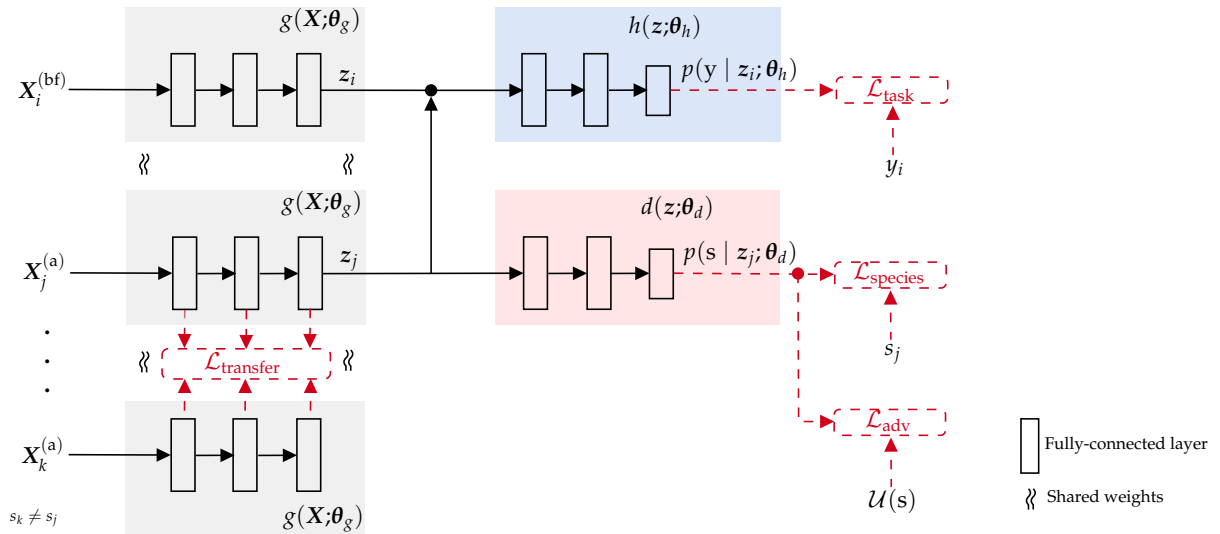
FIGURE 5.5: Block diagram of the proposed species-invariant neural network.
