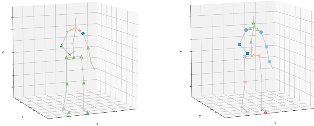
FIGURE 3.8: Assignments of joints to clusters in MHMM (left) and SpaMHMM (right). The different colors (blue, green, orange, red) and the respective symbols ('o', 'Δ', 'x', '+') on each joint represent the cluster that the joint was assigned to.
