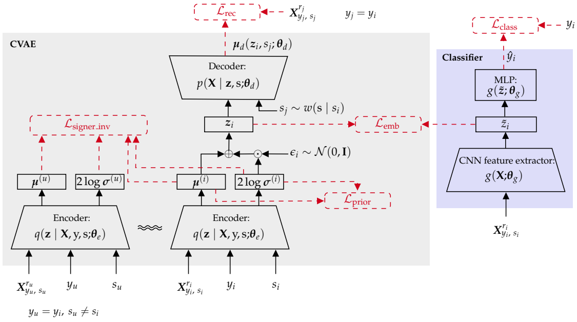
FIGURE C.1: The architecture of the proposed DeSIRe deep neural network for signer-independent SLR. It comprises two main modules or components: a conditional variational autoencoder (CVAE) and a classifier.
