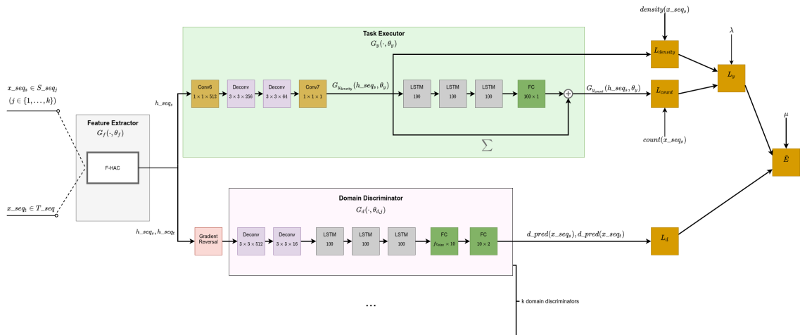
FIGURE 4.8: Double-Temporal model. Reprinted from de Andrade [63].
