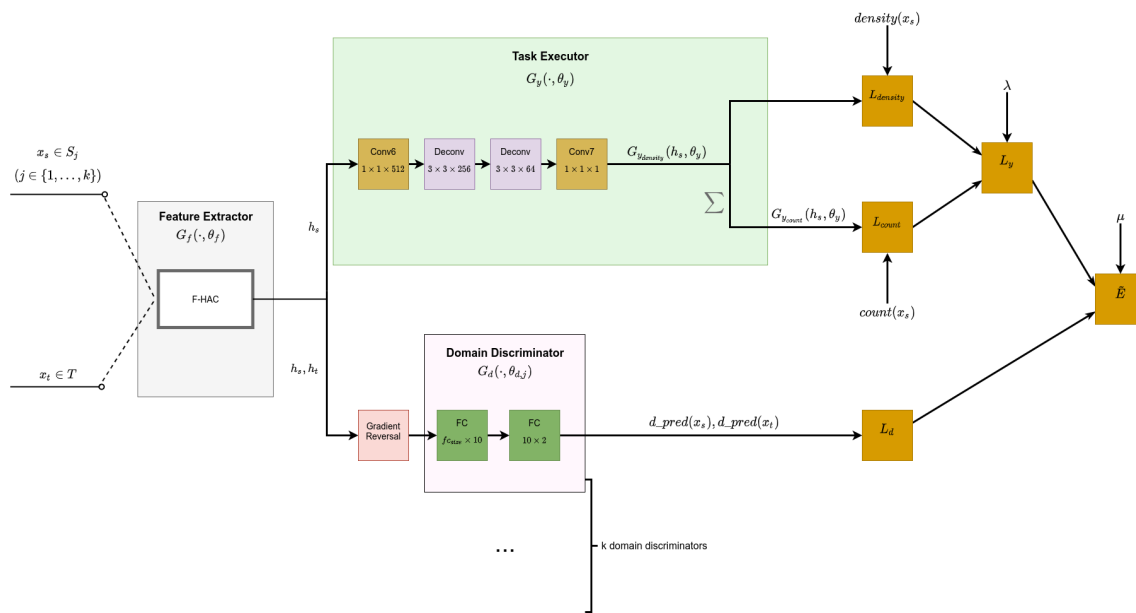
FIGURE 4.6: Non-Temporal model. Reprinted from de Andrade [63].
