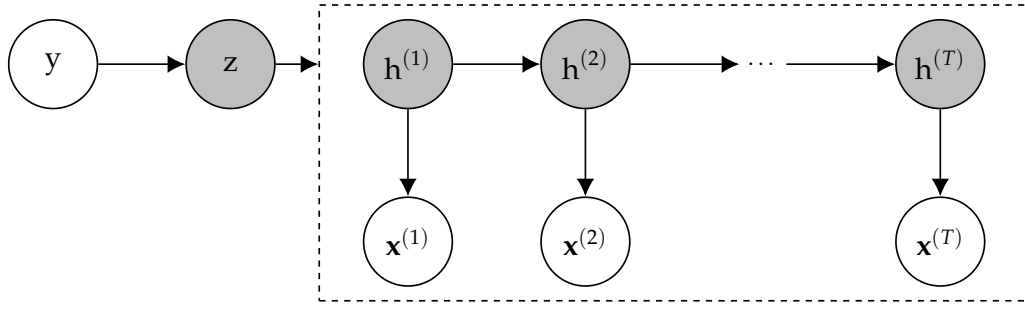
FIGURE 3.5: Representation of the model as a Bayesian network. The node z is a parent of all nodes inside the dashed box (the connections were omitted for clarity). Gray nodes are used for latent variables.
