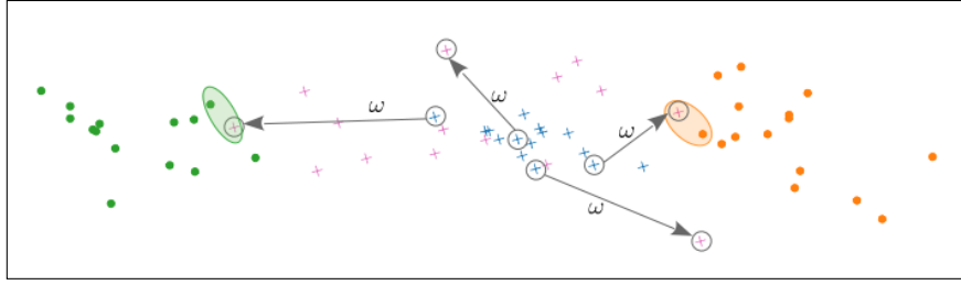
FIGURE 4.19: Toy illustration of the desired effect of the consistency regularization, where images are represented as lying on a 2-D space. Green and orange circles represent (labeled) samples from two distinct source domains; blue and purple x-markers represent original and augmented (unlabeled) target samples, respectively. Colored ellipses enclose pairs of augmented and source samples that are close to each other and therefore are likely to share the same label.
