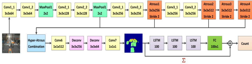
FIGURE 4.5: Architecture of the FCN-rLSTM model (reprinted from Zhang et al. [118]).
