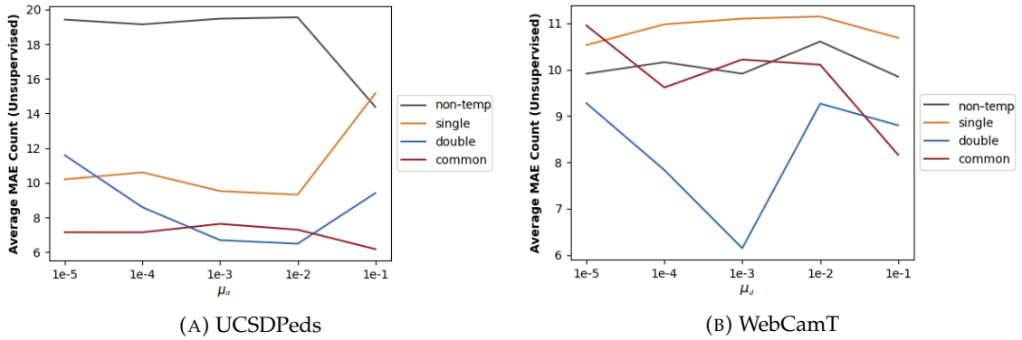
FIGURE 4.18: Average MAE count across domains for each \mu_d in the unsupervised setting in UCSDPeds and WebCamT datasets.
