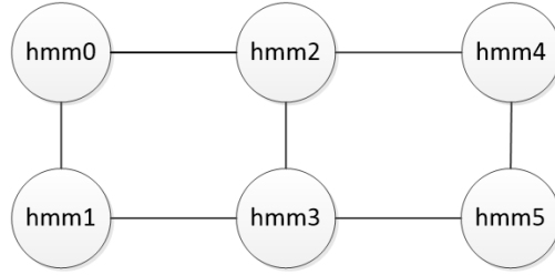
FIGURE 3.1: 2 \times 3 rectangular lattice.
