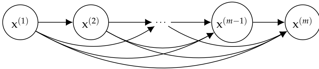
FIGURE 2.1: A complete Bayesian network.
