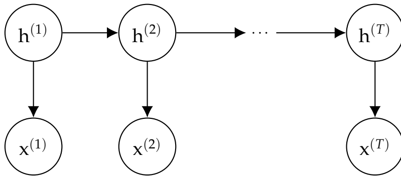
FIGURE 2.5: Hidden Markov model represented as Bayesian network.
