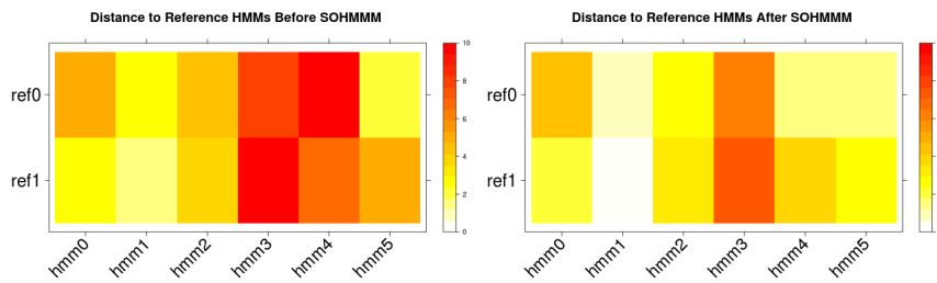
FIGURE 3.2: Monte Carlo approximation of the Kullback-Leibler divergence between the random and reference HMMs before and after applying the SOHMMM algorithm.
