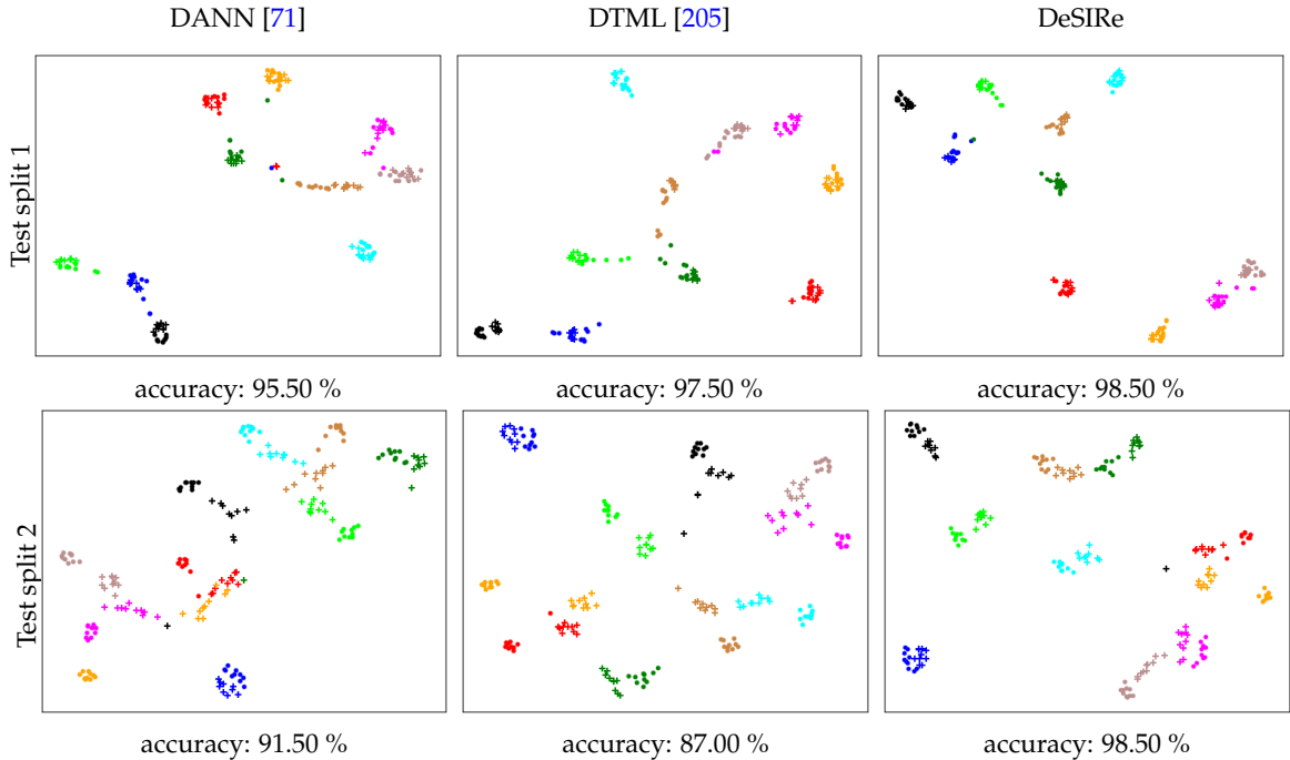
FIGURE C.3: Two-dimensional projection of the latent representation space provided by DeSIRe, DANN, and DTML, using t-SNE [185]. Markers \bullet and + represent two different test signers from the MKLM dataset and the different colors correspond to the 10 sign classes. The accuracy of each model on each split is shown below each picture.
