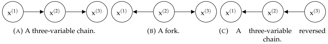
FIGURE 2.3: Equivalent three-variable Bayesian networks.
