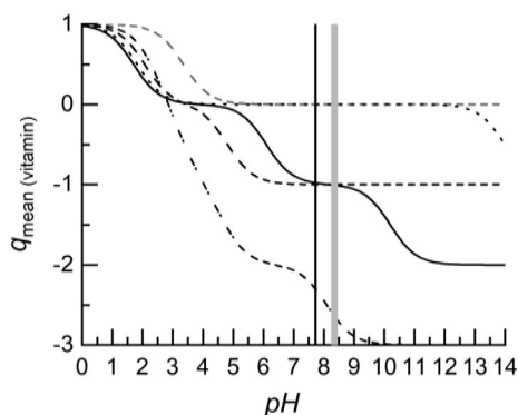
FIGURE 1 The mean charge number q_{\text{mean}} of all species in aqueous solution (calculated from the ionic distribution using pKa values from Table 1) as a function of pH. Lines: dashed—VB3 (gray—VB3 amide , black—VB3 acid ), solid—VB2, dashed-dot—VB9, dotted—VB12. Vertical lines: PEG + Na 3 Citrate (gray), PEG + Na 2 Tartrate (black). The width of the vertical presents the pH range of the two phases of the aqueous two-phase systems (ATPSs)
