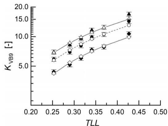
FIGURE 6 Partition coefficients of VB9 species K_{VB9} (circles), K_{VB9^{2-}} (diamonds), K_{VB9^{3-}} (triangles) in aqueous two-phase system (ATPS) PEG 6000 \text{Na}_3\text{Citrate} at different TL compositions, T = 298.15 K and p = 1 bar. Closed symbols: experimental data ( K_{vit, total}^{exp, x} ; total, contains VB9 2- and VB9 3- ) and data calculated with Equation (15) ( K_{vit, j}^{exp, x} ). Open symbols: ePC-SAFT (electrolyte Perturbed-Chain Statistical Associating Fluid Theory) predictions ( K_{vit, j}^{pred, \infty} ; species VB9 2- or VB9 3- ) and data calculated with Equation (10) ( K_{vit, total}^{pred, \infty} ). Lines are the best fit to ePC-SAFT predictions (solid lines— K_{vit, j}^{pred, \infty} and dashed lines— K_{vit, total}^{pred, \infty} ) applied only to guide the eye. Data measured in this work are presented in Table S4 (SI)
