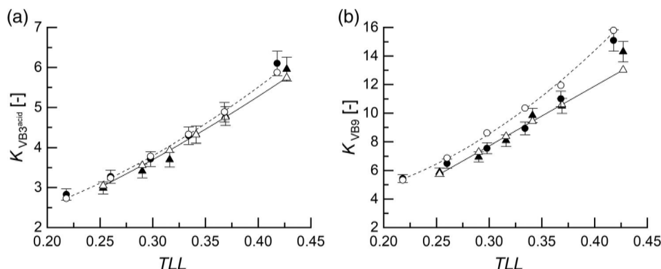
FIGURE 7 PEG molecular weight effect on partition coefficients of VB3 acid and VB9 in aqueous two-phase system (ATPS) at T = 298.15 K and p = 1 bar. ATPS formed by PEG 4000 (dashed lines and circles)—Na 3 Citrate and PEG 6000 (solid lines and triangles)—Na 3 Citrate. Lines and open symbols: ePC-SAFT (electrolyte Perturbed-Chain Statistical Associating Fluid Theory) predictions (using parameters from Tables 3 and 4), closed symbols: experimental data. Lines represent the best fit to ePC-SAFT predictions applied only to guide the eye
