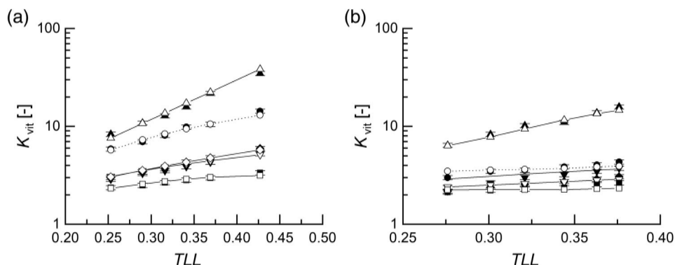
FIGURE 5 Partition coefficients at T = 298.15 K and p = 1 bar in aqueous two-phase system (ATPS): (a) PEG 6000 \text{Na}_3\text{Citrate} , (b) PEG 6000 \text{Na}_2\text{Tartrate} at different TL compositions. Experimental data K_{vit, total}^{exp, x} measured in this work: closed symbols (Table S4, SI), ePC-SAFT (electrolyte Perturbed-Chain Statistical Associating Fluid Theory) predictions: open symbols. Vitamins: VB2 (circles), VB3 acid (squares), VB3 amide (up-to-down triangles), VB9 (diamonds), VB12 (triangles). Solid lines: the best fit to ePC-SAFT predictions of K_{vit, j}^{pred, \infty} —only to guide the eye, dotted lines: K_{vit, total}^{pred, \infty} calculated using Equation (10) and ePC-SAFT predictions of K_{vit, j}^{pred, \infty} . Logarithmic scale was introduced for better data comparison
