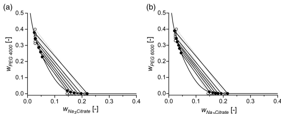
FIGURE 4 Aqueous two-phase system (ATPS) containing PEG (4,000, 6,000) and \text{Na}_3\text{Citrate} at T = 298.15 \text{ K} , p = 1 \text{ bar} : experimental 17 and ePC-SAFT (electrolyte Perturbed-Chain Statistical Associating Fluid Theory modeling). The equilibrium compositions are presented as circles: experimental (closed symbols) and ePC-SAFT modeling (open symbols). The solid lines (binodals, tie-lines) experimental, dotted lines (tie-lines) ePC-SAFT
