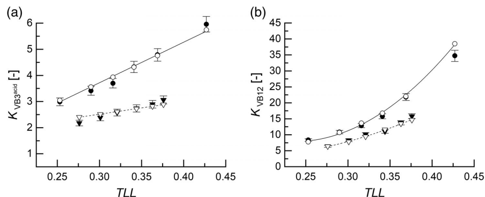
FIGURE 8 Anion effect on partition coefficients of VB3 acid and VB12 in aqueous two-phase system (ATPS) at T = 298.15 K and p = 1 bar. ATPS formed by PEG 6000 Na 3 Citrate (solid lines and circles) and PEG 6000 Na 2 Tartrate (dashed lines and triangles). Lines and open symbols: ePC-SAFT (electrolyte Perturbed-Chain Statistical Associating Fluid Theory) predictions (using parameters from Tables 3 and 4), closed symbols: experimental data. Lines represent the best fit to ePC-SAFT predictions applied only to guide the eye
