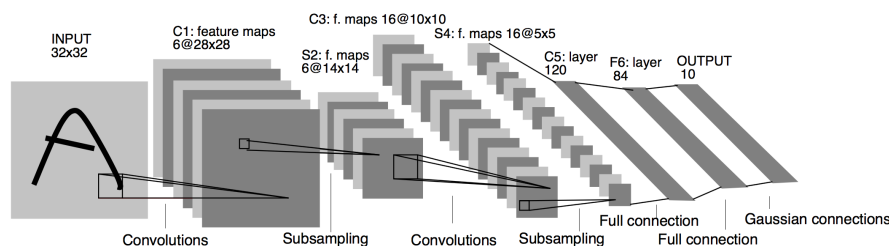
Figure 2.8: Architecture of LeNet-5. Extracted from [21].
