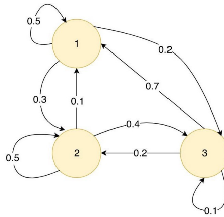
Figure 4.1: Markov process showing the probability of the transition from one state to another. The probability of reaching a state from any state is one. Extracted from [45].
