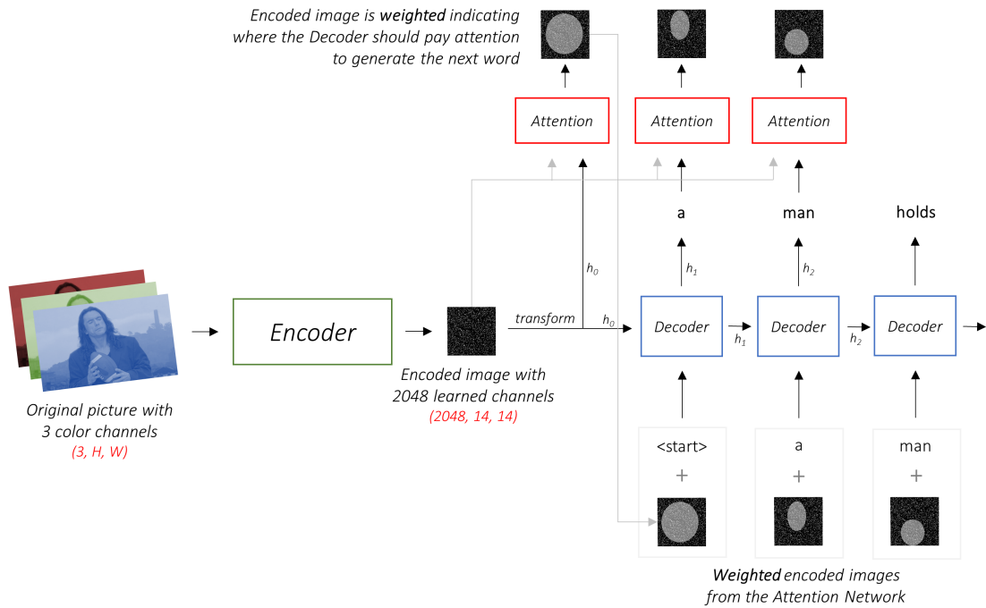
Figure 5.2: Example of an encoder-decoder architecture with an attention mechanism. The encoded image is initially fed to the decoder. In each time step, the decoder receives the weighted encoded image from the attention network. Extracted from [96].
