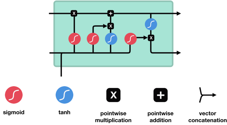
Figure 4.4: LSTM cell and its operations. Extracted from [53].
