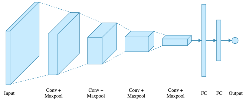
Figure 2.7: Typical CNN architecture. Extracted from [14].
