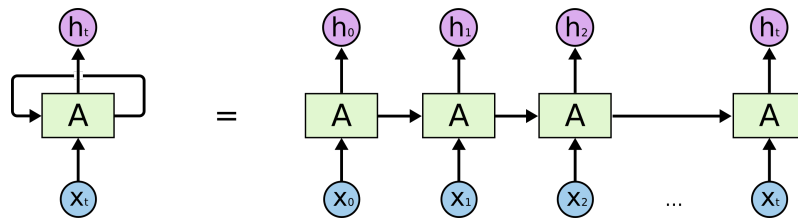
Figure 4.2: RNN model diagram. A RNN can be seen as a chain of multiple copies of the same network, each passing the information to its successor, allowing information to persist. Extracted from [48].
