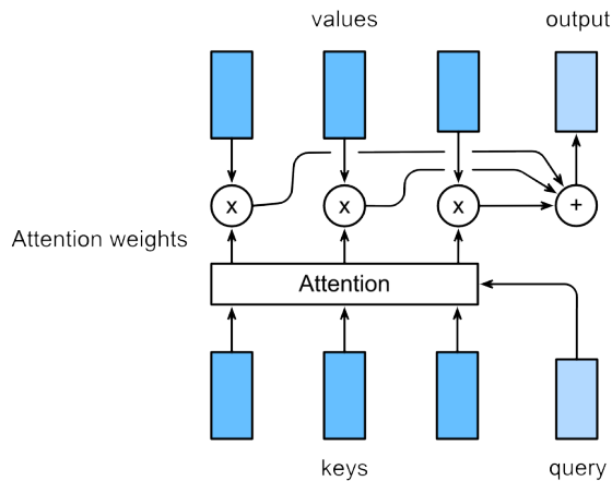
Figure 4.6: Self-attention block. The output is a weighted sum of the values, where each weight is a function of the query and the keys. Extracted from [57].
