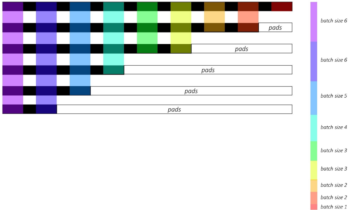
Figure 5.3: Padded sequences sorted by decreasing lengths (left) and packed sequence with the effective batch size in each time step (right). Adapted from [96].
