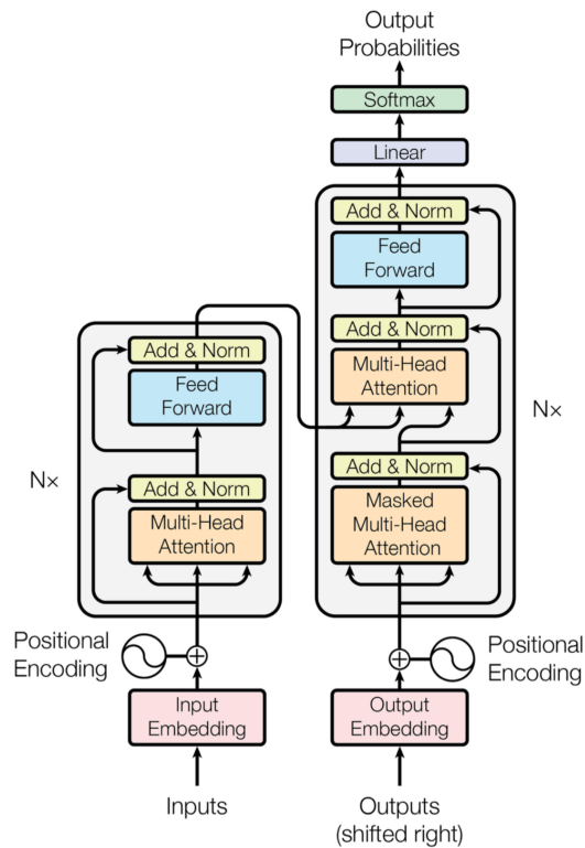
Figure 4.7: The transformer model architecture. First, the positional encoding remembers how the sequence is fed into the model since a sequence depends on the order of its elements. Both the encoder (left) and decoder (right) are composed of stacked layers, N_x . Each layer of the encoder has two sub-layers — the first is a multi-head attention mechanism and the second is a position-wise fully connected feedforward network. There is a residual connection around each sub-layer to avoid the vanishing gradient problem. The decoder is rather similar to the encoder. However, each decoder layer adds a third sub-layer that performs multi-head attention over the output of the encoder layer. Lastly, a linear transformation and a softmax function are used to convert the decoder output to the predicted word probability. Extracted from [56].
