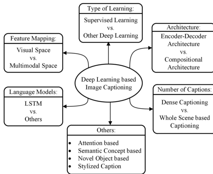
Figure 4.8: Overall taxonomy of DL-based image captioning. Extracted from [59].
