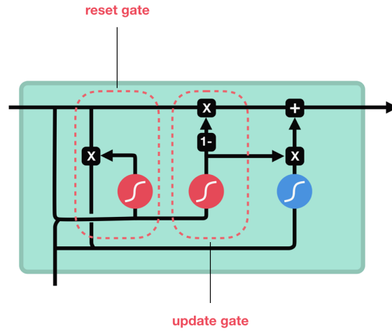
Figure 4.5: GRU cell. Extracted from [53].
