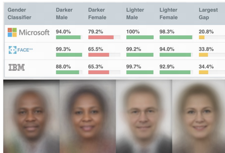
Figure 3.2: Gender classification performance as measured by the positive predictive value (PPV) of the three evaluated commercial gender classifiers on the PPB dataset. Extracted from [31].
