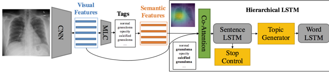
Figure 4.11: Illustration of the model proposed by Jing et al. The visual features are extracted from the last convolutional layer of the CNN (VGG-19 [24]) while the last two fully connected layers are used for the MLC task. Each tag is represented by a word-embedding vector that is used as a semantic feature vector. Both visual and semantic features are concatenated and fed into a co-attention model to obtain a joint context vector. The context vector is the input to a sentence LSTM, which produces a topic vector. Given a topic vector, the word LSTM generates the final sentence. Extracted from [88].
