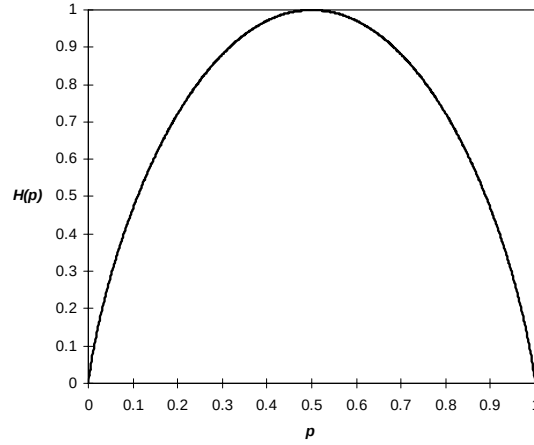
Figure 3.1: Entropy H(p) = H(p, 1 - p) of a binary random variable having two outcomes with probabilities p_1 = p , p_2 = 1 - p , 0 \leq p \leq 1 , as a function of p .
