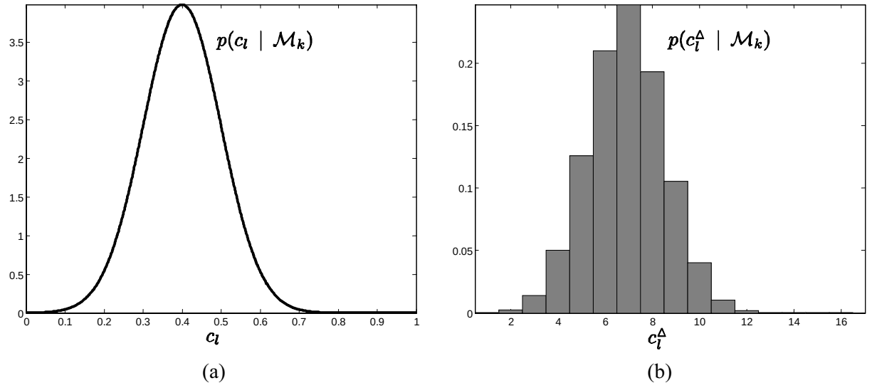
Figure 4.3: Quantization of the voxel's coverage probability density function (pdf): (a) example of a Gaussian for the voxel's pdf p(c_l | \mathcal{M}_k) ; (b) quantized version p(c_l^\Delta | \mathcal{M}_k) of the voxel's pdf p(c_l | \mathcal{M}_k) , using a 16 bins histogram. In this example, the voxel's discrete entropy is H(C_l) = 2.749 bits.
