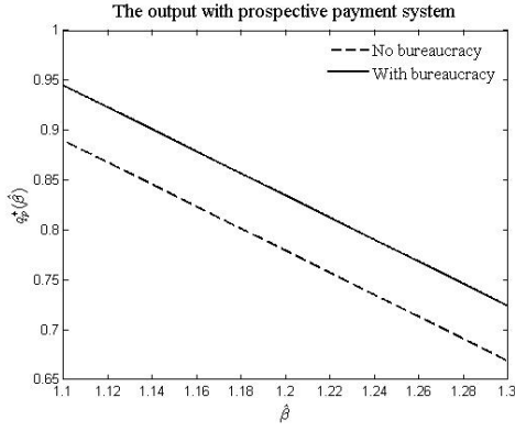
Figure 7: Output with ( \delta = 0.05 ) and without bureaucracy ( \delta = 0 ).
