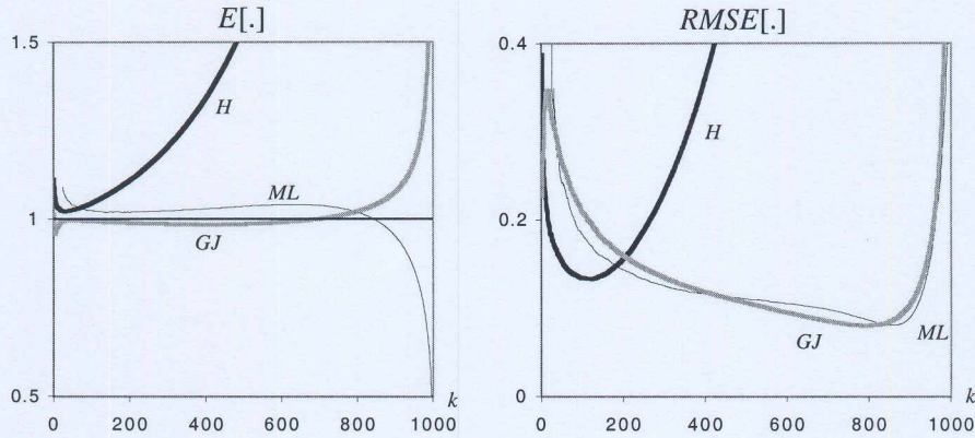
Figure 3: Burr parent with (\gamma, \rho) = (0.25, -1)
