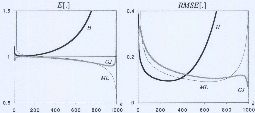
Figure 5: Burr parent with (\gamma, \rho) = (0.25, -2)
