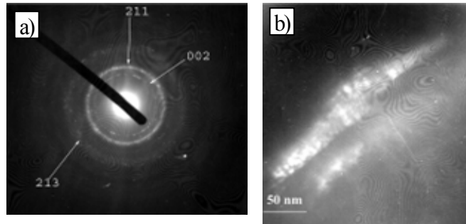
Figure 8. Transmission electron microscopy results of the as prepared BL-HA2: (a) Powder diffraction cliché; (b) Particle size and morphology.
