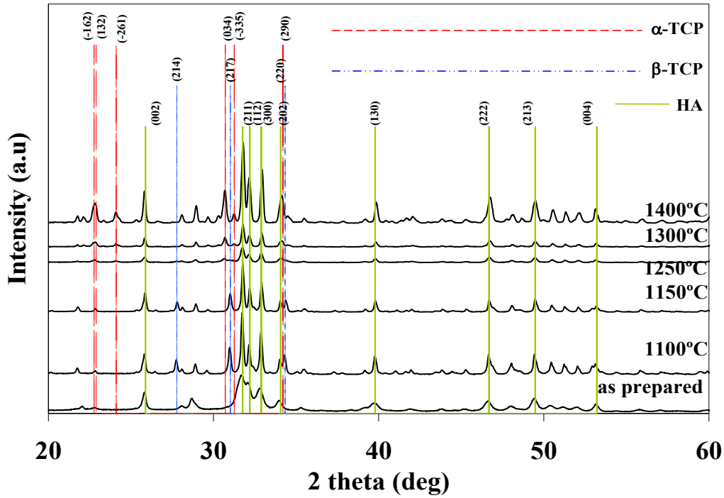
Figure 10. Crystalline phase evolution of Ca-def-HA powders with heat treatment temperatures.
