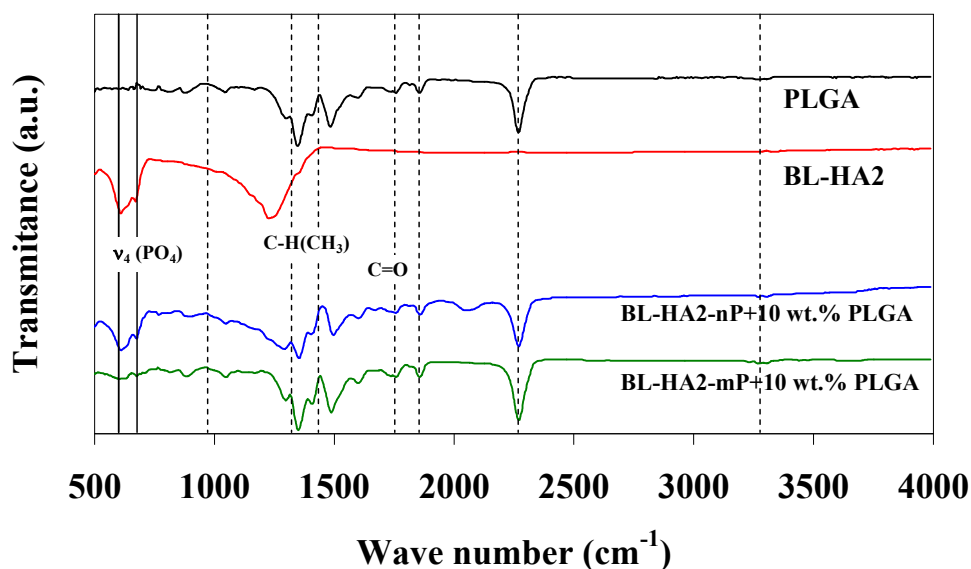
Figure 8. FTIR-ATR spectroscopic results of BL-HA2 surface treatment.
