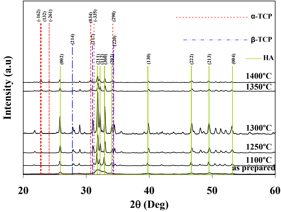
Figure 5. Crystalline phase evolution of Mg-(Ca-def-HA) powders with heat treatment temperatures.
