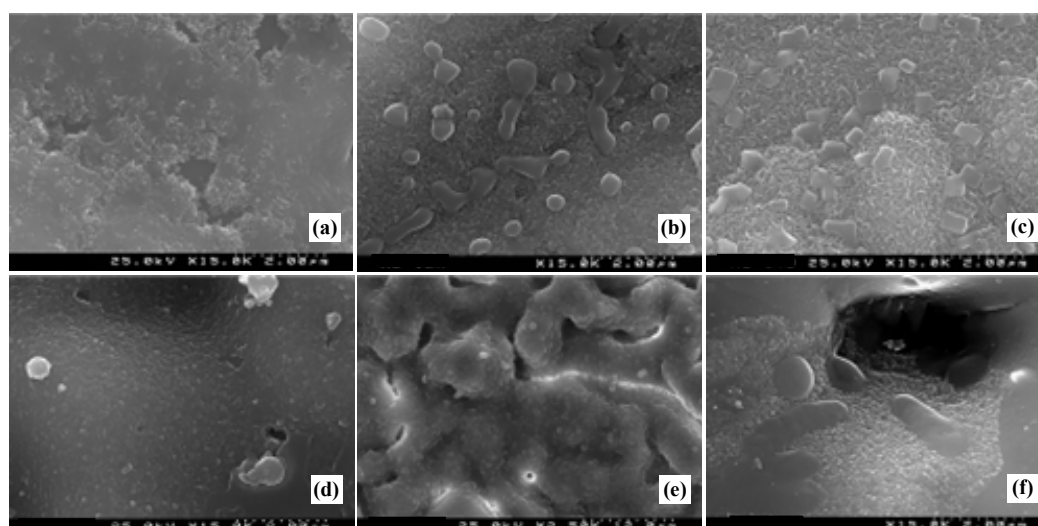
Figure 2. Microstructure of the different samples after sintering at 1250°C: (a) Mg-(Ca-def-HA); (b) BL-HA2; (c) magnification of a pore surface of Mg-(Ca-def-HA); (d) magnification of a pore surface of BL-HA2.
