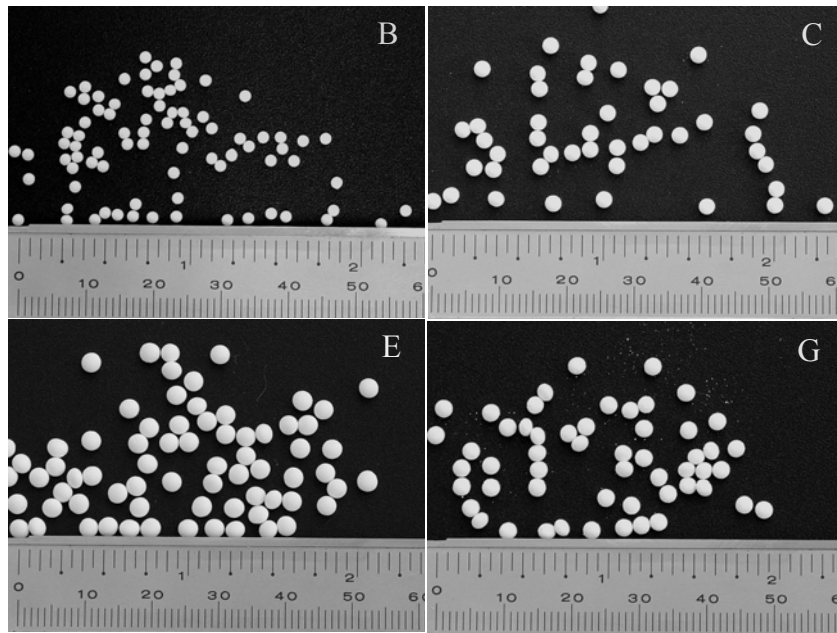
Figure 20. Digital pictures of some of the samples listed in Table 6 (B, C, E and G), showing the influence of the experimental parameters on the granule size and shape.
