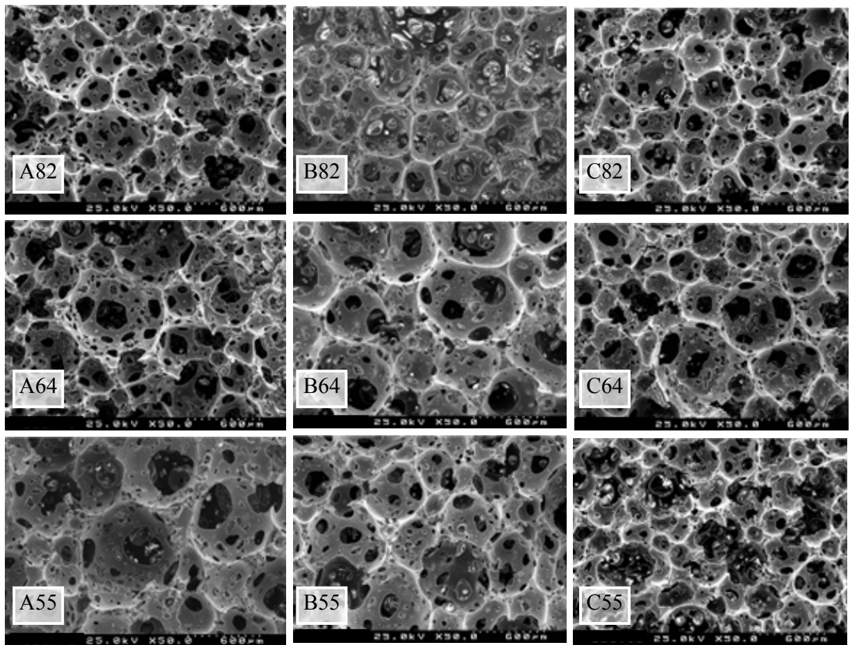
Figure 16. Microstructure of the samples A, B and C with different FBC/SLS proportions, sintered at 1250°C.
