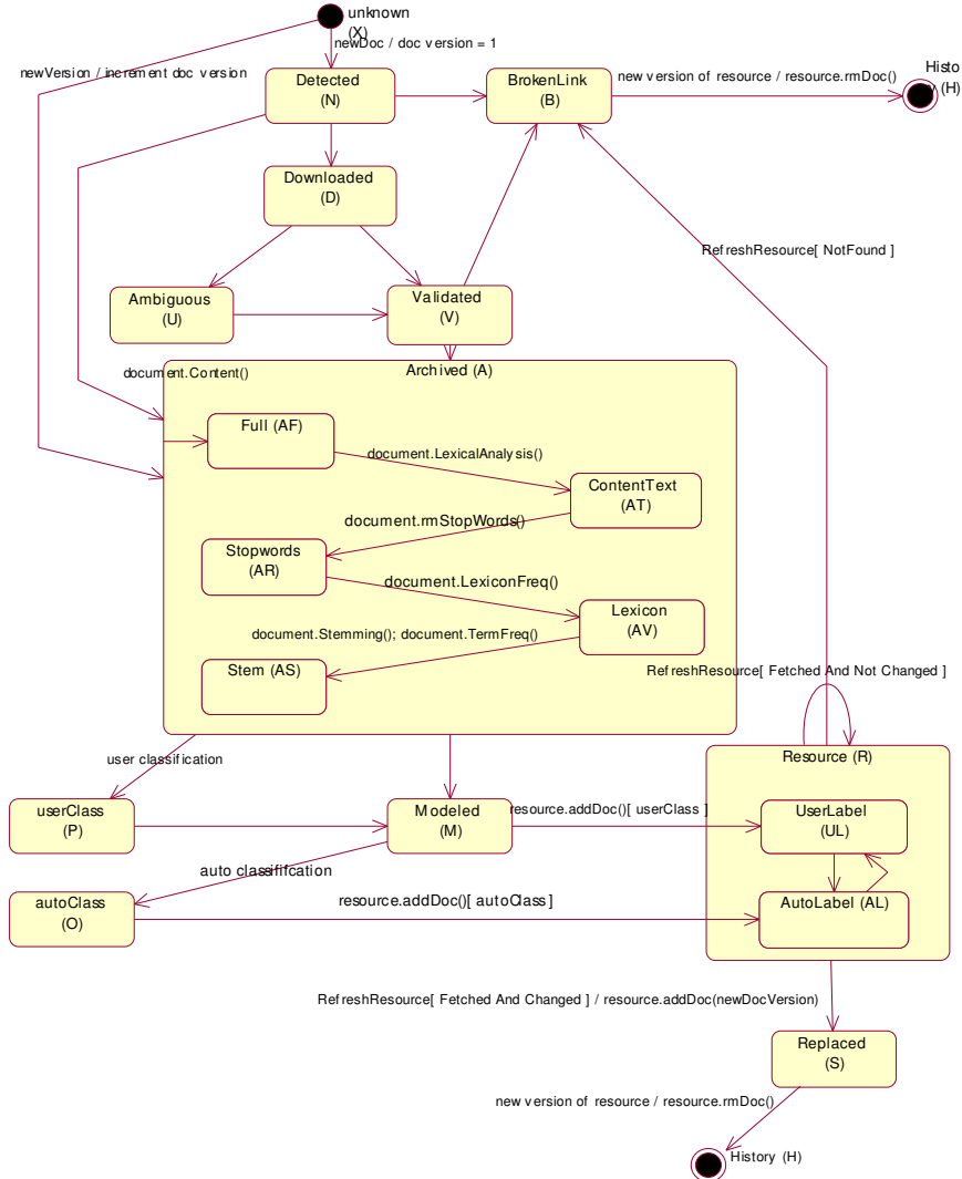
Figure 4.17 – Document entity lifecycle
