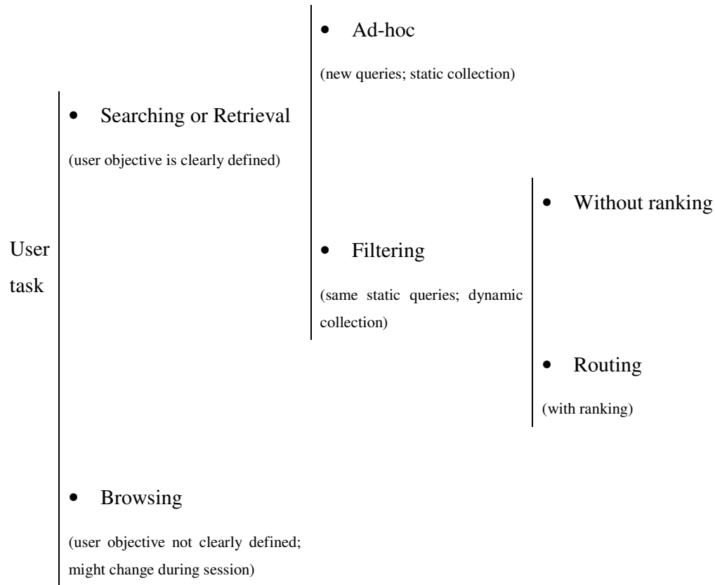
Figure 2.2 – User task
