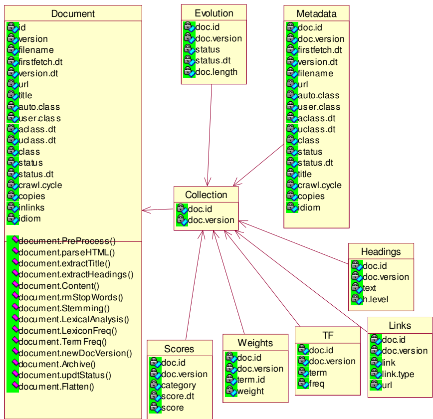
Figure 4.16 – Document entity, attributes and methods
