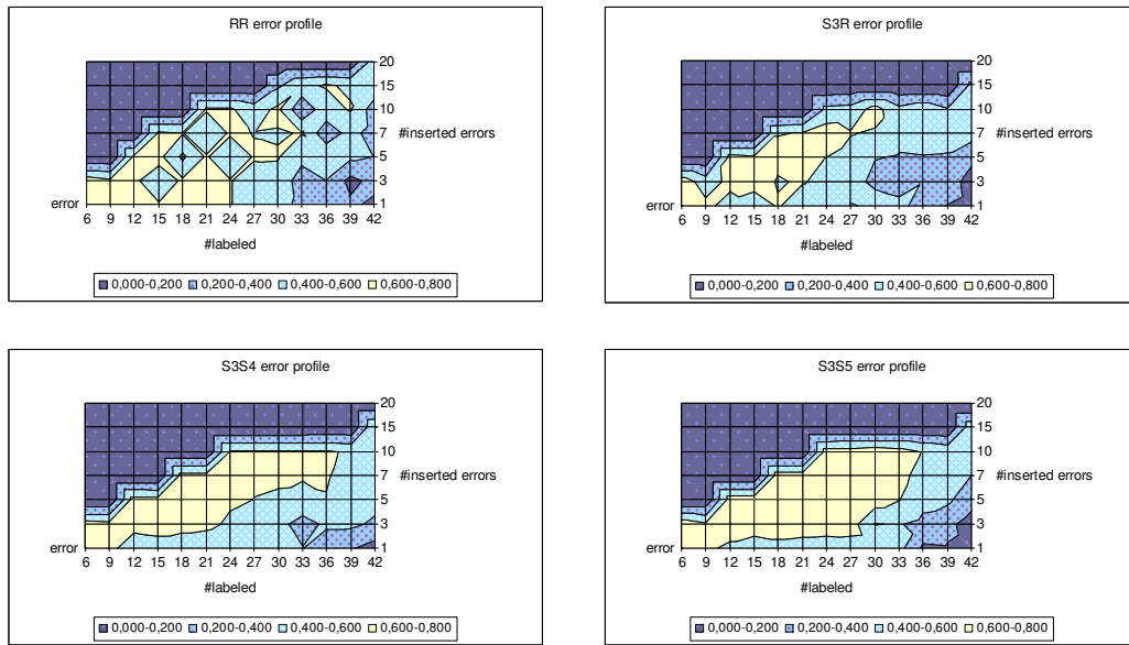
Figure 5.22 – Semi-supervised robustness for PE
