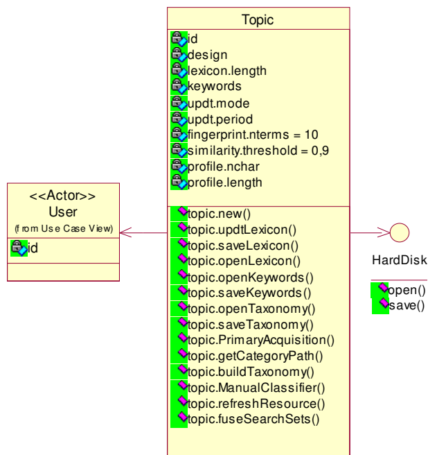
Figure 4.11 – Topic entity, attributes and methods
