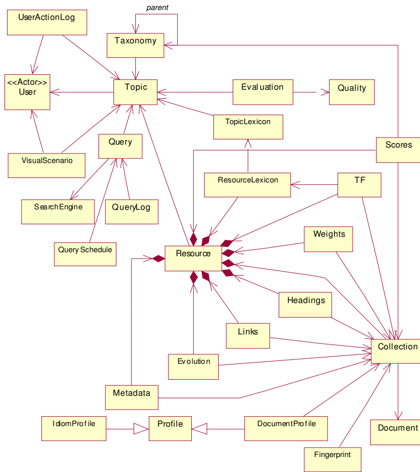
Figure 4.9 – webTOPIC entities
