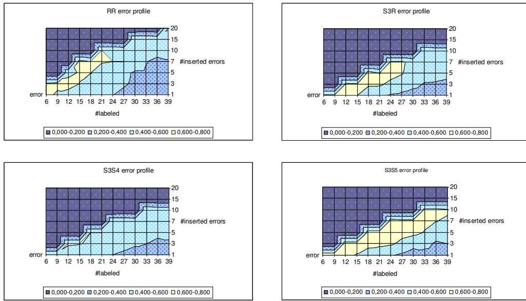
Figure 5.21 – Semi-supervised robustness for AI
