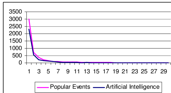
Figure 5.9 – IDF distribution
