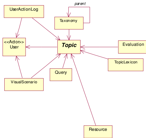
Figure 4.10 – Topic entity relationships
