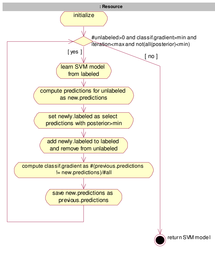
Figure 4.5 – Bootstrapping SVM
