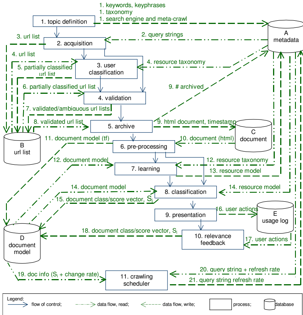
Figure 4.8 – webTOPIC architecture, internal view
