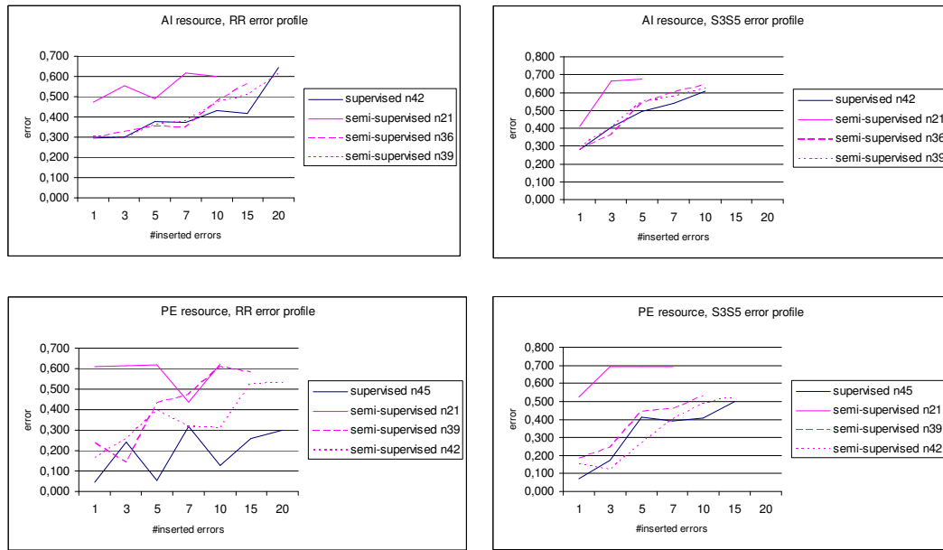
Figure 5.24 – Error rate by inserted errors percentage
