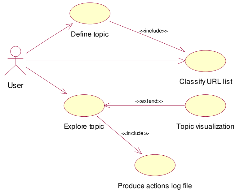
Figure 4.1 – webTOPIC from user's point of view
