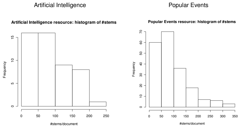
Figure 5.2 – Stems per document histograms
