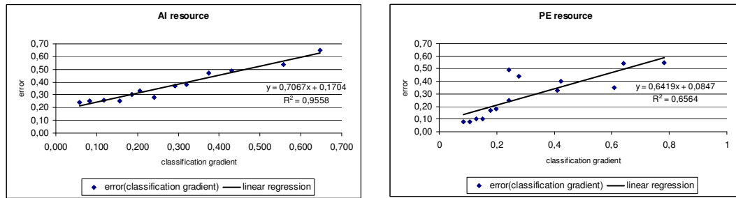
Figure 5.16 – Correlation between error and classification gradient
