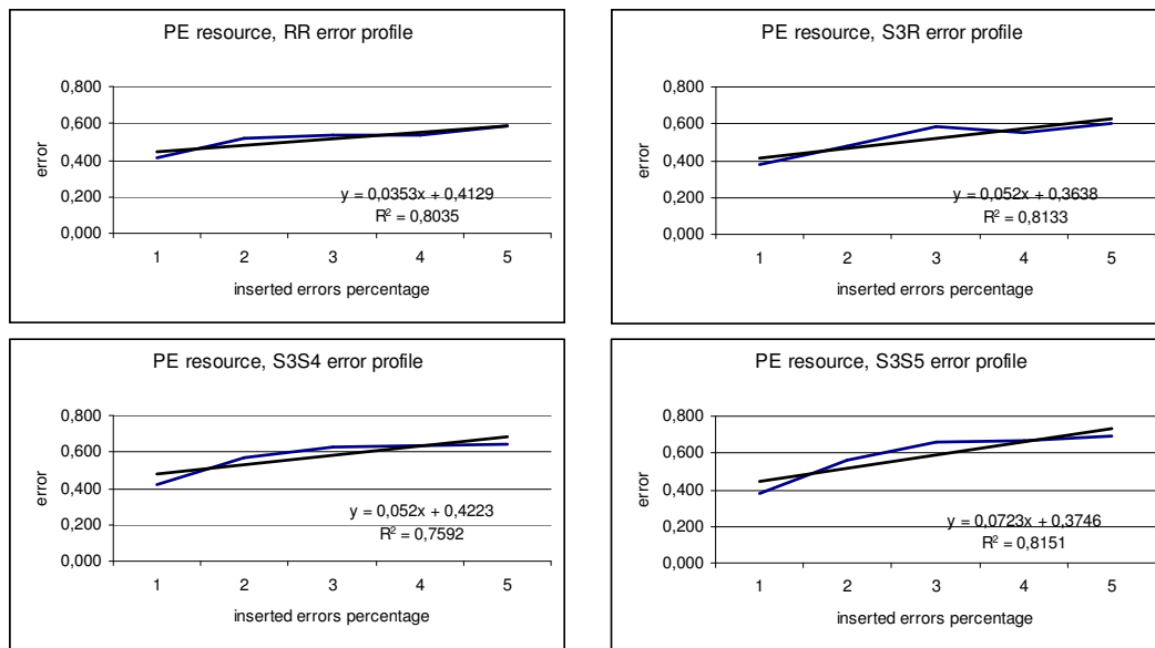
Figure 5.23 – Semi-supervised error rate by inserted errors percentage
