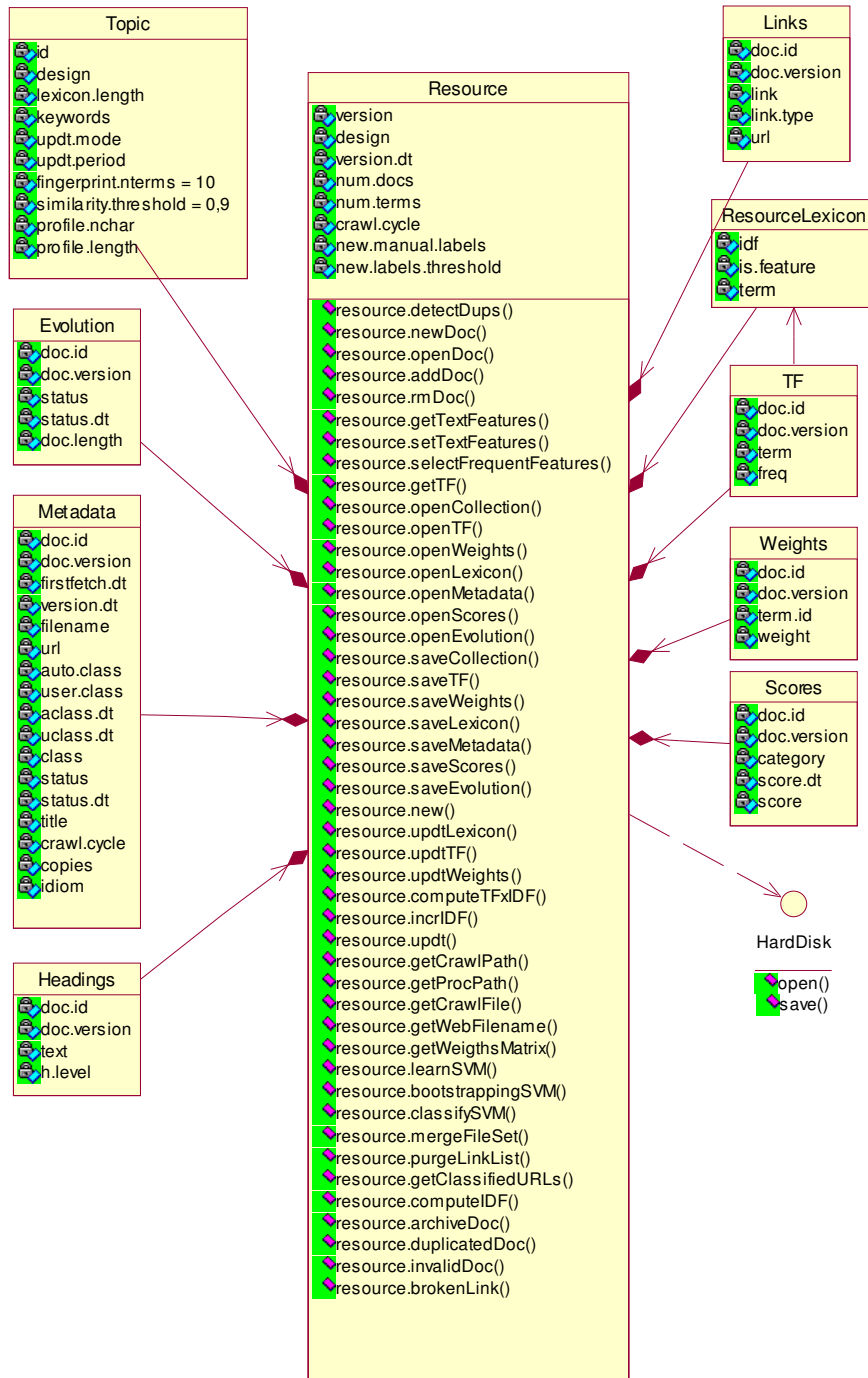
Figure 4.13 – Resource entity, attributes and methods
