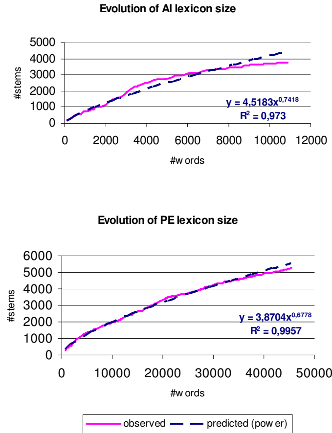
Figure 5.5 – Lexicon size evolution with respect to the number of words in the resource
