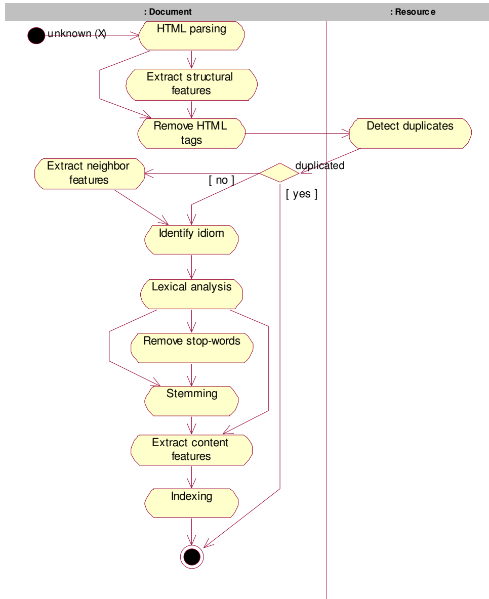
Figure 4.4 – Document pre-processing, data preparation step
