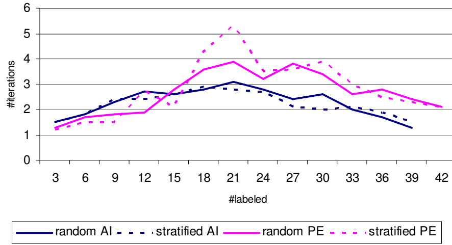
Figure 5.13 – Evolution of required number of iterations
