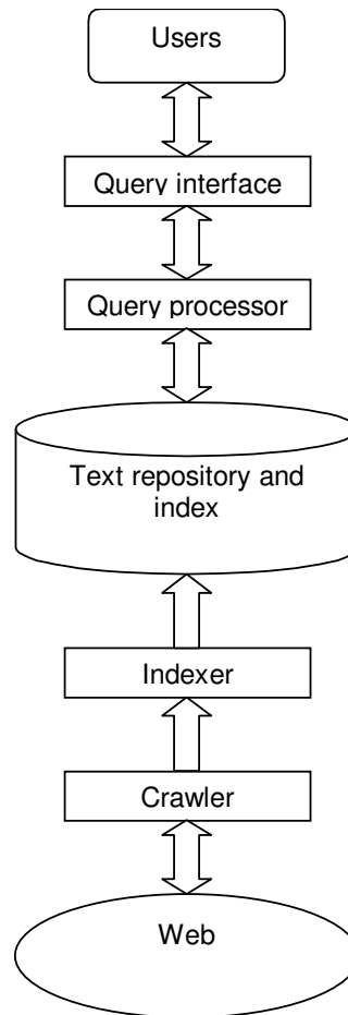
Figure 2.3 – Search engine architecture
