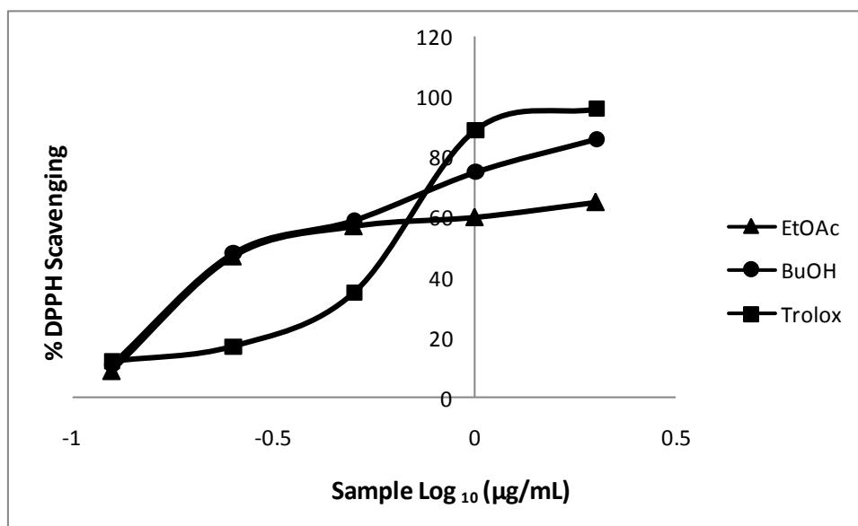
Figure 1: Concentration-response curves for the DPPH radical scavenging activity of trolox (positive control), butanol fraction and ethyl acetate fraction of R. excelsa .
