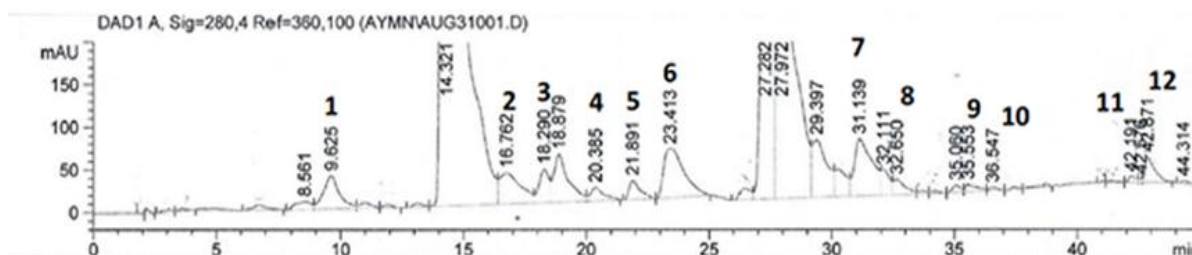
Figure 2: HPLC–DAD chromatograms at 280 nm of the EtOH extracts of Rhapsis leaves; Peak numbers refer to Table 1.
